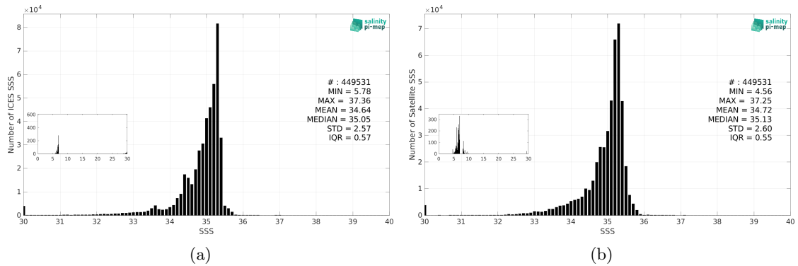
Figure 3: Histograms of SSS from ICES (a) and CCI SSS L4 Merged-OI v5.5 - 7-day running (ESA) (b) considering all match-up pairs per bins of 0.1 over the SMOS coastal zone (<800km) 60N-60S Pi-MEP region and for the full satellite product period.
