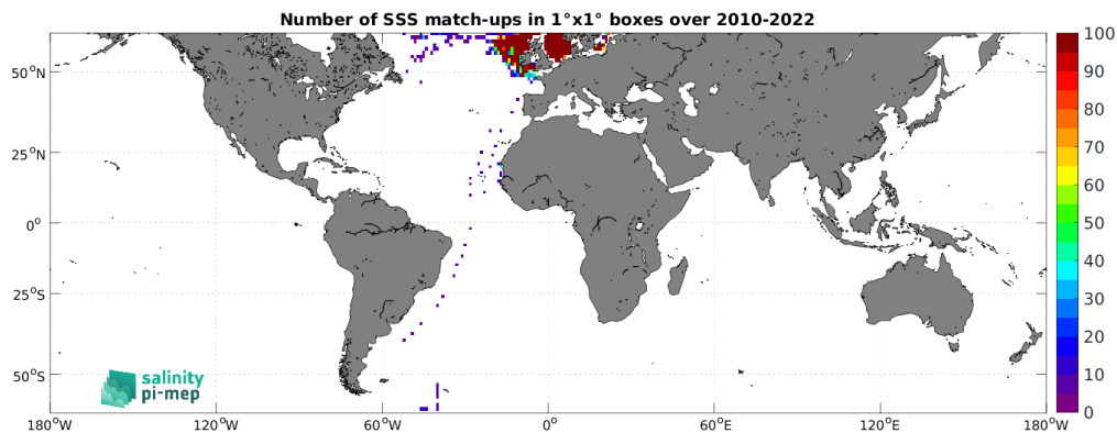
Figure 5: Number of SSS match-ups between ICES SSS and the CCI SSS L4 Merged-OI v5.5 - 7-day running (ESA) SSS product for the SMOS coastal zone (<800km) 60N-60S Pi-MEP region over 1^\circ \times 1^\circ boxes and for the full satellite product period.
