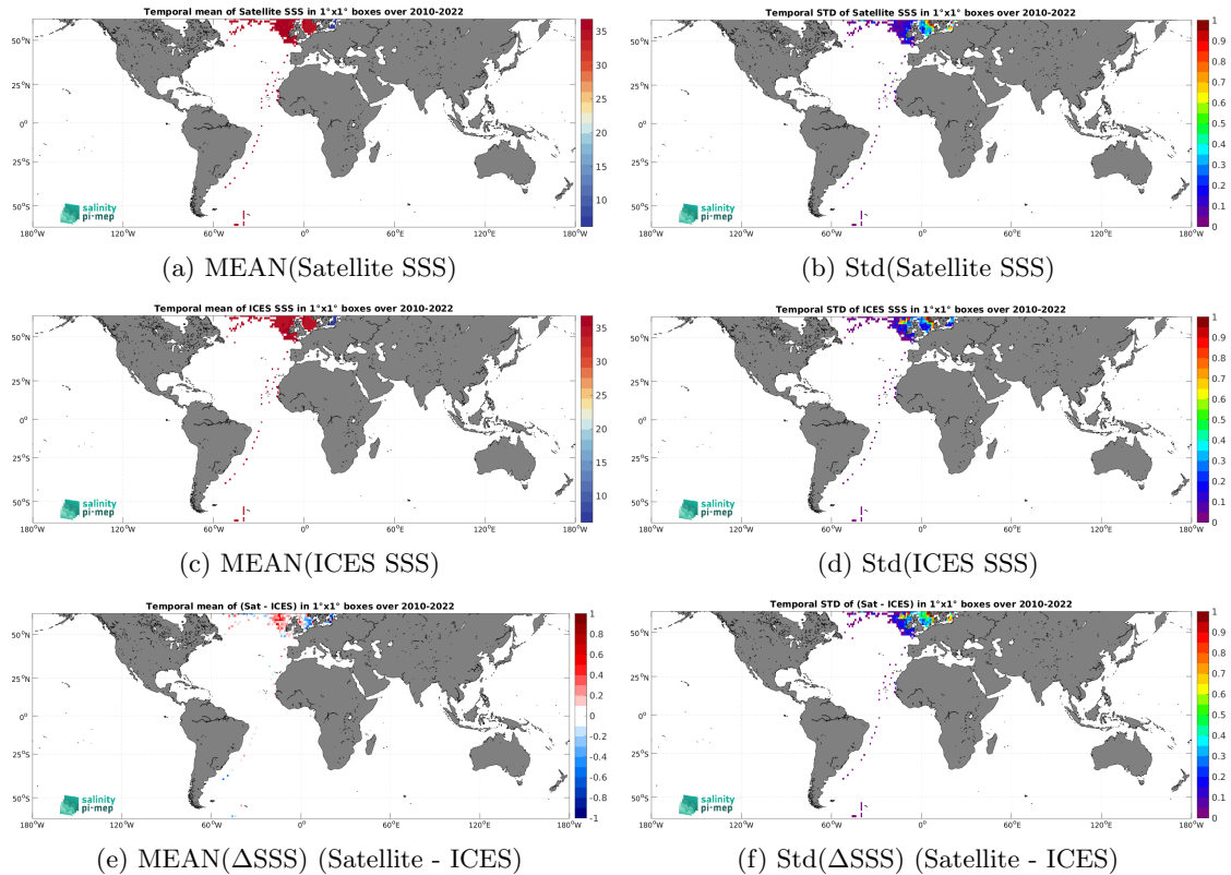
Figure 7: Temporal mean (left) and Std (right) of SSS from CCI SSS L4 Merged-OI v5.5 - 7-day running (ESA) (top), ICES (middle), and of \Delta SSS (Satellite - ICES). Only match-up pairs are used to generate these maps.
