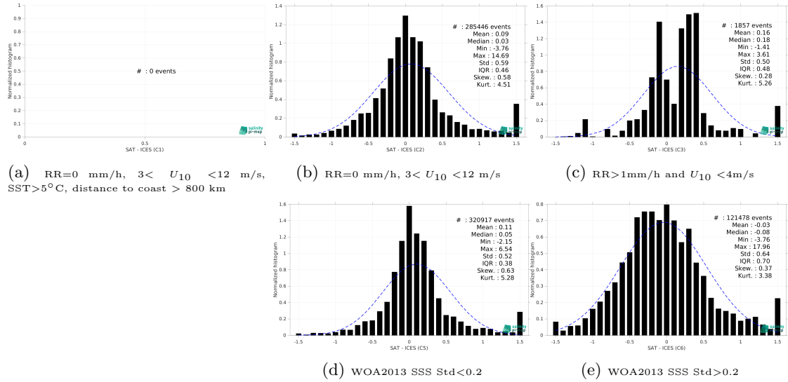
Figure 15: Normalized histogram of \Delta SSS (CCI SSS L4 Merged-OI v5.5 - 7-day running (ESA) - ICES) for 5 different subdatasets corresponding to: RR=0 mm/h, 3 < U_{10} < 12 m/s, SST > 5°C, distance to coast > 800 km (a), RR=0 mm/h, 3 < U_{10} < 12 m/s (b), RR > 1mm/h and U_{10} < 4 m/s (c), WOA2013 SSS Std < 0.2 (d), WOA2013 SSS Std > 0.2 (e).
