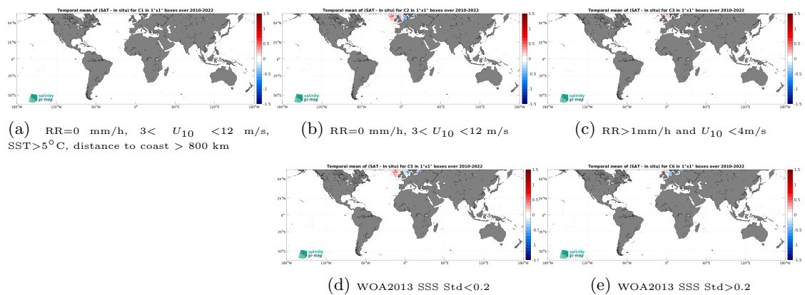
Figure 14: Temporal mean gridded over spatial boxes of size 1^\circ \times 1^\circ of \Delta SSS (CCI SSS L4 Merged-OI v5.5 - 7-day running (ESA) - ICES) for 5 different subdatasets corresponding to:RR=0 mm/h, 3 < U_{10} < 12 m/s, SST >5^\circ\text{C} , distance to coast > 800 km (a), RR=0 mm/h, 3 < U_{10} < 12 m/s (b), RR >1 mm/h and U_{10} < 4 m/s (c), WOA2013 SSS Std <0.2 (d), WOA2013 SSS Std >0.2 (e).
