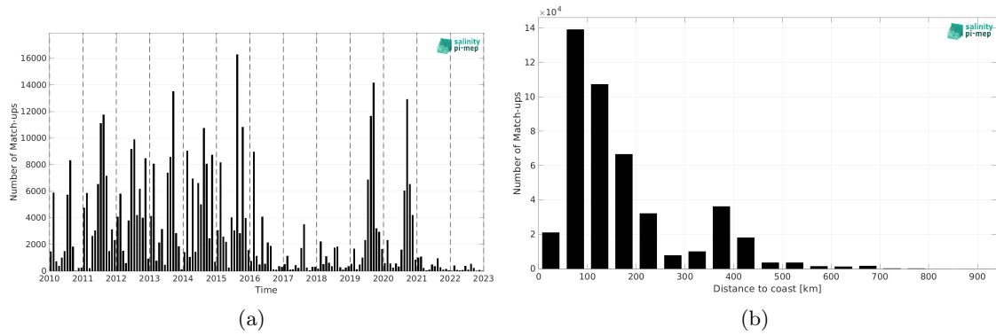
Figure 2: Number of match-ups between ICES and CCI SSS L4 Merged-OI v5.5 - 7-day running (ESA) SSS as a function of time (a) and as function of the distance to coast (b) over the SMOS coastal zone (<800km) 60N-60S Pi-MEP region and for the full satellite product period.
