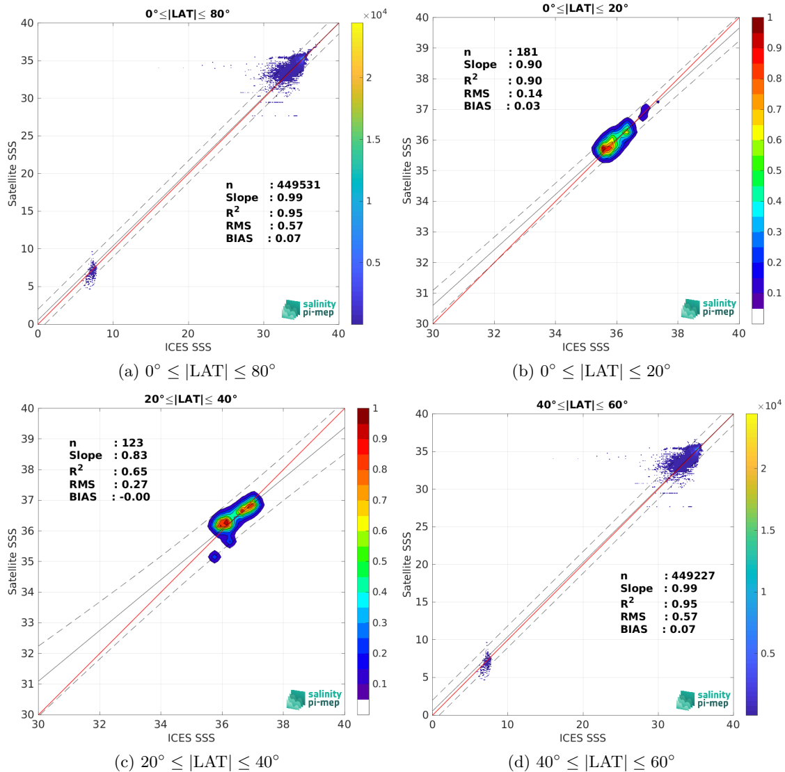
Figure 10: Contour maps of the concentration of CCI SSS L4 Merged-OI v5.5 - 7-day running (ESA) SSS (y-axis) versus ICES SSS (x-axis) at match-up pairs for different latitude bands. For each plot, the red line shows x=y . The black thin and dashed lines indicate a linear fit through the data cloud and the \pm 95\% confidence levels, respectively. The number match-up pairs n , the slope and R^2 coefficient of the linear fit, the root mean square (RMS) and the mean bias between satellite and in situ data are indicated for each latitude band in each plots.
