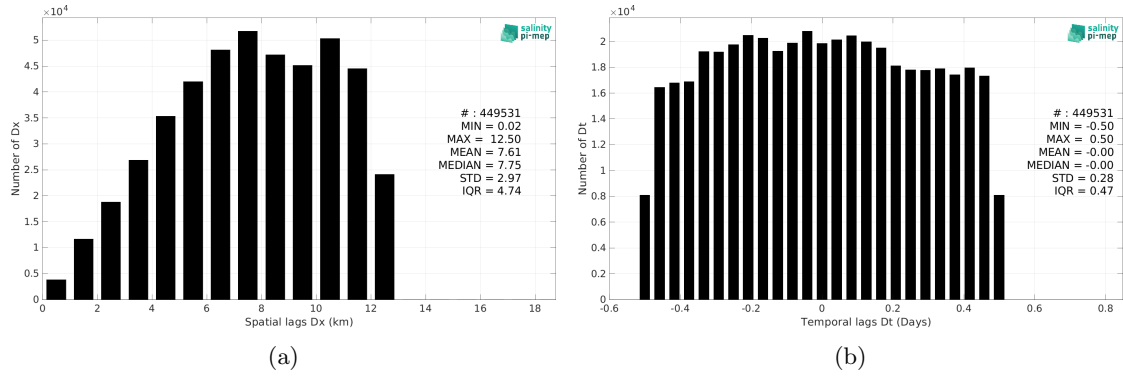
Figure 6: Histograms of the spatial (a) and temporal (b) lags between the location/time of the ICES measurement and the date of the corresponding CCI SSS L4 Merged-OI v5.5 - 7-day running (ESA) SSS pixel.
