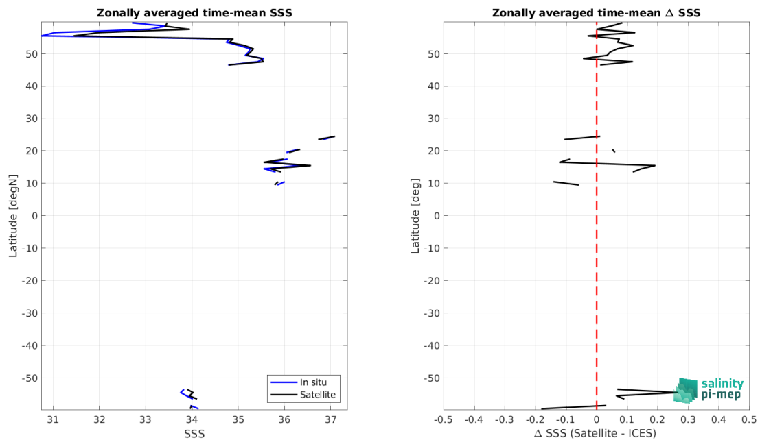
Figure 9: Left panel: Zonal mean SSS from CCI SSS L4 Merged-OI v5.5 - 7-day running (ESA) satellite product (black) and from ICES (blue). Right panel: Zonal mean of \Delta SSS (Satellite - ICES) for all the collected Pi-MEP match-up pairs estimated over the full satellite product period.
