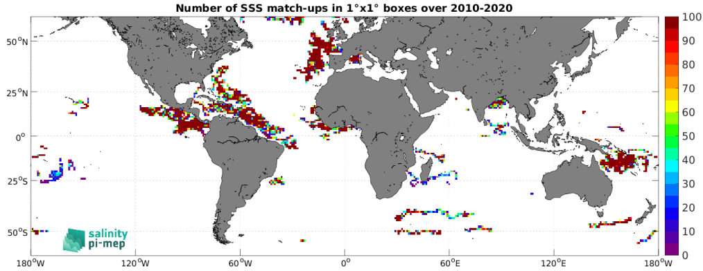
Figure 4: Number of SSS match-ups between Surface drifters SSS and the CCI SSS L4 Merged-OI v5.5 - 7-day running (ESA) SSS product for the SMOS coastal zone (<800km) 60N-60S Pi-MEP region over 1^{\circ} \times 1^{\circ} boxes and for the full satellite product period.
