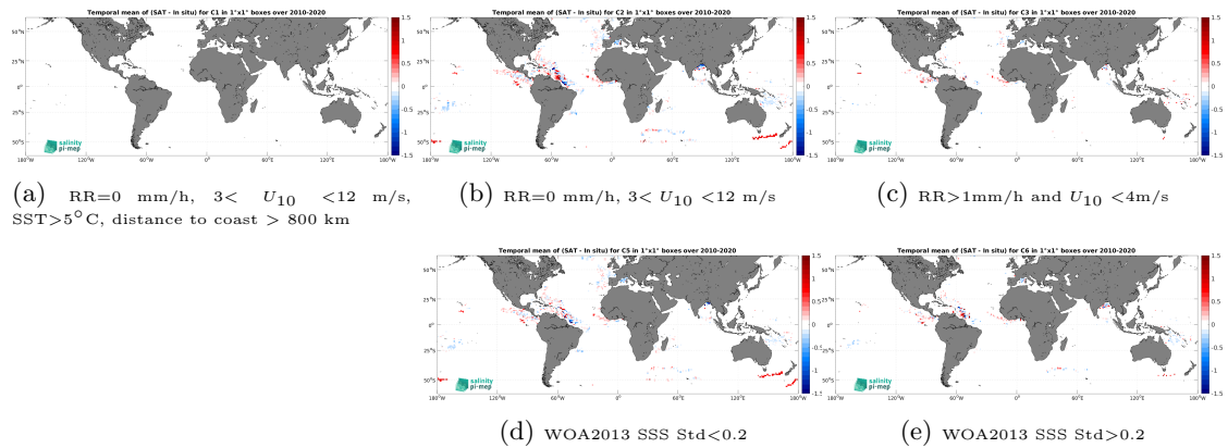
Figure 13: Temporal mean gridded over spatial boxes of size 1^\circ \times 1^\circ of \Delta SSS (CCI SSS L4 Merged-OI v5.5 - 7-day running (ESA) - Surface drifters) for 5 different subdatasets corresponding to:RR=0 mm/h, 3 < U_{10} < 12 m/s, SST >5^\circ C, distance to coast > 800 km (a), RR=0 mm/h, 3 < U_{10} < 12 m/s (b), RR >1 mm/h and U_{10} < 4 m/s (c), WOA2013 SSS Std <0.2 (d), WOA2013 SSS Std >0.2 (e).
