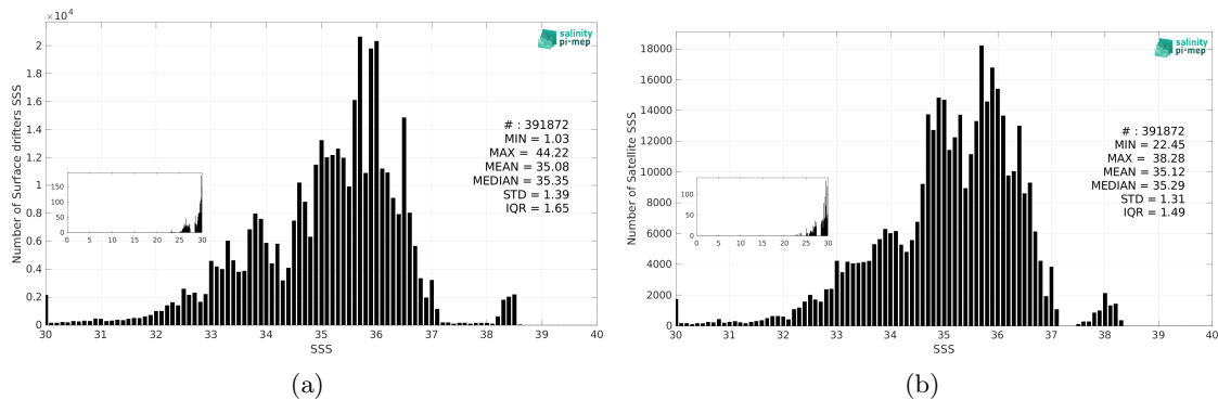
Figure 3: Histograms of SSS from Surface drifters (a) and CCI SSS L4 Merged-OI v5.5 - 7-day running (ESA) (b) considering all match-up pairs per bins of 0.1 over the SMOS coastal zone (<800km) 60N-60S Pi-MEP region and for the full satellite product period.
