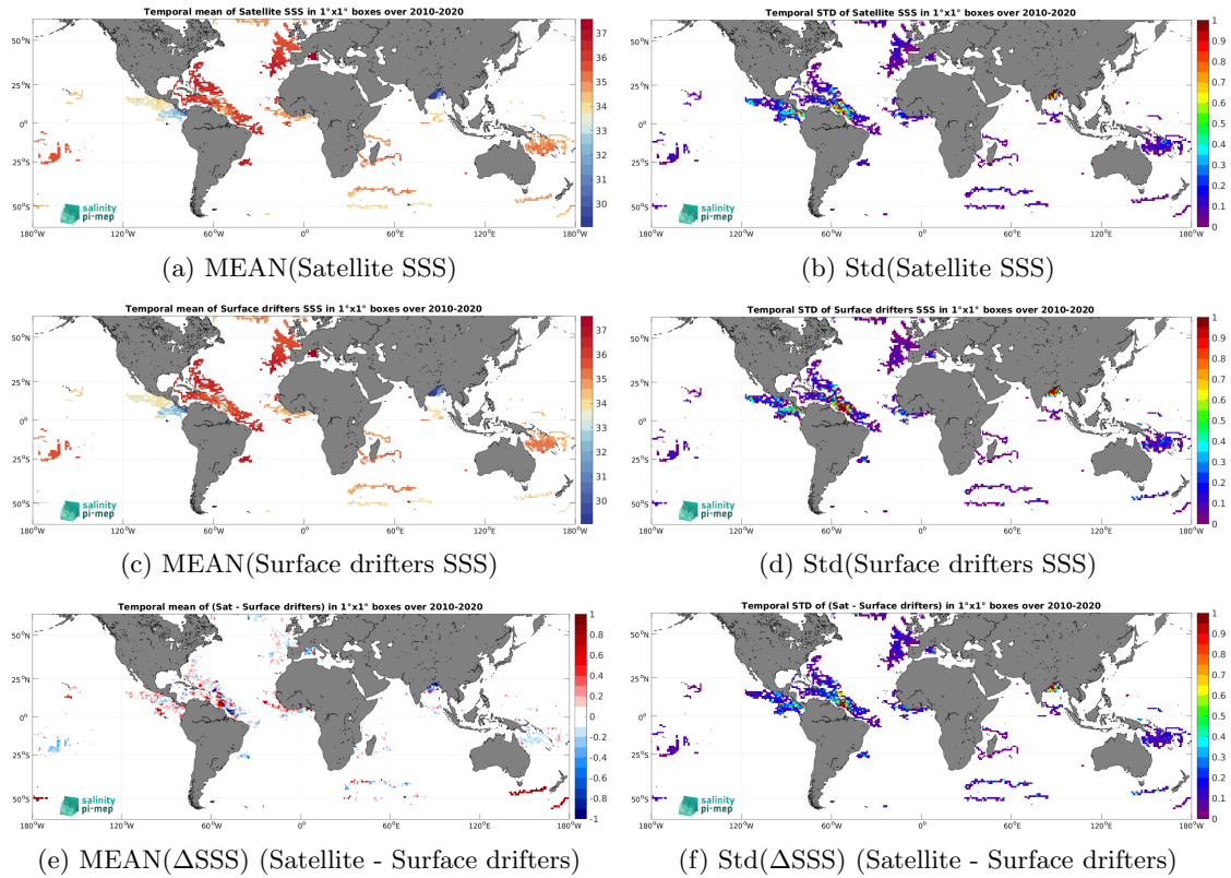
Figure 6: Temporal mean (left) and Std (right) of SSS from CCI SSS L4 Merged-OI v5.5 - 7-day running (ESA) (top), Surface drifters (middle), and of \Delta SSS (Satellite - Surface drifters). Only match-up pairs are used to generate these maps.
