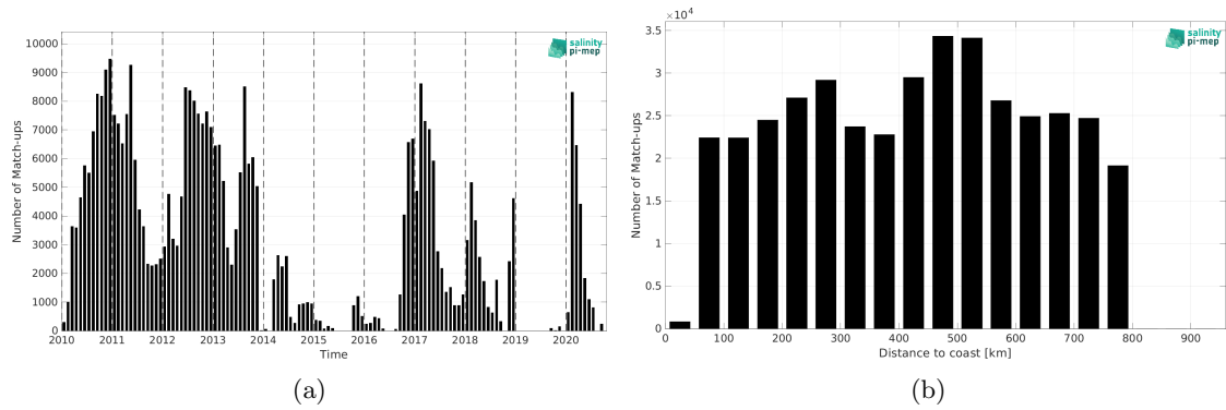
Figure 2: Number of match-ups between Surface drifters and CCI SSS L4 Merged-OI v5.5 - 7-day running (ESA) SSS as a function of time (a) and as function of the distance to coast (b) over the SMOS coastal zone (<800km) 60N-60S Pi-MEP region and for the full satellite product period.
