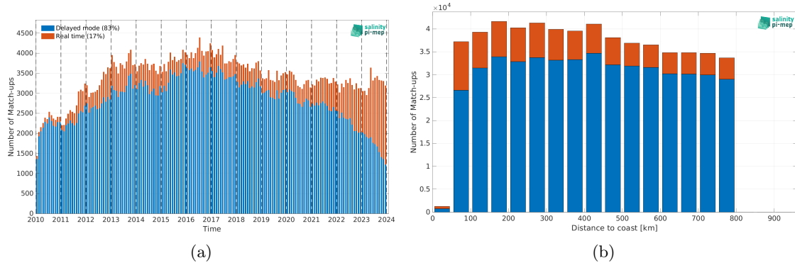
Figure 2: Number of match-ups between Argo and CCI SSS L4 Merged-OI v5.5 - 7-day running (ESA) SSS as a function of time (a) and as function of the distance to coast (b) over the SMOS coastal zone (<800km) 60N-60S Pi-MEP region and for the full satellite product period.
