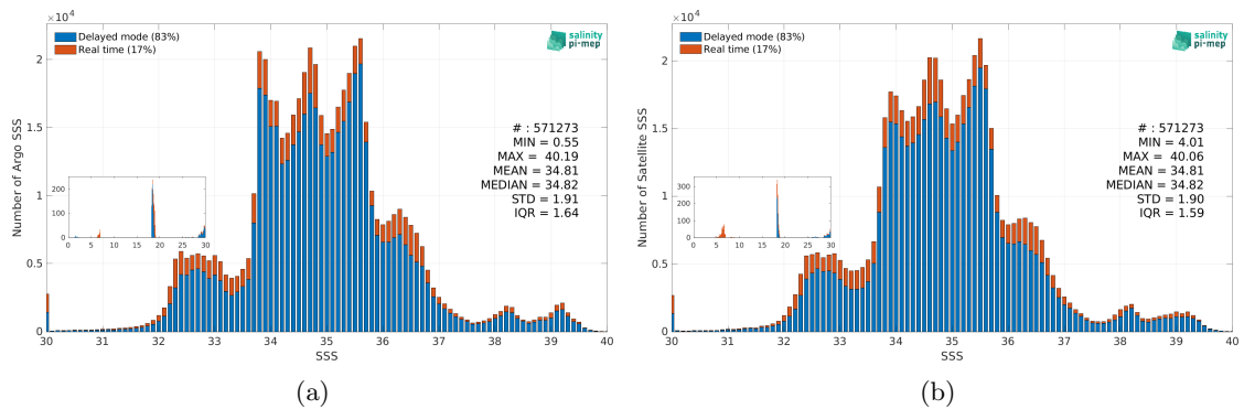
Figure 3: Histograms of SSS from Argo (a) and CCI SSS L4 Merged-OI v5.5 - 7-day running (ESA) (b) considering all match-up pairs per bins of 0.1 over the SMOS coastal zone (<800km) 60N-60S Pi-MEP region and for the full satellite product period.
