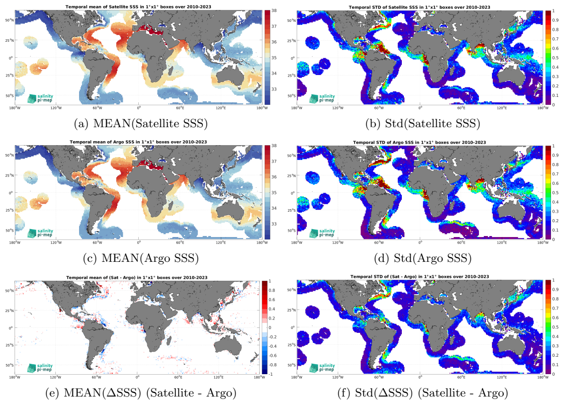
Figure 7: Temporal mean (left) and Std (right) of SSS from CCI SSS L4 Merged-OI v5.5 - 7-day running (ESA) (top), Argo (middle), and of \Delta SSS (Satellite - Argo). Only match-up pairs are used to generate these maps.
