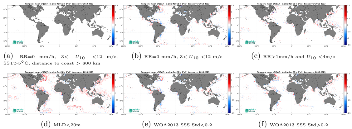
Figure 14: Temporal mean gridded over spatial boxes of size 1^\circ \times 1^\circ of \Delta SSS (CCI SSS L4 Merged-OI v5.5 - 7-day running (ESA) - Argo) for 6 different subdatasets corresponding to:RR=0 mm/h, 3 < U_{10} < 12 m/s, SST >5^\circ C, distance to coast > 800 km (a), RR=0 mm/h, 3 < U_{10} < 12 m/s (b), RR >1 mm/h and U_{10} < 4 m/s (c),MLD <20 m (d),WOA2013 SSS Std <0.2 (e),WOA2013 SSS Std >0.2 (f).
