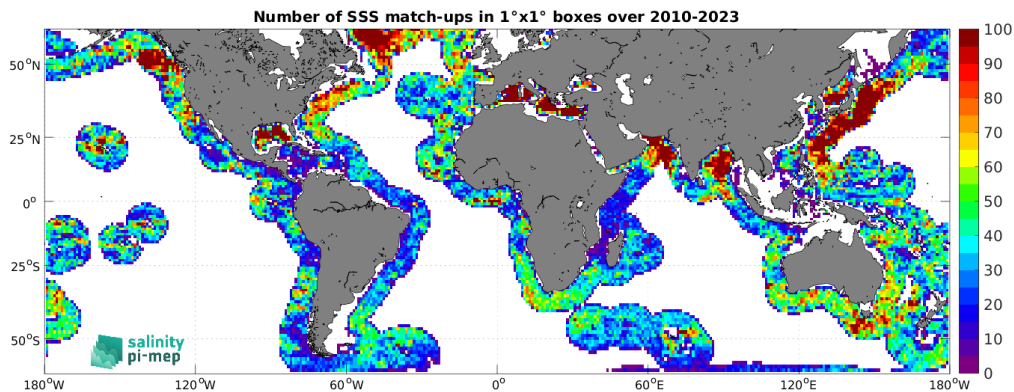
Figure 5: Number of SSS match-ups between Argo SSS and the CCI SSS L4 Merged-OI v5.5 - 7-day running (ESA) SSS product for the SMOS coastal zone ( <800\text{km} ) 60N-60S Pi-MEP region over 1^\circ \times 1^\circ boxes and for the full satellite product period.
