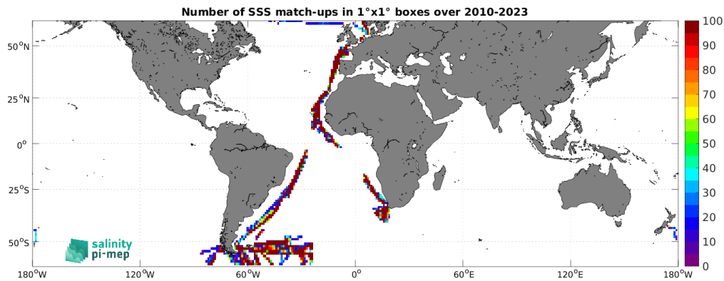
Figure 5: Number of SSS match-ups between TSG (Polarstern) SSS and the CCI SSS L4 Merged-OI v5.5 - 30-day running (ESA) SSS product for the SMOS coastal zone ( <800\text{km} ) 60N-60S Pi-MEP region over 1^\circ \times 1^\circ boxes and for the full satellite product period.
