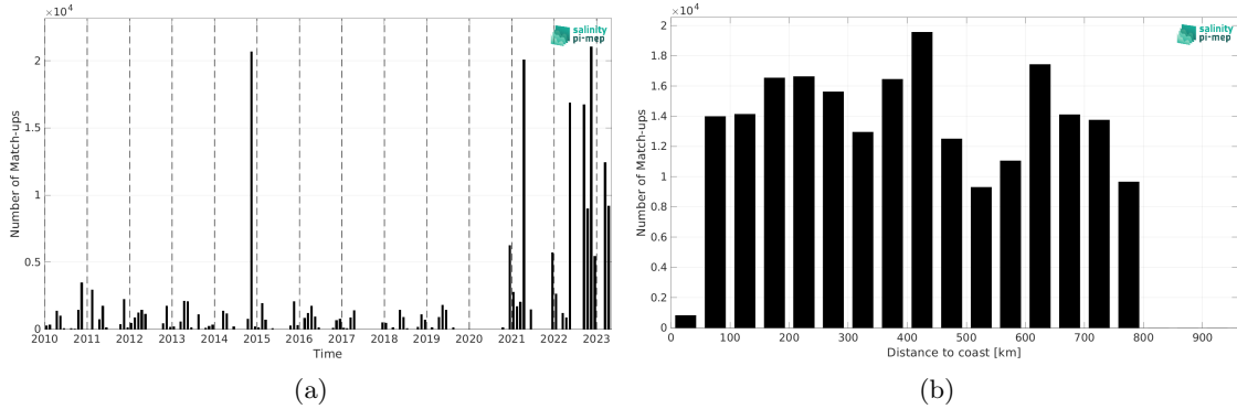
Figure 2: Number of match-ups between TSG (Polarstern) and CCI SSS L4 Merged-OI v5.5 - 30-day running (ESA) SSS as a function of time (a) and as function of the distance to coast (b) over the SMOS coastal zone (<800km) 60N-60S Pi-MEP region and for the full satellite product period.
