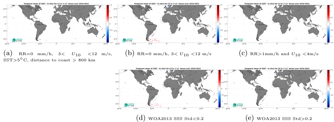
Figure 14: Temporal mean gridded over spatial boxes of size 1^\circ \times 1^\circ of \Delta SSS (CCI SSS L4 Merged-OI v5.5 - 30-day running (ESA) - TSG (Polarstern)) for 5 different subdatasets corresponding to:RR=0 mm/h, 3 < U_{10} < 12 m/s, SST >5^\circ\text{C} , distance to coast > 800 km (a), RR=0 mm/h, 3 < U_{10} < 12 m/s (b), RR >1 mm/h and U_{10} < 4 m/s (c), WOA2013 SSS Std <0.2 (d), WOA2013 SSS Std >0.2 (e).
