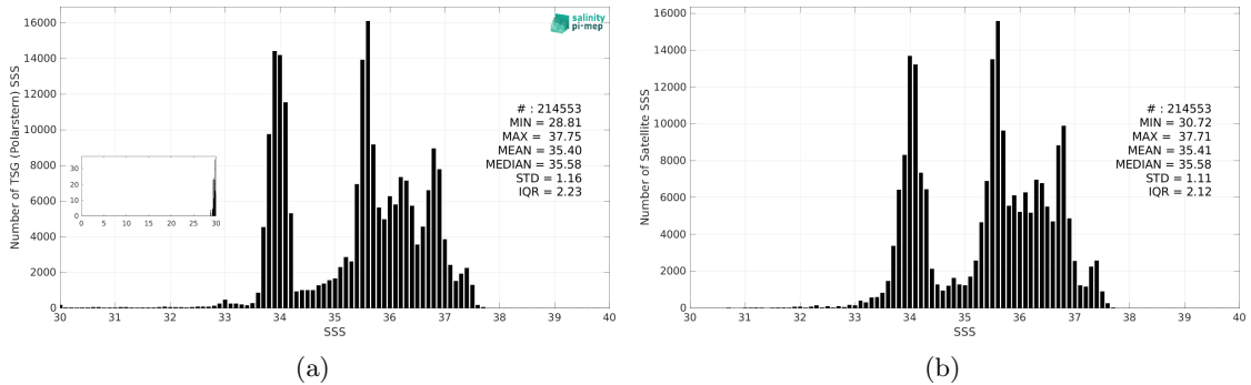
Figure 3: Histograms of SSS from TSG (Polarstern) (a) and CCI SSS L4 Merged-OI v5.5 - 30-day running (ESA) (b) considering all match-up pairs per bins of 0.1 over the SMOS coastal zone (<800km) 60N-60S Pi-MEP region and for the full satellite product period.
