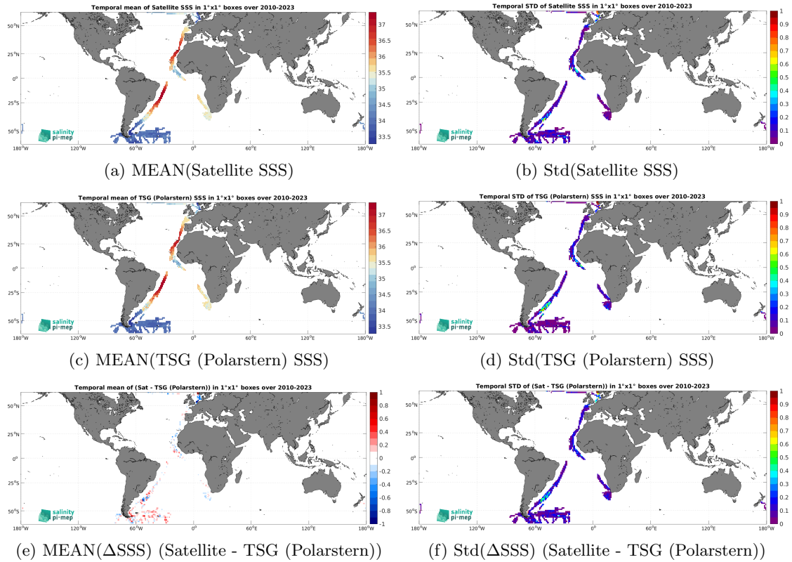
Figure 7: Temporal mean (left) and Std (right) of SSS from CCI SSS L4 Merged-OI v5.5 - 30-day running (ESA) (top), TSG (Polarstern) (middle), and of \Delta SSS (Satellite - TSG (Polarstern)). Only match-up pairs are used to generate these maps.
