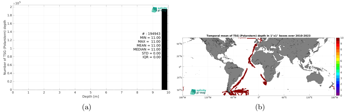
Figure 4: Histograms of the depth of the upper level SSS measurements from TSG (Polarstern) in the Match-up DataBase for the SMOS coastal zone ( <800\text{km} ) 60N-60S Pi-MEP region (a) and temporal mean spatial distribution of pressure of the in situ SSS data over 1^\circ \times 1^\circ boxes and for the full satellite product period (b).
