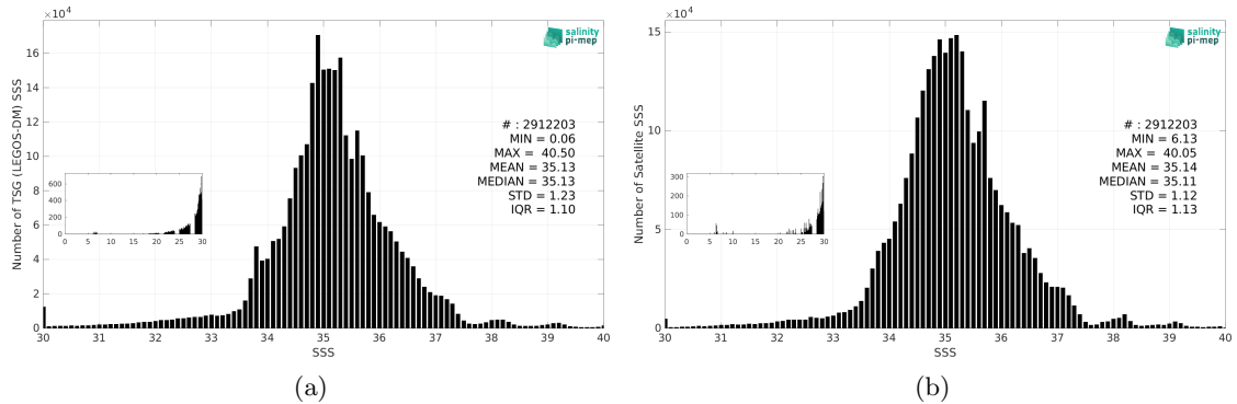
Figure 3: Histograms of SSS from TSG (LEGOS-DM) (a) and CCI SSS L4 Merged-OI v5.5 - 30-day running (ESA) (b) considering all match-up pairs per bins of 0.1 over the SMOS coastal zone (<800km) 60N-60S Pi-MEP region and for the full satellite product period.
