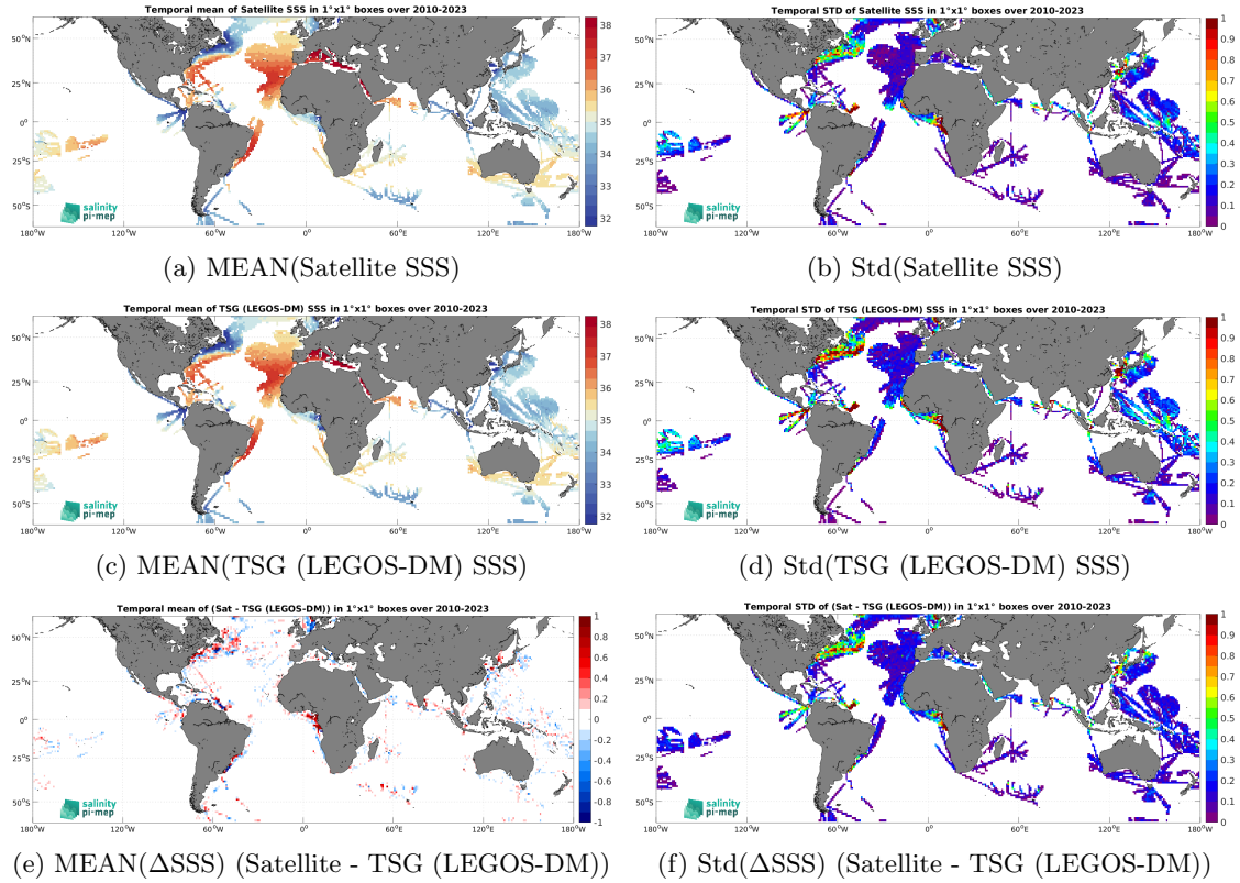
Figure 7: Temporal mean (left) and Std (right) of SSS from CCI SSS L4 Merged-OI v5.5 - 30-day running (ESA) (top), TSG (LEGOS-DM) (middle), and of \Delta SSS (Satellite - TSG (LEGOS-DM)). Only match-up pairs are used to generate these maps.
