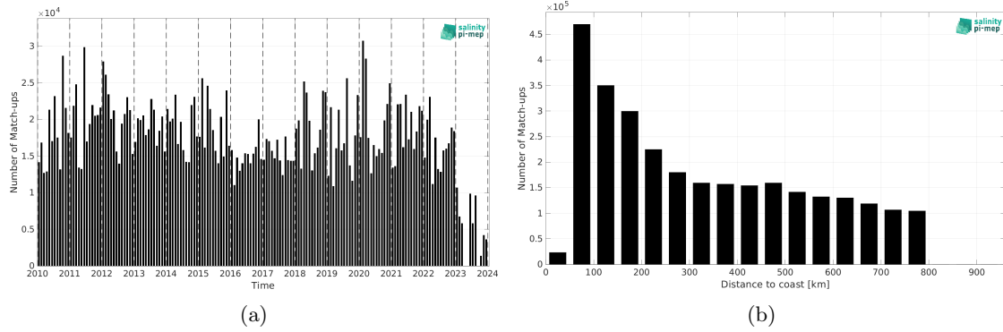
Figure 2: Number of match-ups between TSG (LEGOS-DM) and CCI SSS L4 Merged-OI v5.5 - 30-day running (ESA) SSS as a function of time (a) and as function of the distance to coast (b) over the SMOS coastal zone (<800km) 60N-60S Pi-MEP region and for the full satellite product period.
