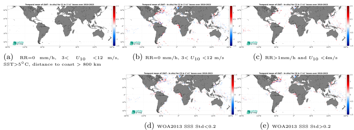
Figure 14: Temporal mean gridded over spatial boxes of size 1^\circ \times 1^\circ of \Delta\text{SSS} (CCI SSS L4 Merged-OI v5.5 - 30-day running (ESA) - TSG (LEGOS-DM)) for 5 different subdatasets corresponding to:RR=0 mm/h, 3 < U_{10} < 12 m/s, SST >5^\circ\text{C} , distance to coast > 800 km (a), RR=0 mm/h, 3 < U_{10} < 12 m/s (b), RR >1 mm/h and U_{10} < 4 m/s (c), WOA2013 SSS Std <0.2 (d), WOA2013 SSS Std >0.2 (e).
