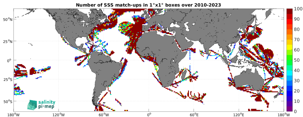
Figure 5: Number of SSS match-ups between TSG (LEGOS-DM) SSS and the CCI SSS L4 Merged-OI v5.5 - 30-day running (ESA) SSS product for the SMOS coastal zone ( <800\text{km} ) 60\text{N} - 60\text{S} Pi-MEP region over 1^\circ \times 1^\circ boxes and for the full satellite product period.
