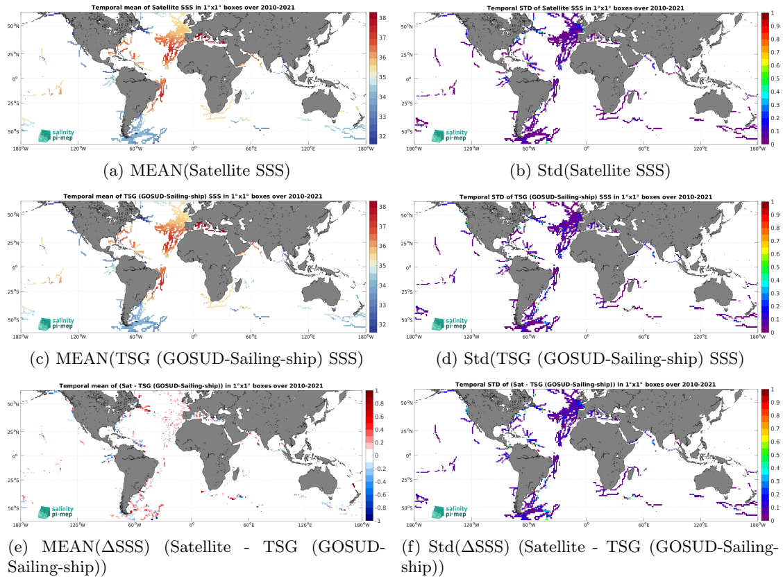
Figure 7: Temporal mean (left) and Std (right) of SSS from CCI SSS L4 Merged-OI v5.5 - 30-day running (ESA) (top), TSG (GOSUD-Sailing-ship) (middle), and of \Delta SSS (Satellite - TSG (GOSUD-Sailing-ship)). Only match-up pairs are used to generate these maps.
