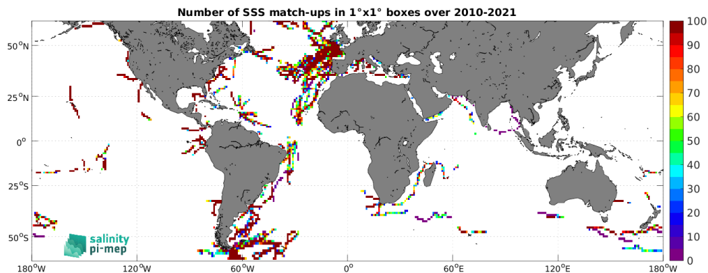
Figure 5: Number of SSS match-ups between TSG (GOSUD-Sailing-ship) SSS and the CCI SSS L4 Merged-OI v5.5 - 30-day running (ESA) SSS product for the SMOS coastal zone ( <800\text{km} ) 60N-60S Pi-MEP region over 1^\circ \times 1^\circ boxes and for the full satellite product period.
