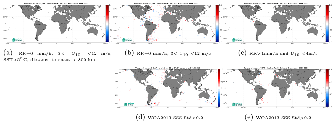
Figure 14: Temporal mean gridded over spatial boxes of size 1^\circ \times 1^\circ of \Delta\text{SSS} (CCI SSS L4 Merged-OI v5.5 - 30-day running (ESA) - TSG (GOSUD-Sailing-ship)) for 5 different subdatasets corresponding to: RR=0 mm/h, 3 < U_{10} < 12 m/s, SST > 5°C, distance to coast > 800 km (a), RR=0 mm/h, 3 < U_{10} < 12 m/s (b), RR > 1mm/h and U_{10} < 4 m/s (c), WOA2013 SSS Std < 0.2 (d), WOA2013 SSS Std > 0.2 (e).
