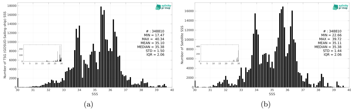
Figure 3: Histograms of SSS from TSG (GOSUD-Sailing-ship) (a) and CCI SSS L4 Merged-OI v5.5 - 30-day running (ESA) (b) considering all match-up pairs per bins of 0.1 over the SMOS coastal zone (<800km) 60N-60S Pi-MEP region and for the full satellite product period.
