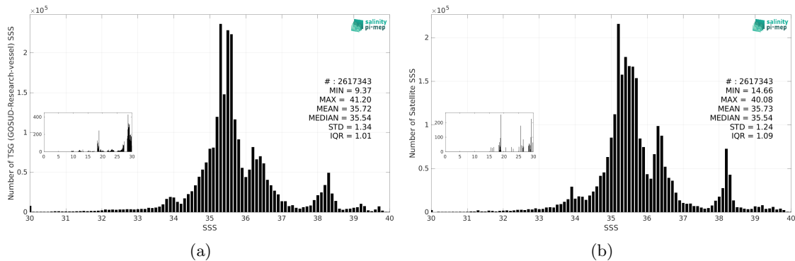
Figure 3: Histograms of SSS from TSG (GOSUD-Research-vessel) (a) and CCI SSS L4 Merged-OI v5.5 - 30-day running (ESA) (b) considering all match-up pairs per bins of 0.1 over the SMOS coastal zone (<800km) 60N-60S Pi-MEP region and for the full satellite product period.
