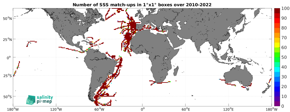
Figure 5: Number of SSS match-ups between TSG (CSIC-UTM) SSS and the CCI SSS L4 Merged-OI v5.5 - 30-day running (ESA) SSS product for the SMOS coastal zone (<800km) 60N-60S Pi-MEP region over 1^\circ \times 1^\circ boxes and for the full satellite product period.
