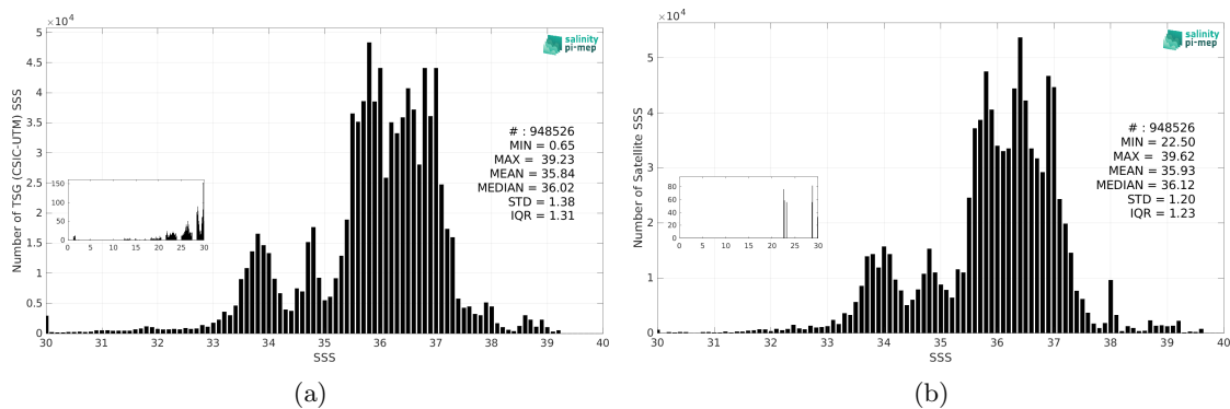
Figure 3: Histograms of SSS from TSG (CSIC-UTM) (a) and CCI SSS L4 Merged-OI v5.5 - 30-day running (ESA) (b) considering all match-up pairs per bins of 0.1 over the SMOS coastal zone (<800km) 60N-60S Pi-MEP region and for the full satellite product period.
