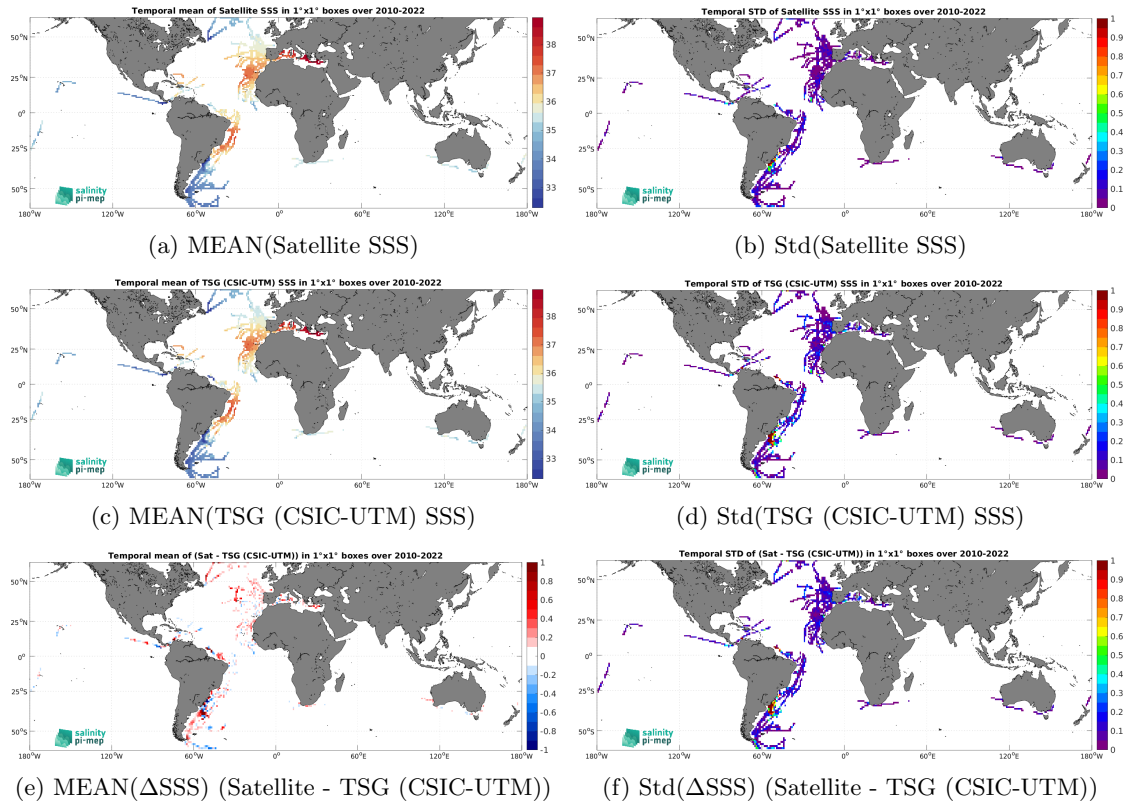
Figure 7: Temporal mean (left) and Std (right) of SSS from CCI SSS L4 Merged-OI v5.5 - 30-day running (ESA) (top), TSG (CSIC-UTM) (middle), and of \Delta SSS (Satellite - TSG (CSIC-UTM)). Only match-up pairs are used to generate these maps.
