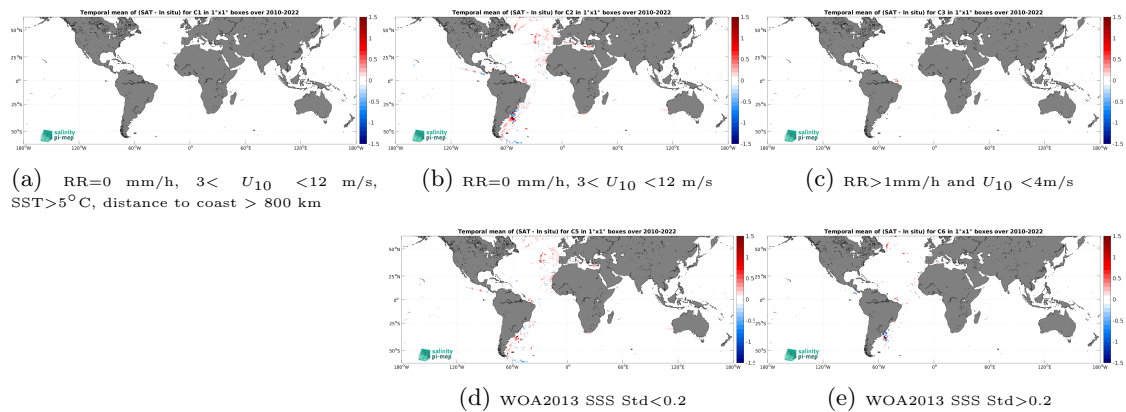
Figure 14: Temporal mean gridded over spatial boxes of size 1^\circ \times 1^\circ of \Delta\text{SSS} (CCI SSS L4 Merged-OI v5.5 - 30-day running (ESA) - TSG (CSIC-UTM)) for 5 different subdatasets corresponding to:RR=0 mm/h, 3 < U_{10} < 12 m/s, SST >5^\circ\text{C} , distance to coast > 800 km (a), RR=0 mm/h, 3 < U_{10} < 12 m/s (b), RR >1 mm/h and U_{10} < 4 m/s (c), WOA2013 SSS Std <0.2 (d), WOA2013 SSS Std >0.2 (e).
