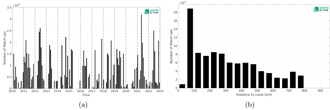
Figure 2: Number of match-ups between TSG (CSIC-UTM) and CCI SSS L4 Merged-OI v5.5 - 30-day running (ESA) SSS as a function of time (a) and as function of the distance to coast (b) over the SMOS coastal zone (<800km) 60N-60S Pi-MEP region and for the full satellite product period.
