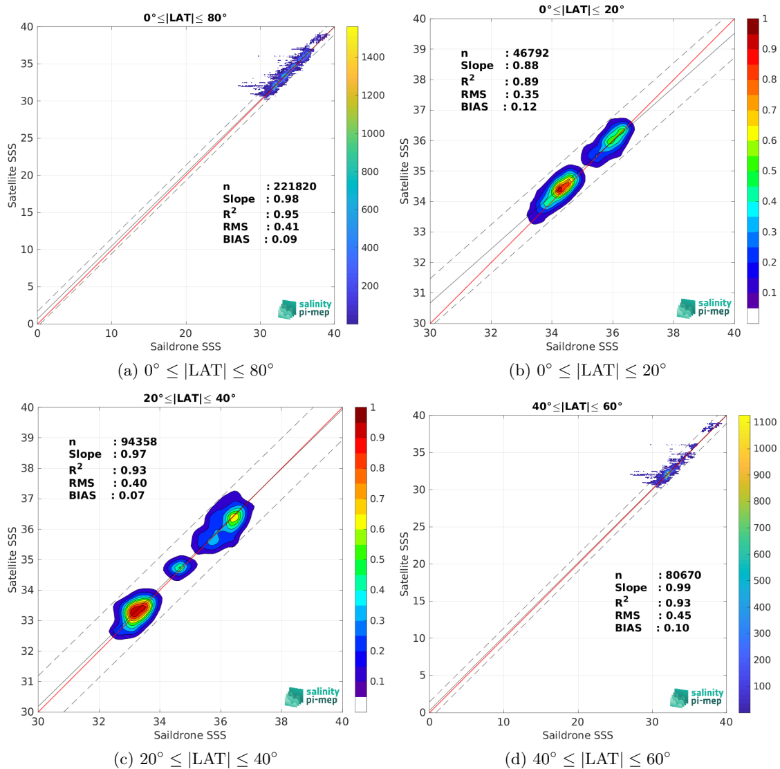
Figure 10: Contour maps of the concentration of CCI SSS L4 Merged-OI v5.5 - 30-day running (ESA) SSS (y-axis) versus Sairdrone SSS (x-axis) at match-up pairs for different latitude bands. For each plot, the red line shows x=y . The black thin and dashed lines indicate a linear fit through the data cloud and the \pm 95\% confidence levels, respectively. The number match-up pairs n , the slope and R^2 coefficient of the linear fit, the root mean square (RMS) and the mean bias between satellite and in situ data are indicated for each latitude band in each plots.
