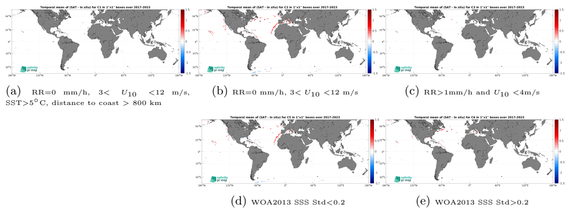
Figure 14: Temporal mean gridded over spatial boxes of size 1^\circ \times 1^\circ of \Delta SSS (CCI SSS L4 Merged-OI v5.5 - 30-day running (ESA) - Saildrone) for 5 different subdatasets corresponding to:RR=0 mm/h, 3 < U_{10} < 12 m/s, SST >5^\circ C, distance to coast > 800 km (a), RR=0 mm/h, 3 < U_{10} < 12 m/s (b), RR >1 mm/h and U_{10} < 4 m/s (c), WOA2013 SSS Std <0.2 (d), WOA2013 SSS Std >0.2 (e).
