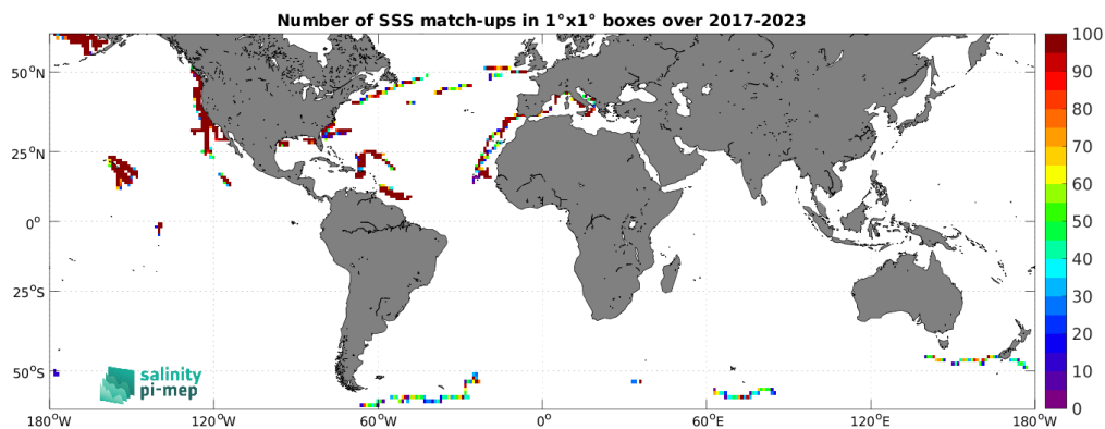
Figure 5: Number of SSS match-ups between Saildrone SSS and the CCI SSS L4 Merged-OI v5.5 - 30-day running (ESA) SSS product for the SMOS coastal zone (<800km) 60N-60S Pi-MEP region over 1^\circ \times 1^\circ boxes and for the full satellite product period.
