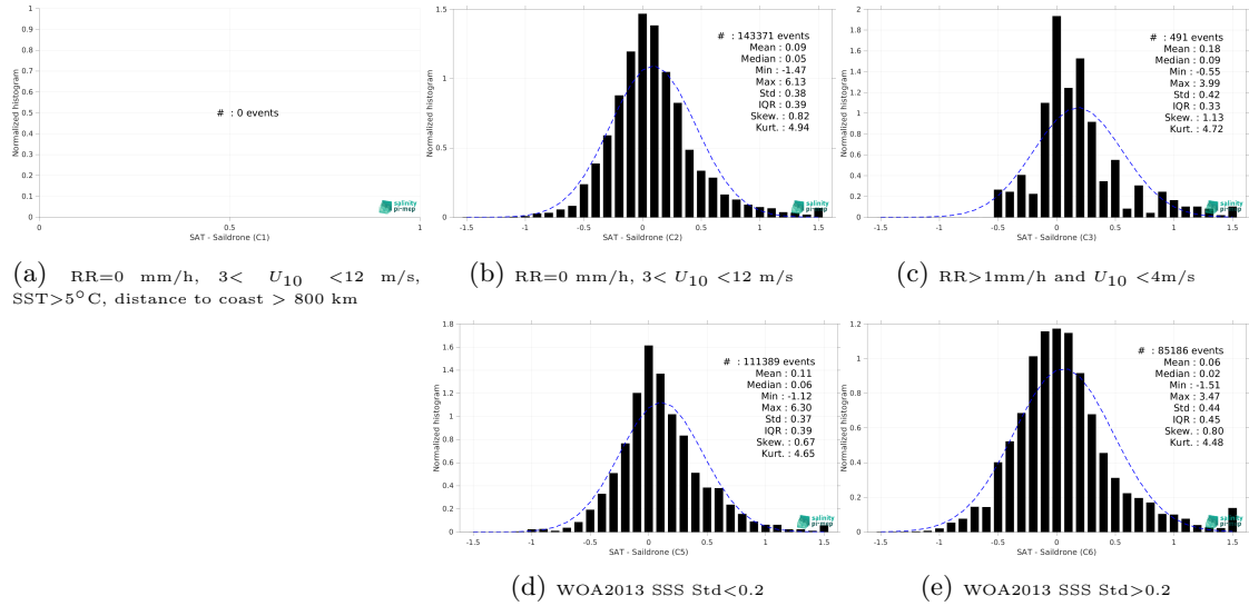
Figure 15: Normalized histogram of \Delta SSS (CCI SSS L4 Merged-OI v5.5 - 30-day running (ESA) - Saikdrone) for 5 different subdatasets corresponding to: RR=0 mm/h, 3 < U_{10} < 12 m/s, SST > 5°C, distance to coast > 800 km (a), RR=0 mm/h, 3 < U_{10} < 12 m/s (b), RR > 1mm/h and U_{10} < 4 m/s (c), WOA2013 SSS Std < 0.2 (d), WOA2013 SSS Std > 0.2 (e).
