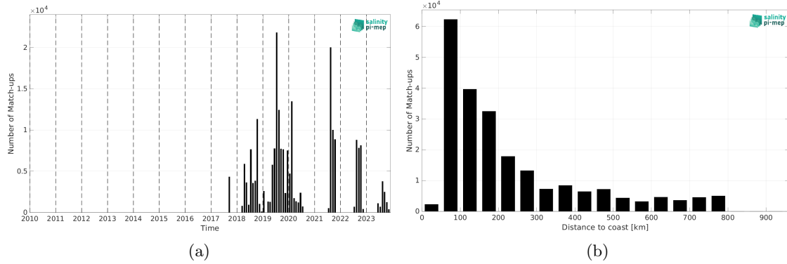
Figure 2: Number of match-ups between Saildrone and CCI SSS L4 Merged-OI v5.5 - 30-day running (ESA) SSS as a function of time (a) and as function of the distance to coast (b) over the SMOS coastal zone (<800km) 60N-60S Pi-MEP region and for the full satellite product period.
