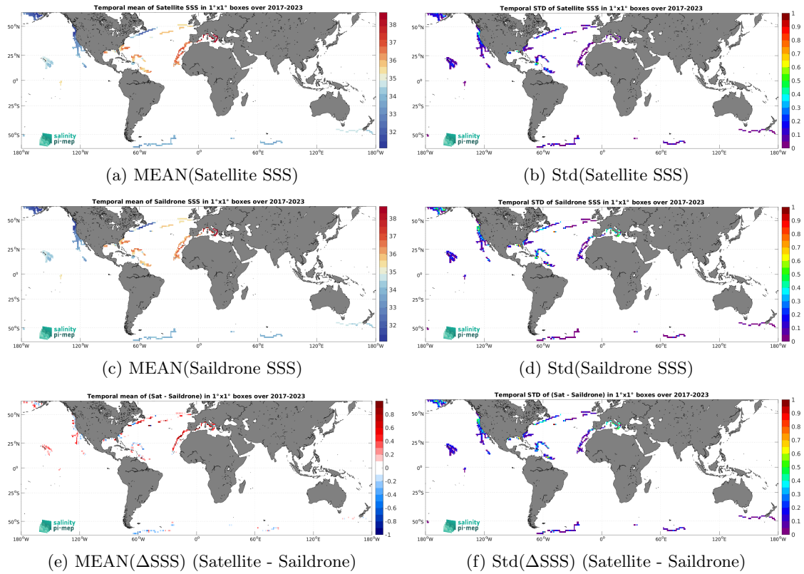
Figure 7: Temporal mean (left) and Std (right) of SSS from CCI SSS L4 Merged-OI v5.5 - 30-day running (ESA) (top), Saildrone (middle), and of \Delta SSS (Satellite - Saildrone). Only match-up pairs are used to generate these maps.
