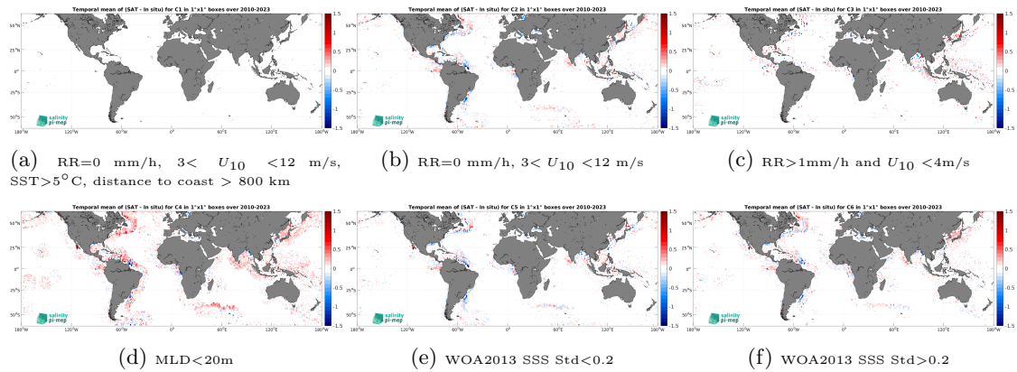
Figure 14: Temporal mean gridded over spatial boxes of size 1^\circ \times 1^\circ of \Delta SSS (CCI SSS L4 Merged-OI v5.5 - 30-day running (ESA) - Argo) for 6 different subdatasets corresponding to:RR=0 mm/h, 3 < U_{10} < 12 m/s, SST >5^\circ C, distance to coast > 800 km (a), RR=0 mm/h, 3 < U_{10} < 12 m/s (b), RR >1 mm/h and U_{10} < 4 m/s (c),MLD <20 m (d),WOA2013 SSS Std <0.2 (e),WOA2013 SSS Std >0.2 (f).
