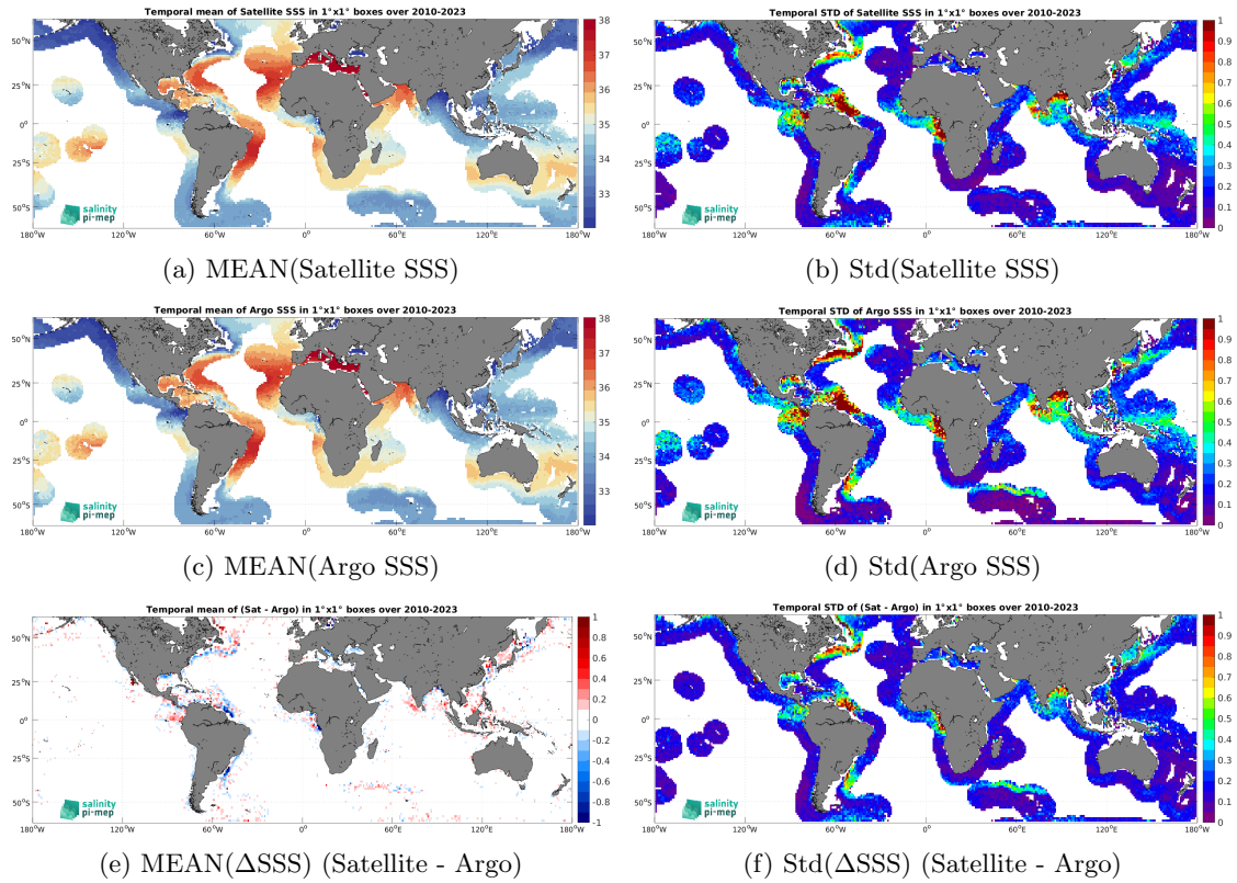
Figure 7: Temporal mean (left) and Std (right) of SSS from CCI SSS L4 Merged-OI v5.5 - 30-day running (ESA) (top), Argo (middle), and of \Delta SSS (Satellite - Argo). Only match-up pairs are used to generate these maps.
