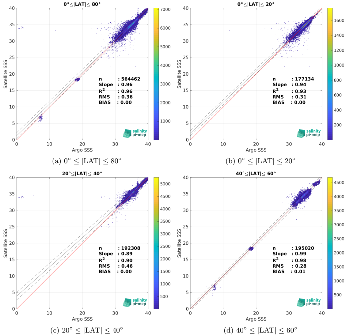
Figure 10: Contour maps of the concentration of CCI SSS L4 Merged-OI v5.5 - 30-day running (ESA) SSS (y-axis) versus Argo SSS (x-axis) at match-up pairs for different latitude bands. For each plot, the red line shows x=y . The black thin and dashed lines indicate a linear fit through the data cloud and the \pm 95\% confidence levels, respectively. The number match-up pairs n , the slope and R^2 coefficient of the linear fit, the root mean square (RMS) and the mean bias between satellite and in situ data are indicated for each latitude band in each plot.
