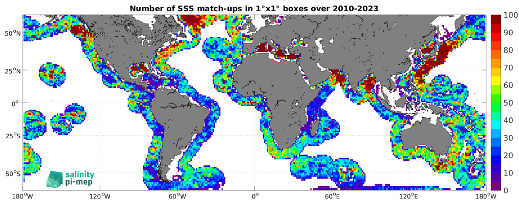
Figure 5: Number of SSS match-ups between Argo SSS and the CCI SSS L4 Merged-OI v5.5 - 30-day running (ESA) SSS product for the SMOS coastal zone (<800km) 60N-60S Pi-MEP region over 1^\circ \times 1^\circ boxes and for the full satellite product period.
