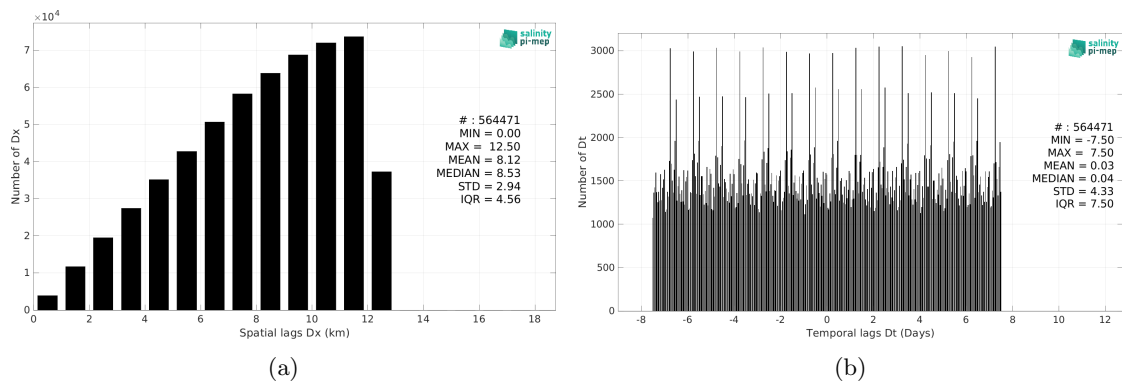
Figure 6: Histograms of the spatial (a) and temporal (b) lags between the location/time of the Argo measurement and the date of the corresponding CCI SSS L4 Merged-OI v5.5 - 30-day running (ESA) SSS pixel.
