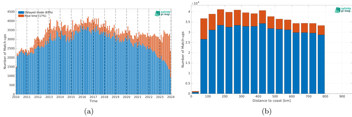
Figure 2: Number of match-ups between Argo and CCI SSS L4 Merged-OI v5.5 - 30-day running (ESA) SSS as a function of time (a) and as function of the distance to coast (b) over the SMOS coastal zone (<800km) 60N-60S Pi-MEP region and for the full satellite product period.
