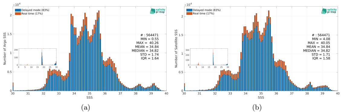
Figure 3: Histograms of SSS from Argo (a) and CCI SSS L4 Merged-OI v5.5 - 30-day running (ESA) (b) considering all match-up pairs per bins of 0.1 over the SMOS coastal zone (<800km) 60N-60S Pi-MEP region and for the full satellite product period.
