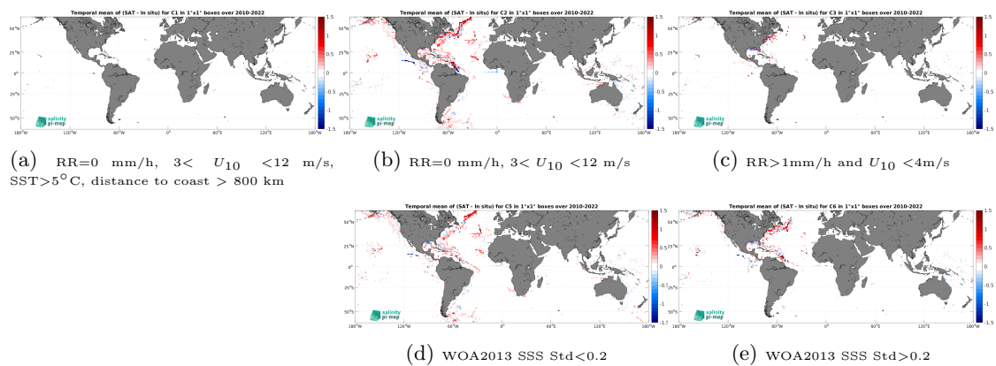
Figure 14: Temporal mean gridded over spatial boxes of size 1^\circ \times 1^\circ of \Delta\text{SSS} (CCI SSS L4 Merged-OI v4.41 - 7-day running (ESA) - TSG (SAMOS)) for 5 different subdatasets corresponding to:RR=0 mm/h, 3 < U_{10} < 12 m/s, SST >5^\circ\text{C} , distance to coast > 800 km (a), RR=0 mm/h, 3 < U_{10} < 12 m/s (b), RR >1 mm/h and U_{10} < 4 m/s (c), WOA2013 SSS Std <0.2 (d), WOA2013 SSS Std >0.2 (e).
