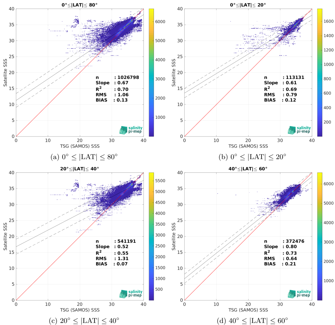
Figure 10: Contour maps of the concentration of CCI SSS L4 Merged-OI v4.41 - 7-day running (ESA) SSS (y-axis) versus TSG (SAMOS) SSS (x-axis) at match-up pairs for different latitude bands. For each plot, the red line shows x=y . The black thin and dashed lines indicate a linear fit through the data cloud and the \pm 95\% confidence levels, respectively. The number match-up pairs n , the slope and R^2 coefficient of the linear fit, the root mean square (RMS) and the mean bias between satellite and in situ data are indicated for each latitude band in each plots.
