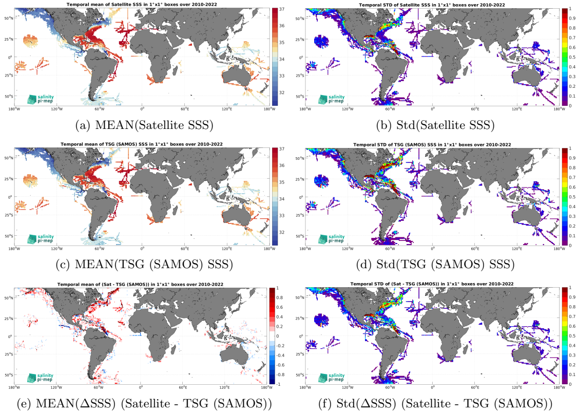
Figure 7: Temporal mean (left) and Std (right) of SSS from CCI SSS L4 Merged-OI v4.41 - 7-day running (ESA) (top), TSG (SAMOS) (middle), and of \Delta SSS (Satellite - TSG (SAMOS)). Only match-up pairs are used to generate these maps.
