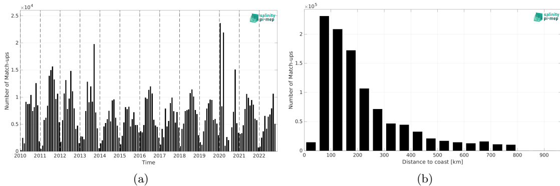
Figure 2: Number of match-ups between TSG (SAMOS) and CCI SSS L4 Merged-OI v4.41 - 7-day running (ESA) SSS as a function of time (a) and as function of the distance to coast (b) over the SMOS coastal zone (<800km) 60N-60S Pi-MEP region and for the full satellite product period.
