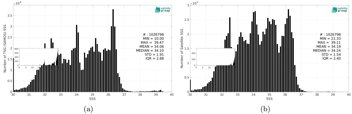
Figure 3: Histograms of SSS from TSG (SAMOS) (a) and CCI SSS L4 Merged-OI v4.41 - 7-day running (ESA) (b) considering all match-up pairs per bins of 0.1 over the SMOS coastal zone (<800km) 60N-60S Pi-MEP region and for the full satellite product period.
