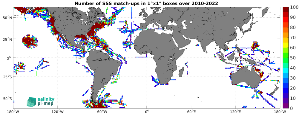
Figure 5: Number of SSS match-ups between TSG (SAMOS) SSS and the CCI SSS L4 Merged-OI v4.41 - 7-day running (ESA) SSS product for the SMOS coastal zone (<800km) 60N-60S Pi-MEP region over 1^\circ \times 1^\circ boxes and for the full satellite product period.
