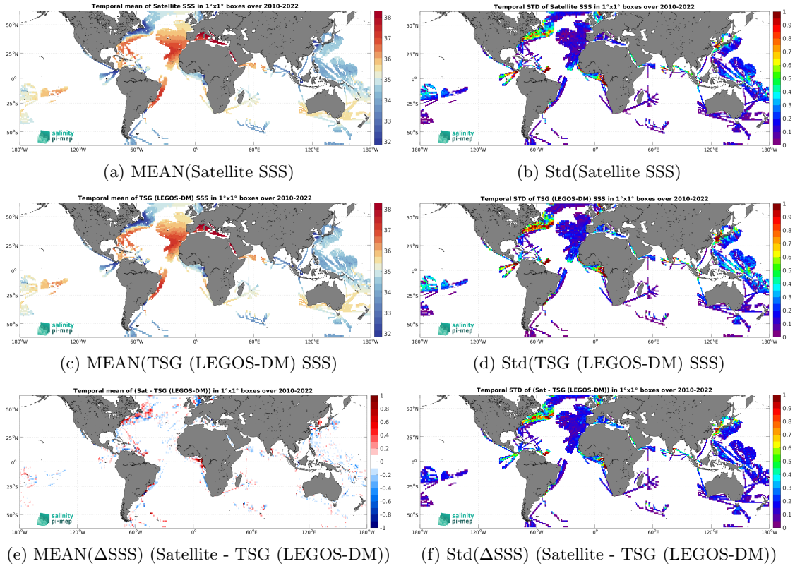
Figure 7: Temporal mean (left) and Std (right) of SSS from CCI SSS L4 Merged-OI v4.41 - 7-day running (ESA) (top), TSG (LEGOS-DM) (middle), and of \Delta SSS (Satellite - TSG (LEGOS-DM)). Only match-up pairs are used to generate these maps.
