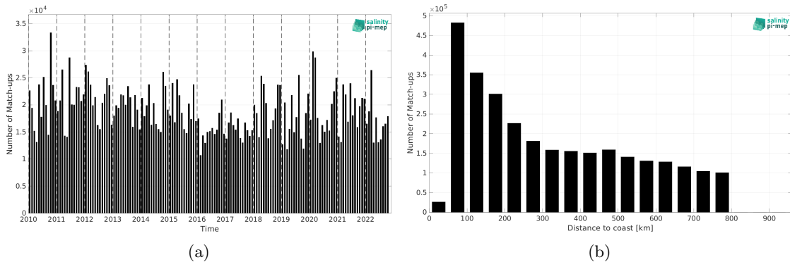
Figure 2: Number of match-ups between TSG (LEGOS-DM) and CCI SSS L4 Merged-OI v4.41 - 7-day running (ESA) SSS as a function of time (a) and as function of the distance to coast (b) over the SMOS coastal zone (<800km) 60N-60S Pi-MEP region and for the full satellite product period.
