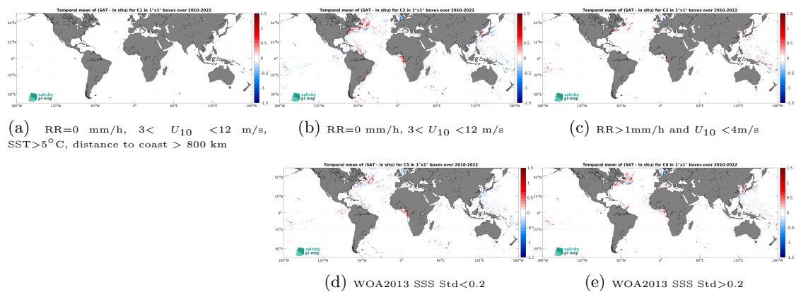
Figure 14: Temporal mean gridded over spatial boxes of size 1^\circ \times 1^\circ of \Delta\text{SSS} (CCI SSS L4 Merged-OI v4.41 - 7-day running (ESA) - TSG (LEGOS-DM)) for 5 different subdatasets corresponding to:RR=0 mm/h, 3 < U_{10} < 12 m/s, SST >5^\circ\text{C} , distance to coast > 800 km (a), RR=0 mm/h, 3 < U_{10} < 12 m/s (b), RR >1 mm/h and U_{10} < 4 m/s (c), WOA2013 SSS Std <0.2 (d), WOA2013 SSS Std >0.2 (e).
