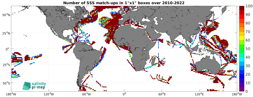
Figure 5: Number of SSS match-ups between TSG (LEGOS-DM) SSS and the CCI SSS L4 Merged-OI v4.41 - 7-day running (ESA) SSS product for the SMOS coastal zone (<800km) 60N-60S Pi-MEP region over 1^{\circ} \times 1^{\circ} boxes and for the full satellite product period.
