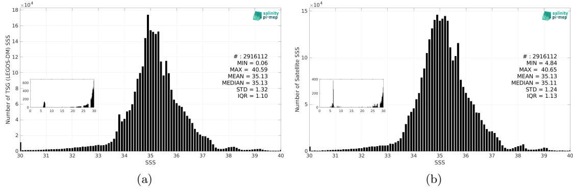
Figure 3: Histograms of SSS from TSG (LEGOS-DM) (a) and CCI SSS L4 Merged-OI v4.41 - 7-day running (ESA) (b) considering all match-up pairs per bins of 0.1 over the SMOS coastal zone (<800km) 60N-60S Pi-MEP region and for the full satellite product period.
