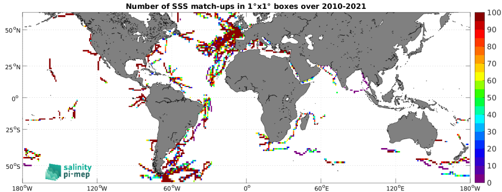
Figure 5: Number of SSS match-ups between TSG (GOSUD-Sailing-ship) SSS and the CCI SSS L4 Merged-OI v4.41 - 7-day running (ESA) SSS product for the SMOS coastal zone ( <800\text{km} ) 60N-60S Pi-MEP region over 1^\circ \times 1^\circ boxes and for the full satellite product period.
