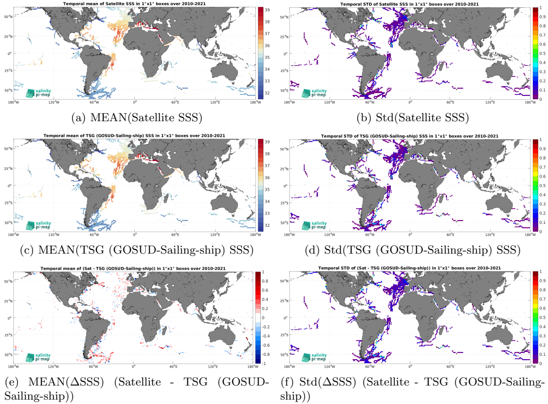
Figure 7: Temporal mean (left) and Std (right) of SSS from CCI SSS L4 Merged-OI v4.41 - 7-day running (ESA) (top), TSG (GOSUD-Sailing-ship) (middle), and of \Delta\text{SSS} (Satellite - TSG (GOSUD-Sailing-ship)). Only match-up pairs are used to generate these maps.
