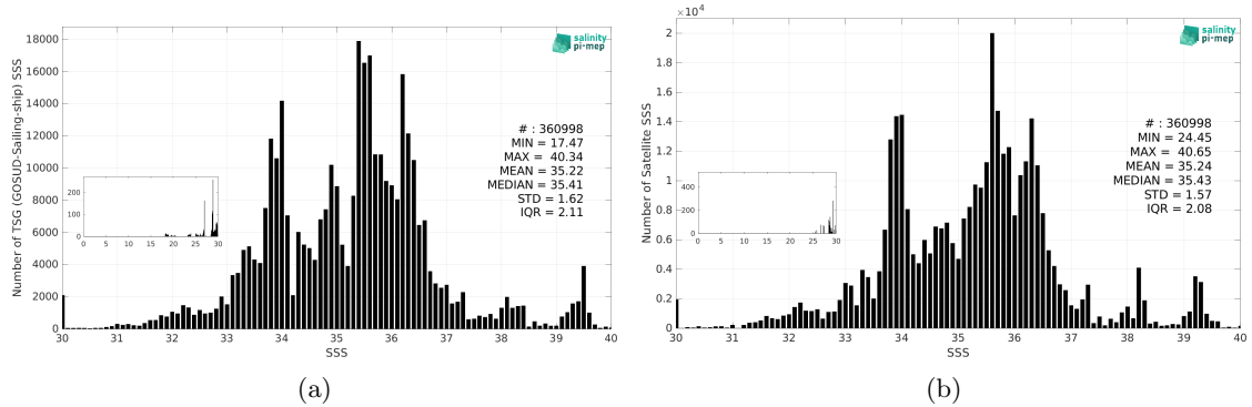
Figure 3: Histograms of SSS from TSG (GOSUD-Sailing-ship) (a) and CCI SSS L4 Merged-OI v4.41 - 7-day running (ESA) (b) considering all match-up pairs per bins of 0.1 over the SMOS coastal zone (<800km) 60N-60S Pi-MEP region and for the full satellite product period.
