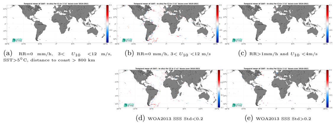
Figure 14: Temporal mean gridded over spatial boxes of size 1^\circ \times 1^\circ of \Delta\text{SSS} (CCI SSS L4 Merged-OI v4.41 - 7-day running (ESA) - TSG (GOSUD-Sailing-ship)) for 5 different subdatasets corresponding to: RR=0 mm/h, 3 < U_{10} < 12 m/s, SST > 5^\circ\text{C} , distance to coast > 800 km (a), RR=0 mm/h, 3 < U_{10} < 12 m/s (b), RR > 1 mm/h and U_{10} < 4 m/s (c), WOA2013 SSS Std < 0.2 (d), WOA2013 SSS Std > 0.2 (e).
