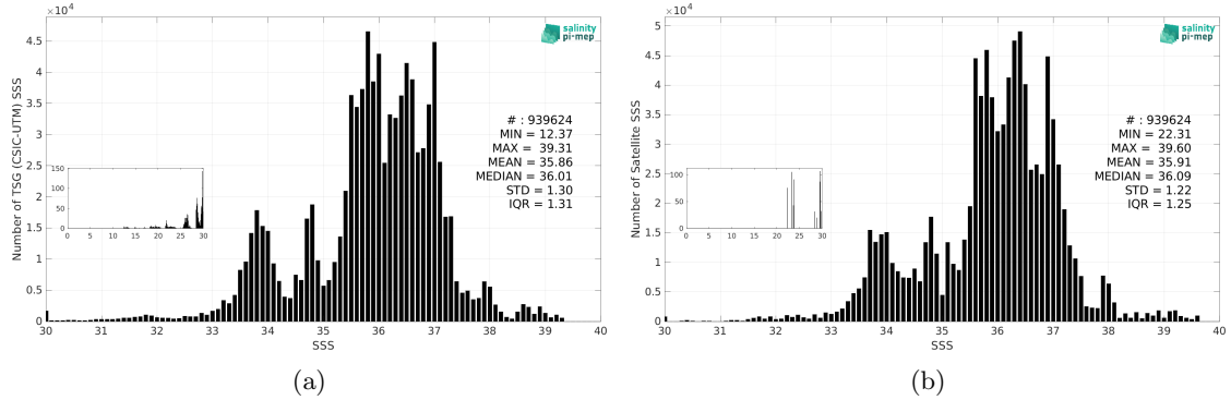
Figure 3: Histograms of SSS from TSG (CSIC-UTM) (a) and CCI SSS L4 Merged-OI v4.41 - 7-day running (ESA) (b) considering all match-up pairs per bins of 0.1 over the SMOS coastal zone (<800km) 60N-60S Pi-MEP region and for the full satellite product period.
