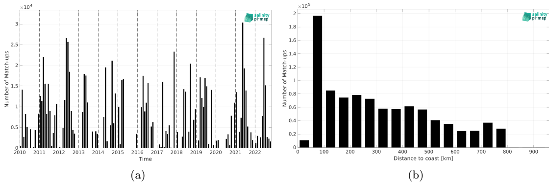
Figure 2: Number of match-ups between TSG (CSIC-UTM) and CCI SSS L4 Merged-OI v4.41 - 7-day running (ESA) SSS as a function of time (a) and as function of the distance to coast (b) over the SMOS coastal zone (<800km) 60N-60S Pi-MEP region and for the full satellite product period.
