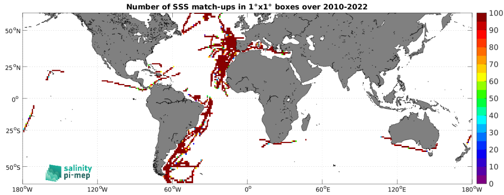
Figure 5: Number of SSS match-ups between TSG (CSIC-UTM) SSS and the CCI SSS L4 Merged-OI v4.41 - 7-day running (ESA) SSS product for the SMOS coastal zone (<800km) 60N-60S Pi-MEP region over 1^{\circ} \times 1^{\circ} boxes and for the full satellite product period.
