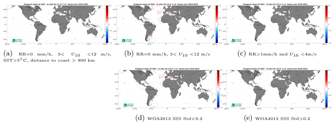
Figure 14: Temporal mean gridded over spatial boxes of size 1^\circ \times 1^\circ of \Delta\text{SSS} (CCI SSS L4 Merged-OI v4.41 - 7-day running (ESA) - TSG (CSIC-UTM)) for 5 different subdatasets corresponding to:RR=0 mm/h, 3 < U_{10} < 12 m/s, SST >5^\circ\text{C} , distance to coast > 800 km (a), RR=0 mm/h, 3 < U_{10} < 12 m/s (b), RR >1 mm/h and U_{10} < 4 m/s (c), WOA2013 SSS Std <0.2 (d), WOA2013 SSS Std >0.2 (e).
