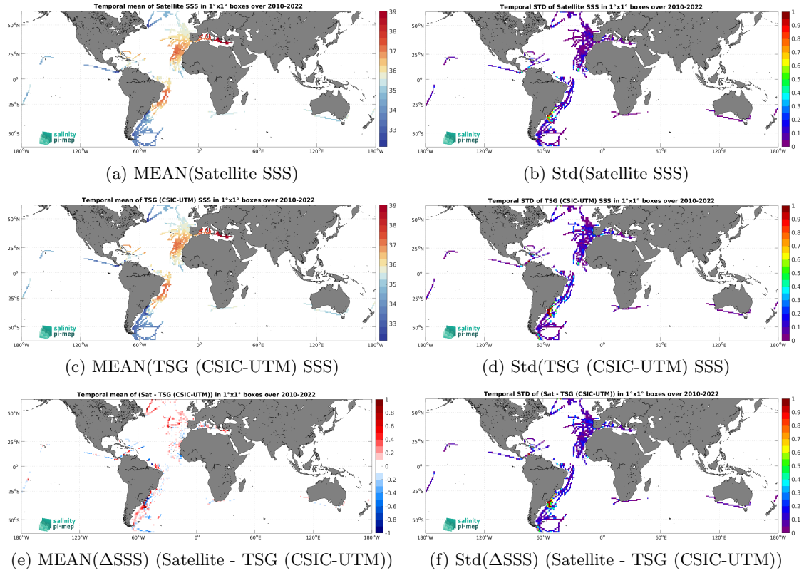
Figure 7: Temporal mean (left) and Std (right) of SSS from CCI SSS L4 Merged-OI v4.41 - 7-day running (ESA) (top), TSG (CSIC-UTM) (middle), and of \Delta SSS (Satellite - TSG (CSIC-UTM)). Only match-up pairs are used to generate these maps.
