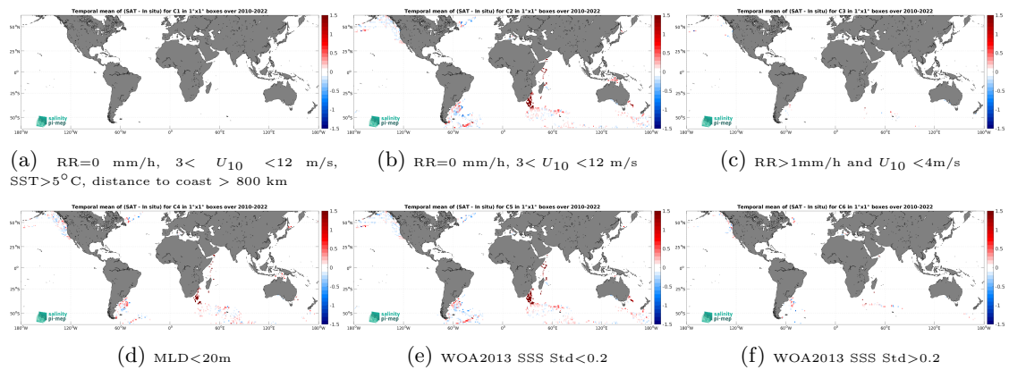
Figure 14: Temporal mean gridded over spatial boxes of size 1^\circ \times 1^\circ of \Delta SSS (CCI SSS L4 Merged-OI v4.41 - 7-day running (ESA) - Marine mammals) for 6 different subdatasets corresponding to:RR=0 mm/h, 3 < U_{10} < 12 m/s, SST >5^\circ C, distance to coast > 800 km (a), RR=0 mm/h, 3 < U_{10} < 12 m/s (b), RR >1 mm/h and U_{10} < 4 m/s (c),MLD <20 m (d),WOA2013 SSS Std <0.2 (e),WOA2013 SSS Std >0.2 (f).
