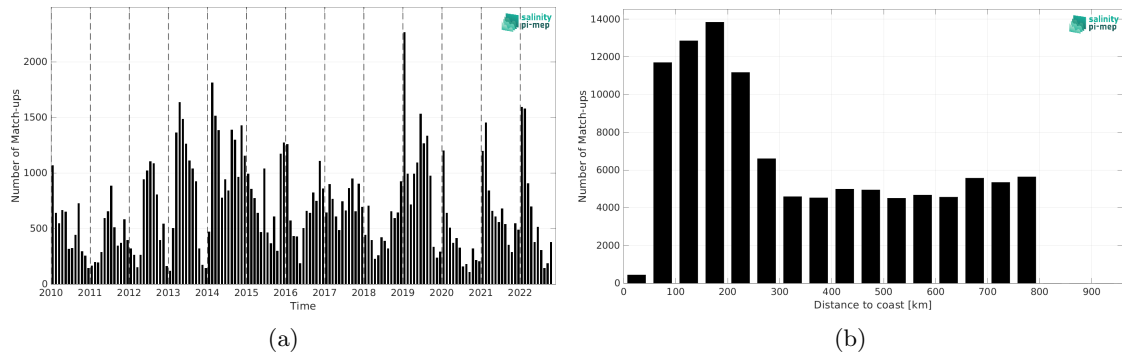
Figure 2: Number of match-ups between Marine mammals and CCI SSS L4 Merged-OI v4.41 - 7-day running (ESA) SSS as a function of time (a) and as function of the distance to coast (b) over the SMOS coastal zone (<800km) 60N-60S Pi-MEP region and for the full satellite product period.
