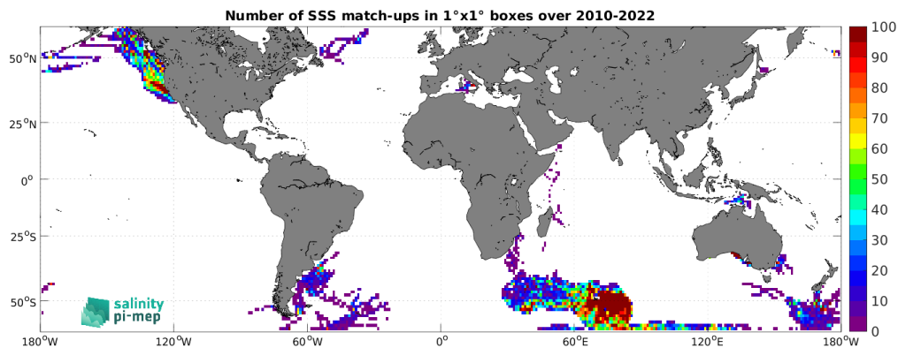
Figure 5: Number of SSS match-ups between Marine mammals SSS and the CCI SSS L4 Merged-OI v4.41 - 7-day running (ESA) SSS product for the SMOS coastal zone (<800km) 60N-60S Pi-MEP region over 1^\circ \times 1^\circ boxes and for the full satellite product period.
