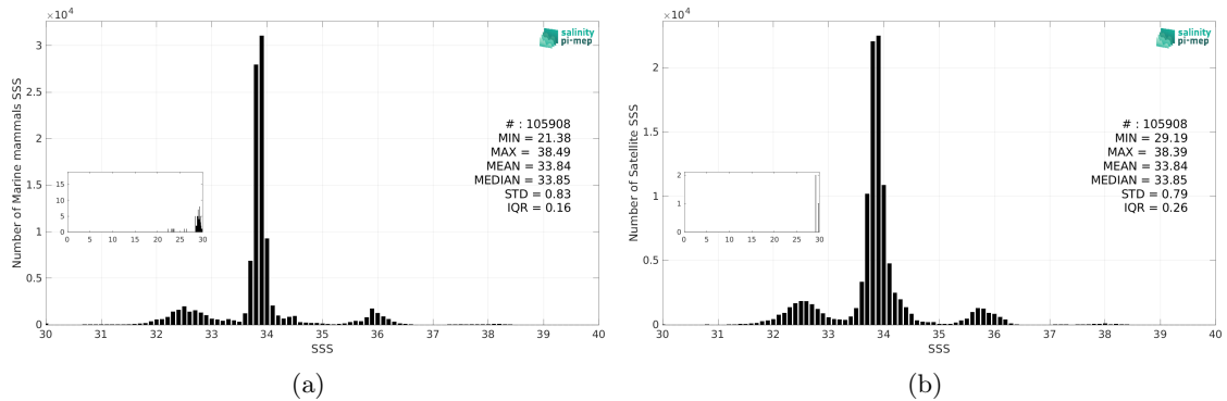
Figure 3: Histograms of SSS from Marine mammals (a) and CCI SSS L4 Merged-OI v4.41 - 7-day running (ESA) (b) considering all match-up pairs per bins of 0.1 over the SMOS coastal zone (<800km) 60N-60S Pi-MEP region and for the full satellite product period.
