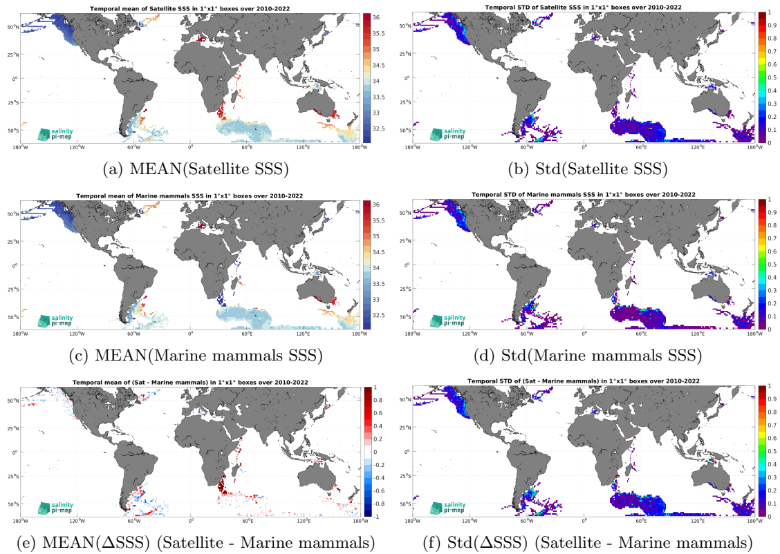
Figure 7: Temporal mean (left) and Std (right) of SSS from CCI SSS L4 Merged-OI v4.41 - 7-day running (ESA) (top), Marine mammals (middle), and of \Delta SSS (Satellite - Marine mammals). Only match-up pairs are used to generate these maps.
