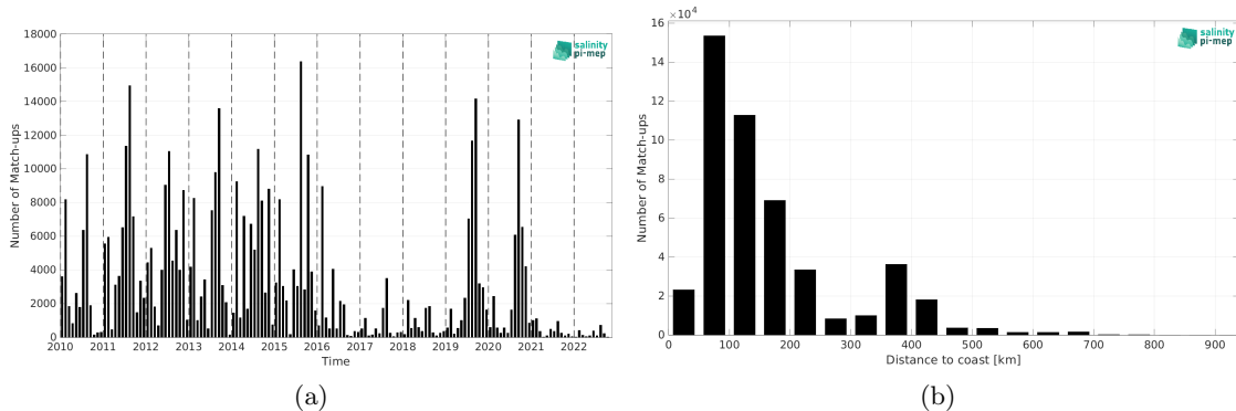
Figure 2: Number of match-ups between ICES and CCI SSS L4 Merged-OI v4.41 - 7-day running (ESA) SSS as a function of time (a) and as function of the distance to coast (b) over the SMOS coastal zone (<800km) 60N-60S Pi-MEP region and for the full satellite product period.
