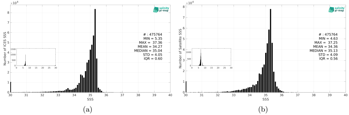
Figure 3: Histograms of SSS from ICES (a) and CCI SSS L4 Merged-OI v4.41 - 7-day running (ESA) (b) considering all match-up pairs per bins of 0.1 over the SMOS coastal zone (<800km) 60N-60S Pi-MEP region and for the full satellite product period.
