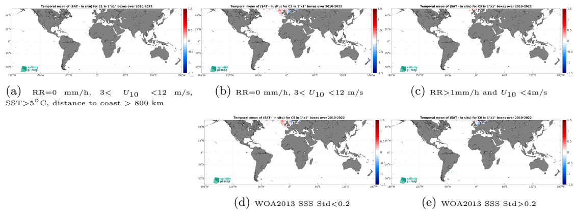
Figure 14: Temporal mean gridded over spatial boxes of size 1^\circ \times 1^\circ of \Delta SSS (CCI SSS L4 Merged-OI v4.41 - 7-day running (ESA) - ICES) for 5 different subdatasets corresponding to:RR=0 mm/h, 3 < U_{10} < 12 m/s, SST >5^\circ\text{C} , distance to coast > 800 km (a), RR=0 mm/h, 3 < U_{10} < 12 m/s (b), RR >1 mm/h and U_{10} < 4 m/s (c), WOA2013 SSS Std <0.2 (d), WOA2013 SSS Std >0.2 (e).
