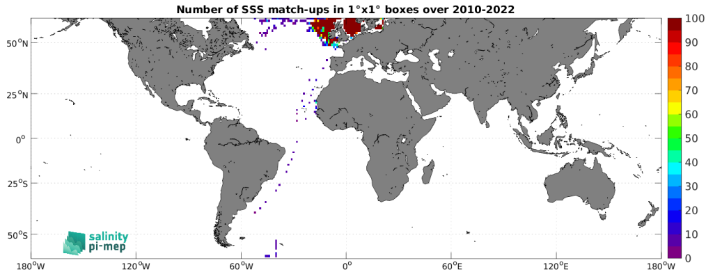
Figure 5: Number of SSS match-ups between ICES SSS and the CCI SSS L4 Merged-OI v4.41 - 7-day running (ESA) SSS product for the SMOS coastal zone (<800km) 60N-60S Pi-MEP region over 1^\circ \times 1^\circ boxes and for the full satellite product period.
