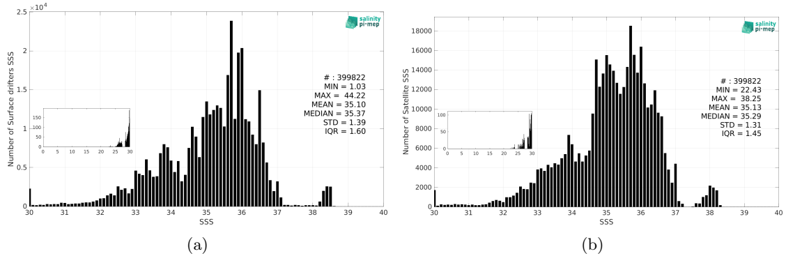
Figure 3: Histograms of SSS from Surface drifters (a) and CCI SSS L4 Merged-OI v4.41 - 7-day running (ESA) (b) considering all match-up pairs per bins of 0.1 over the SMOS coastal zone (<800km) 60N-60S Pi-MEP region and for the full satellite product period.
