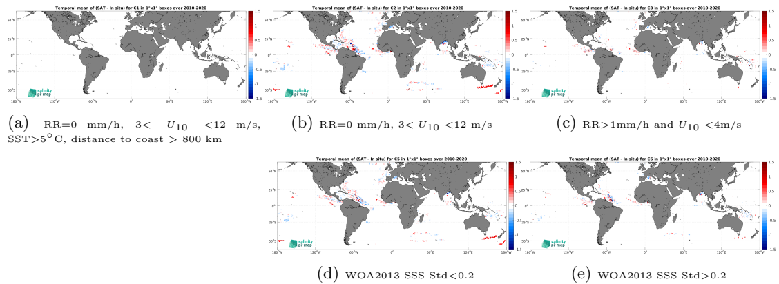
Figure 13: Temporal mean gridded over spatial boxes of size 1^\circ \times 1^\circ of \Delta\text{SSS} (CCI SSS L4 Merged-OI v4.41 - 7-day running (ESA) - Surface drifters) for 5 different subdatasets corresponding to:RR=0 mm/h, 3 < U_{10} < 12 m/s, SST >5^\circ\text{C} , distance to coast > 800 km (a), RR=0 mm/h, 3 < U_{10} < 12 m/s (b), RR >1 mm/h and U_{10} < 4 m/s (c), WOA2013 SSS Std <0.2 (d), WOA2013 SSS Std >0.2 (e).
