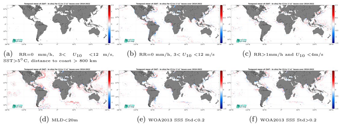
Figure 14: Temporal mean gridded over spatial boxes of size 1^\circ \times 1^\circ of \Delta SSS (CCI SSS L4 Merged-OI v4.41 - 7-day running (ESA) - Argo) for 6 different subdatasets corresponding to:RR=0 mm/h, 3 < U_{10} < 12 m/s, SST >5^\circ C, distance to coast > 800 km (a), RR=0 mm/h, 3 < U_{10} < 12 m/s (b), RR >1 mm/h and U_{10} < 4 m/s (c),MLD <20 m (d),WOA2013 SSS Std <0.2 (e),WOA2013 SSS Std >0.2 (f).
