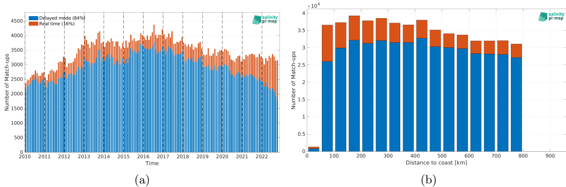
Figure 2: Number of match-ups between Argo and CCI SSS L4 Merged-OI v4.41 - 7-day running (ESA) SSS as a function of time (a) and as function of the distance to coast (b) over the SMOS coastal zone (<800km) 60N-60S Pi-MEP region and for the full satellite product period.
