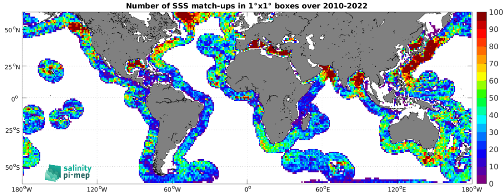
Figure 5: Number of SSS match-ups between Argo SSS and the CCI SSS L4 Merged-OI v4.41 - 7-day running (ESA) SSS product for the SMOS coastal zone (<800km) 60N-60S Pi-MEP region over 1^\circ \times 1^\circ boxes and for the full satellite product period.
