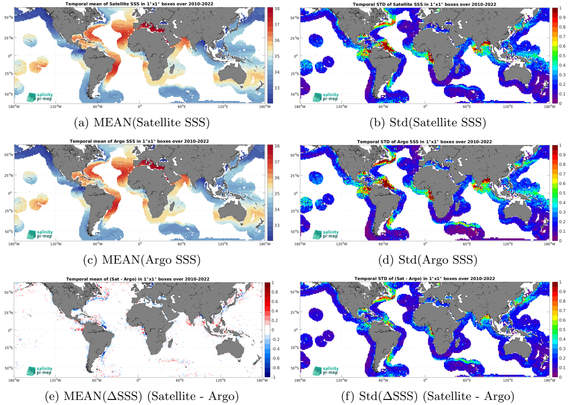
Figure 7: Temporal mean (left) and Std (right) of SSS from CCI SSS L4 Merged-OI v4.41 - 7-day running (ESA) (top), Argo (middle), and of \Delta SSS (Satellite - Argo). Only match-up pairs are used to generate these maps.
