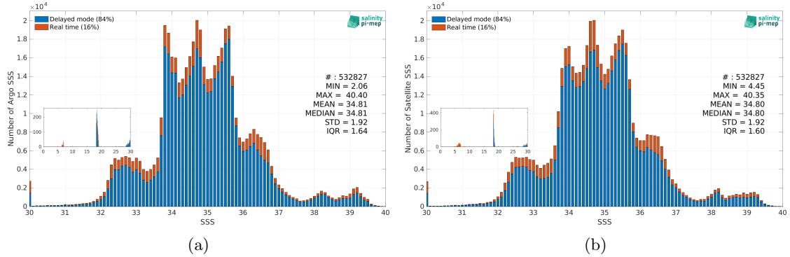
Figure 3: Histograms of SSS from Argo (a) and CCI SSS L4 Merged-OI v4.41 - 7-day running (ESA) (b) considering all match-up pairs per bins of 0.1 over the SMOS coastal zone (<800km) 60N-60S Pi-MEP region and for the full satellite product period.
