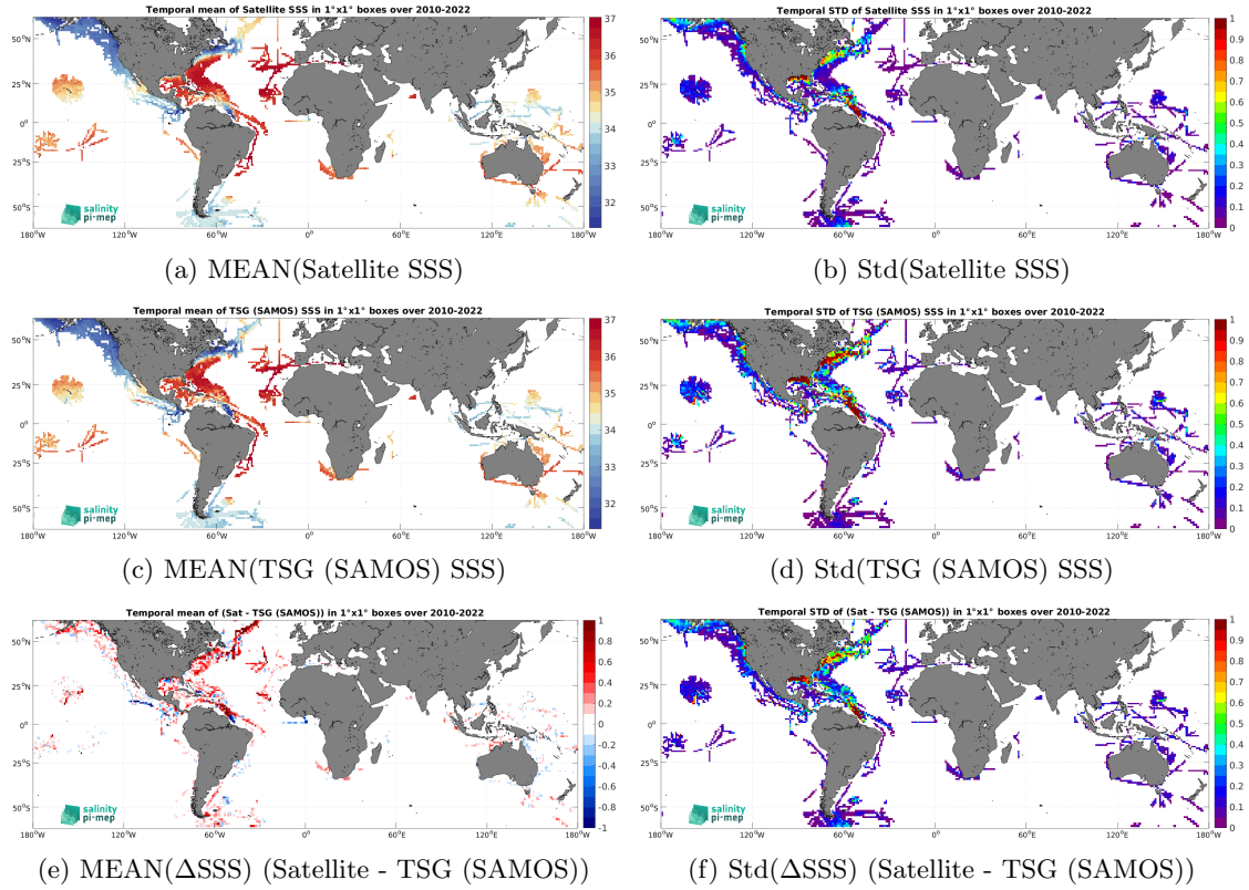
Figure 7: Temporal mean (left) and Std (right) of SSS from CCI SSS L4 Merged-OI v4.41 - 30-day running (ESA) (top), TSG (SAMOS) (middle), and of \Delta SSS (Satellite - TSG (SAMOS)). Only match-up pairs are used to generate these maps.
