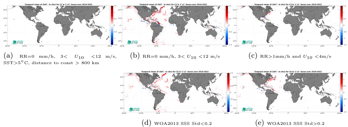
Figure 14: Temporal mean gridded over spatial boxes of size 1^\circ \times 1^\circ of \Delta SSS (CCI SSS L4 Merged-OI v4.41 - 30-day running (ESA) - TSG (SAMOS)) for 5 different subdatasets corresponding to:RR=0 mm/h, 3 < U_{10} < 12 m/s, SST >5^\circ\text{C} , distance to coast > 800 km (a), RR=0 mm/h, 3 < U_{10} < 12 m/s (b), RR >1 mm/h and U_{10} < 4 m/s (c), WOA2013 SSS Std <0.2 (d), WOA2013 SSS Std >0.2 (e).
