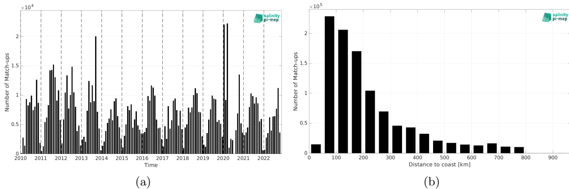
Figure 2: Number of match-ups between TSG (SAMOS) and CCI SSS L4 Merged-OI v4.41 - 30-day running (ESA) SSS as a function of time (a) and as function of the distance to coast (b) over the SMOS coastal zone (<800km) 60N-60S Pi-MEP region and for the full satellite product period.
