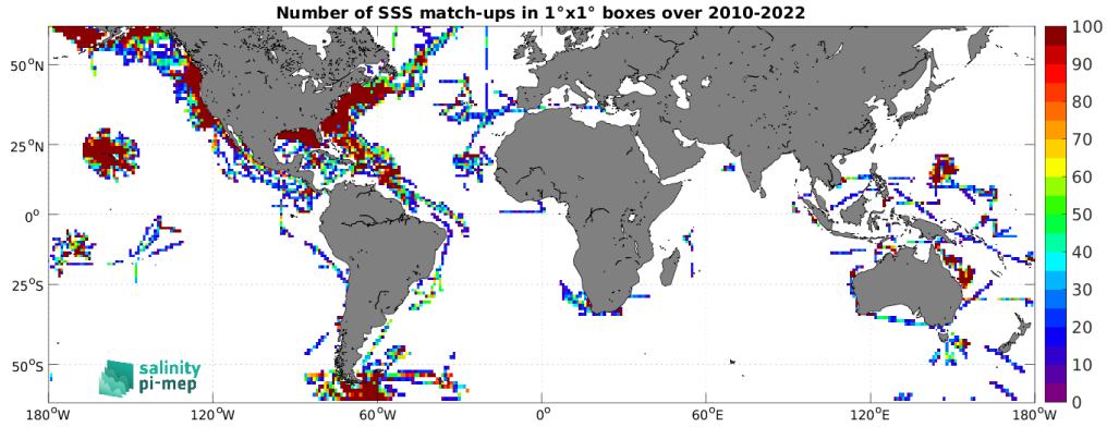
Figure 5: Number of SSS match-ups between TSG (SAMOS) SSS and the CCI SSS L4 Merged-OI v4.41 - 30-day running (ESA) SSS product for the SMOS coastal zone (<800km) 60N-60S Pi-MEP region over 1^\circ \times 1^\circ boxes and for the full satellite product period.
