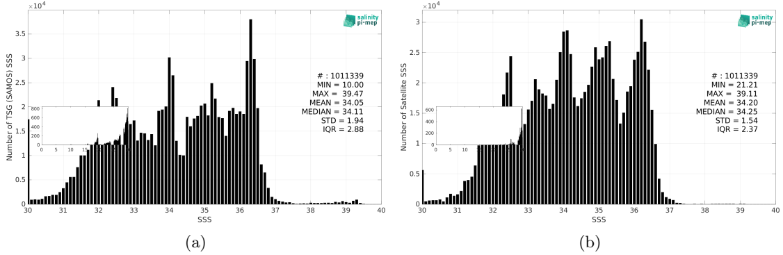
Figure 3: Histograms of SSS from TSG (SAMOS) (a) and CCI SSS L4 Merged-OI v4.41 - 30-day running (ESA) (b) considering all match-up pairs per bins of 0.1 over the SMOS coastal zone (<800km) 60N-60S Pi-MEP region and for the full satellite product period.
