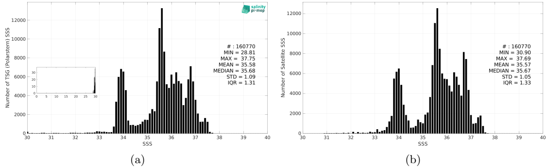
Figure 3: Histograms of SSS from TSG (Polarstern) (a) and CCI SSS L4 Merged-OI v4.41 - 30-day running (ESA) (b) considering all match-up pairs per bins of 0.1 over the SMOS coastal zone (<800km) 60N-60S Pi-MEP region and for the full satellite product period.
