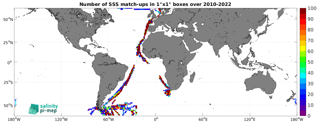
Figure 5: Number of SSS match-ups between TSG (Polarstern) SSS and the CCI SSS L4 Merged-OI v4.41 - 30-day running (ESA) SSS product for the SMOS coastal zone (<800km) 60N-60S Pi-MEP region over 1^\circ \times 1^\circ boxes and for the full satellite product period.
