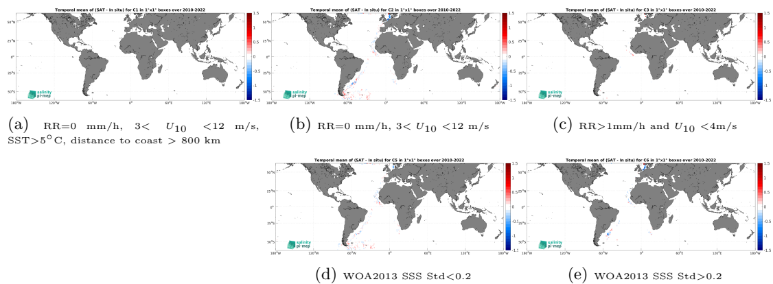
Figure 14: Temporal mean gridded over spatial boxes of size 1^\circ \times 1^\circ of \Delta\text{SSS} (CCI SSS L4 Merged-OI v4.41 - 30-day running (ESA) - TSG (Polarstern)) for 5 different subdatasets corresponding to:RR=0 mm/h, 3 < U_{10} < 12 m/s, SST >5^\circ\text{C} , distance to coast > 800 km (a), RR=0 mm/h, 3 < U_{10} < 12 m/s (b), RR >1 mm/h and U_{10} < 4 m/s (c), WOA2013 SSS Std <0.2 (d), WOA2013 SSS Std >0.2 (e).
