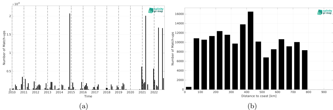
Figure 2: Number of match-ups between TSG (Polarstern) and CCI SSS L4 Merged-OI v4.41 - 30-day running (ESA) SSS as a function of time (a) and as function of the distance to coast (b) over the SMOS coastal zone (<800km) 60N-60S Pi-MEP region and for the full satellite product period.
