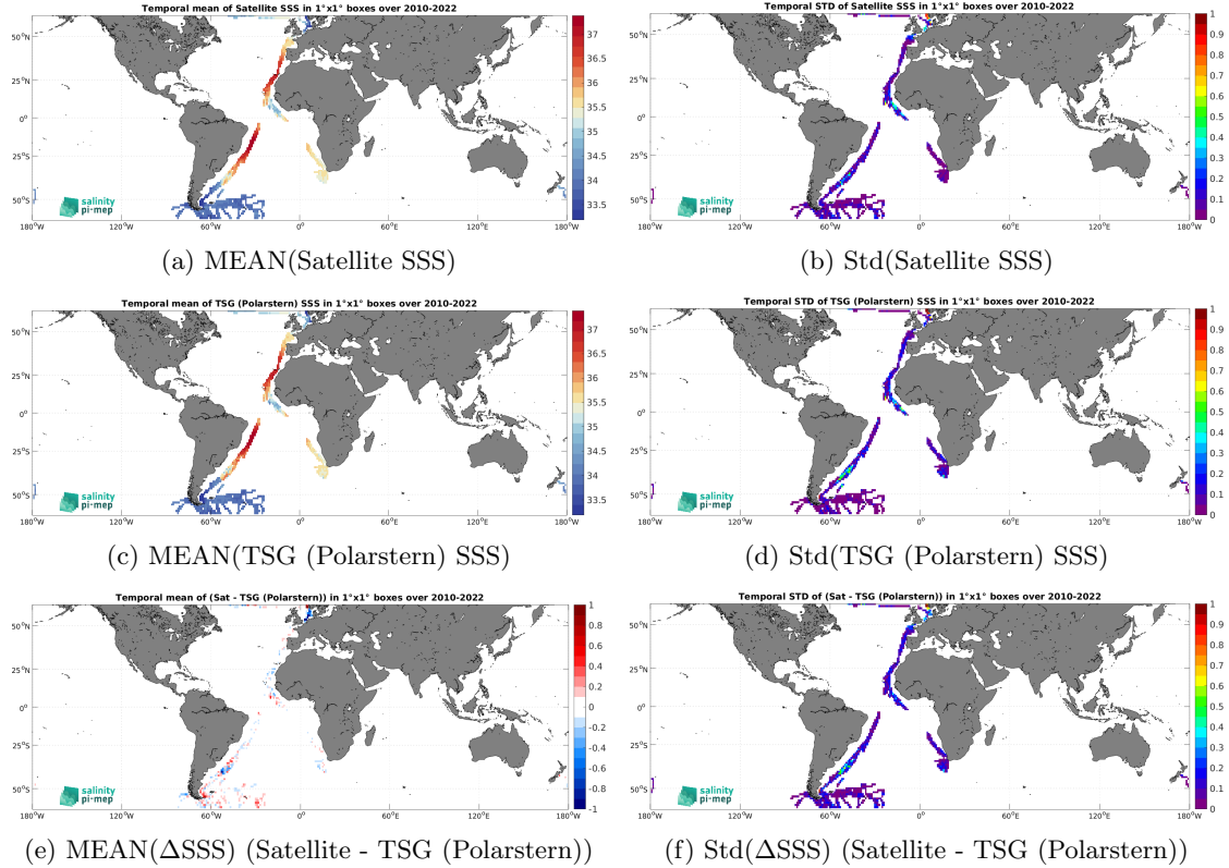
Figure 7: Temporal mean (left) and Std (right) of SSS from CCI SSS L4 Merged-OI v4.41 - 30-day running (ESA) (top), TSG (Polarstern) (middle), and of \Delta SSS (Satellite - TSG (Polarstern)). Only match-up pairs are used to generate these maps.
