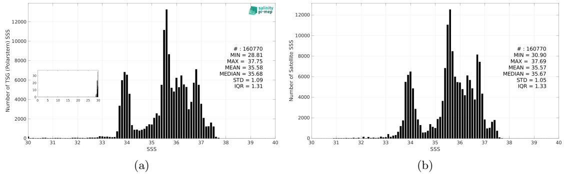
Figure 3: Histograms of SSS from TSG (Polarstern) (a) and CCI SSS L4 Merged-OI v4.41 - 30-day running (ESA) (b) considering all match-up pairs per bins of 0.1 over the SMOS coastal zone (<800km) 60N-60S Pi-MEP region and for the full satellite product period.
