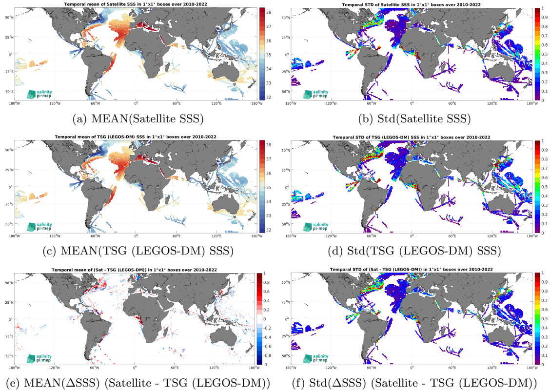
Figure 7: Temporal mean (left) and Std (right) of SSS from CCI SSS L4 Merged-OI v4.41 - 30-day running (ESA) (top), TSG (LEGOS-DM) (middle), and of \Delta SSS (Satellite - TSG (LEGOS-DM)). Only match-up pairs are used to generate these maps.
