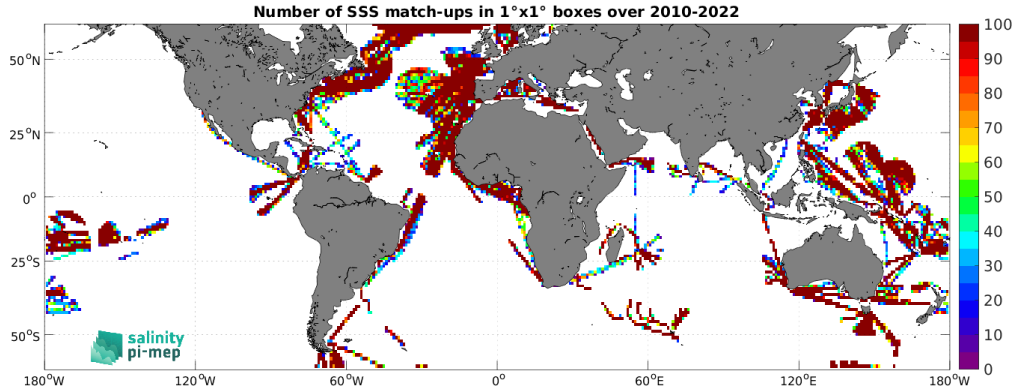
Figure 5: Number of SSS match-ups between TSG (LEGOS-DM) SSS and the CCI SSS L4 Merged-OI v4.41 - 30-day running (ESA) SSS product for the SMOS coastal zone (<800km) 60N-60S Pi-MEP region over 1^{\circ} \times 1^{\circ} boxes and for the full satellite product period.
