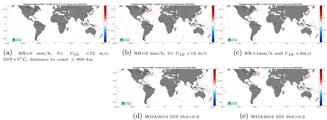
Figure 14: Temporal mean gridded over spatial boxes of size 1^\circ \times 1^\circ of \Delta SSS (CCI SSS L4 Merged-OI v4.41 - 30-day running (ESA) - TSG (LEGOS-DM)) for 5 different subdatasets corresponding to:RR=0 mm/h, 3 < U_{10} < 12 m/s, SST >5^\circ\text{C} , distance to coast > 800 km (a), RR=0 mm/h, 3 < U_{10} < 12 m/s (b), RR >1 mm/h and U_{10} < 4 m/s (c), WOA2013 SSS Std <0.2 (d), WOA2013 SSS Std >0.2 (e).
