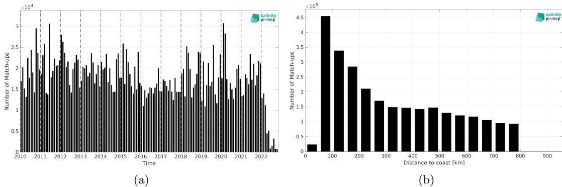
Figure 2: Number of match-ups between TSG (LEGOS-DM) and CCI SSS L4 Merged-OI v4.41 - 30-day running (ESA) SSS as a function of time (a) and as function of the distance to coast (b) over the SMOS coastal zone (<800km) 60N-60S Pi-MEP region and for the full satellite product period.
