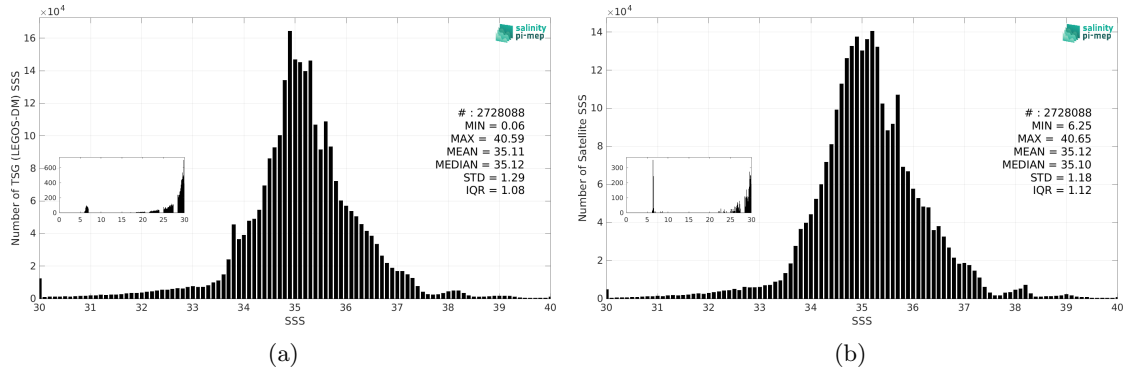
Figure 3: Histograms of SSS from TSG (LEGOS-DM) (a) and CCI SSS L4 Merged-OI v4.41 - 30-day running (ESA) (b) considering all match-up pairs per bins of 0.1 over the SMOS coastal zone (<800km) 60N-60S Pi-MEP region and for the full satellite product period.
