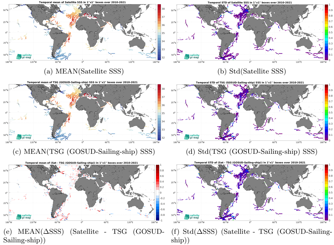
Figure 7: Temporal mean (left) and Std (right) of SSS from CCI SSS L4 Merged-OI v4.41 - 30-day running (ESA) (top), TSG (GOSUD-Sailing-ship) (middle), and of \Delta\text{SSS} (Satellite - TSG (GOSUD-Sailing-ship)). Only match-up pairs are used to generate these maps.
