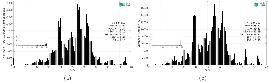
Figure 3: Histograms of SSS from TSG (GOSUD-Sailing-ship) (a) and CCI SSS L4 Merged-OI v4.41 - 30-day running (ESA) (b) considering all match-up pairs per bins of 0.1 over the SMOS coastal zone (<800km) 60N-60S Pi-MEP region and for the full satellite product period.
