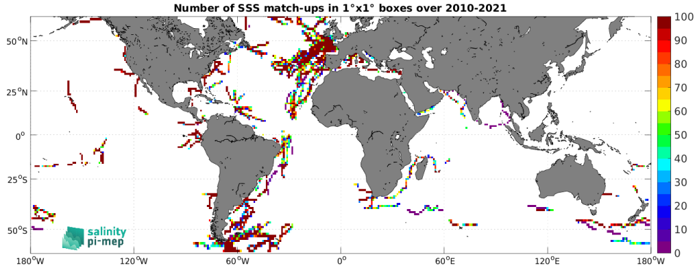
Figure 5: Number of SSS match-ups between TSG (GOSUD-Sailing-ship) SSS and the CCI SSS L4 Merged-OI v4.41 - 30-day running (ESA) SSS product for the SMOS coastal zone ( <800\text{km} ) 60N-60S Pi-MEP region over 1^\circ \times 1^\circ boxes and for the full satellite product period.
