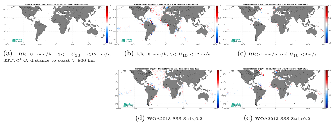
Figure 14: Temporal mean gridded over spatial boxes of size 1^\circ \times 1^\circ of \Delta\text{SSS} (CCI SSS L4 Merged-OI v4.41 - 30-day running (ESA) - TSG (GOSUD-Research-vessel)) for 5 different subdatasets corresponding to:RR=0 mm/h, 3 < U_{10} < 12 m/s, SST > 5^\circ\text{C} , distance to coast > 800 km (a), RR=0 mm/h, 3 < U_{10} < 12 m/s (b), RR > 1 mm/h and U_{10} < 4 m/s (c), WOA2013 SSS Std < 0.2 (d), WOA2013 SSS Std > 0.2 (e).
