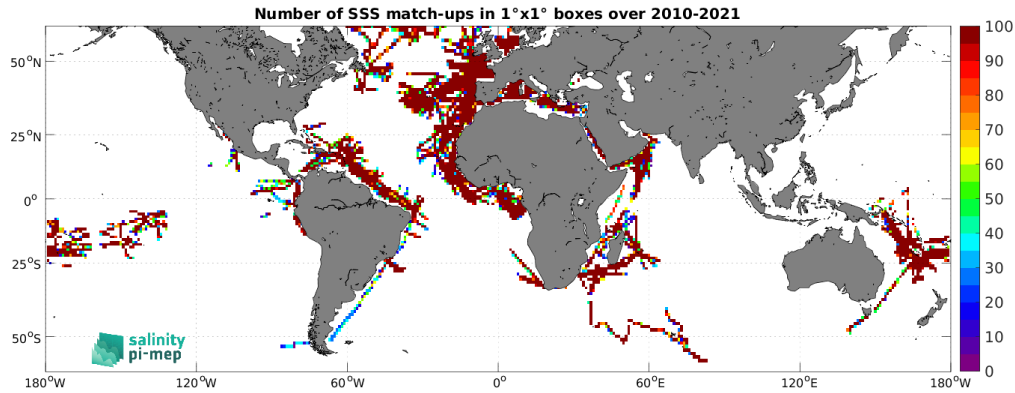
Figure 5: Number of SSS match-ups between TSG (GOSUD-Research-vessel) SSS and the CCI SSS L4 Merged-OI v4.41 - 30-day running (ESA) SSS product for the SMOS coastal zone (<800km) 60N-60S Pi-MEP region over 1^\circ \times 1^\circ boxes and for the full satellite product period.
