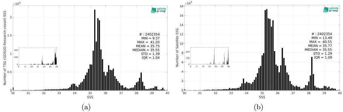
Figure 3: Histograms of SSS from TSG (GOSUD-Research-vessel) (a) and CCI SSS L4 Merged-OI v4.41 - 30-day running (ESA) (b) considering all match-up pairs per bins of 0.1 over the SMOS coastal zone (<800km) 60N-60S Pi-MEP region and for the full satellite product period.
