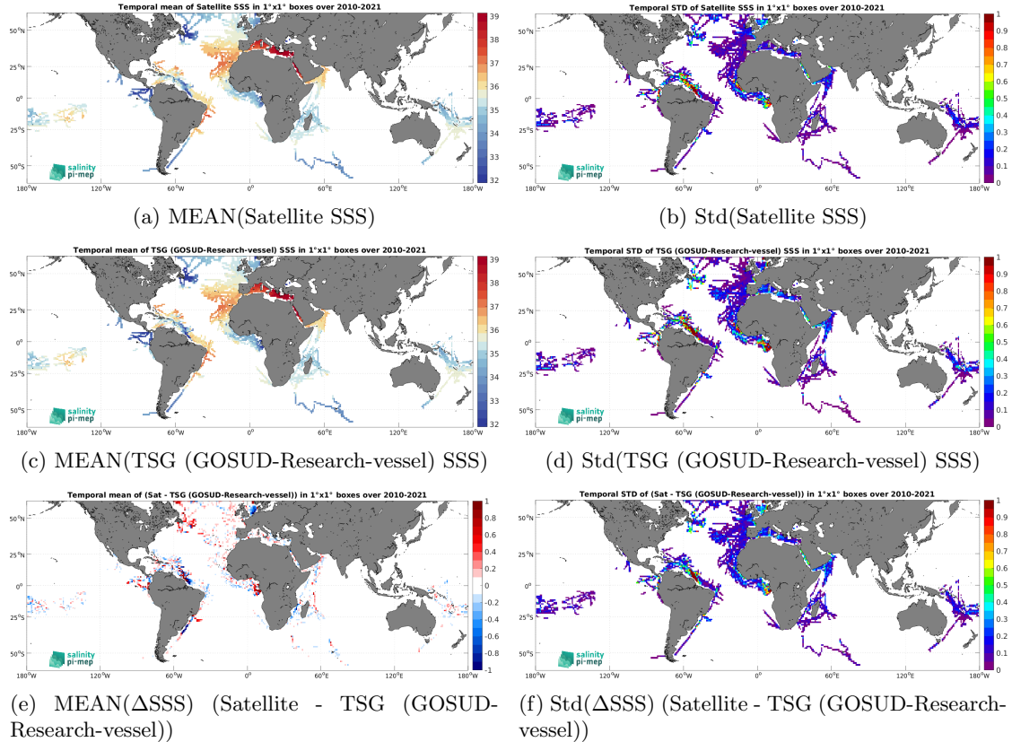
Figure 7: Temporal mean (left) and Std (right) of SSS from CCI SSS L4 Merged-OI v4.41 - 30-day running (ESA) (top), TSG (GOSUD-Research-vessel) (middle), and of \Delta\text{SSS} (Satellite - TSG (GOSUD-Research-vessel)). Only match-up pairs are used to generate these maps.
