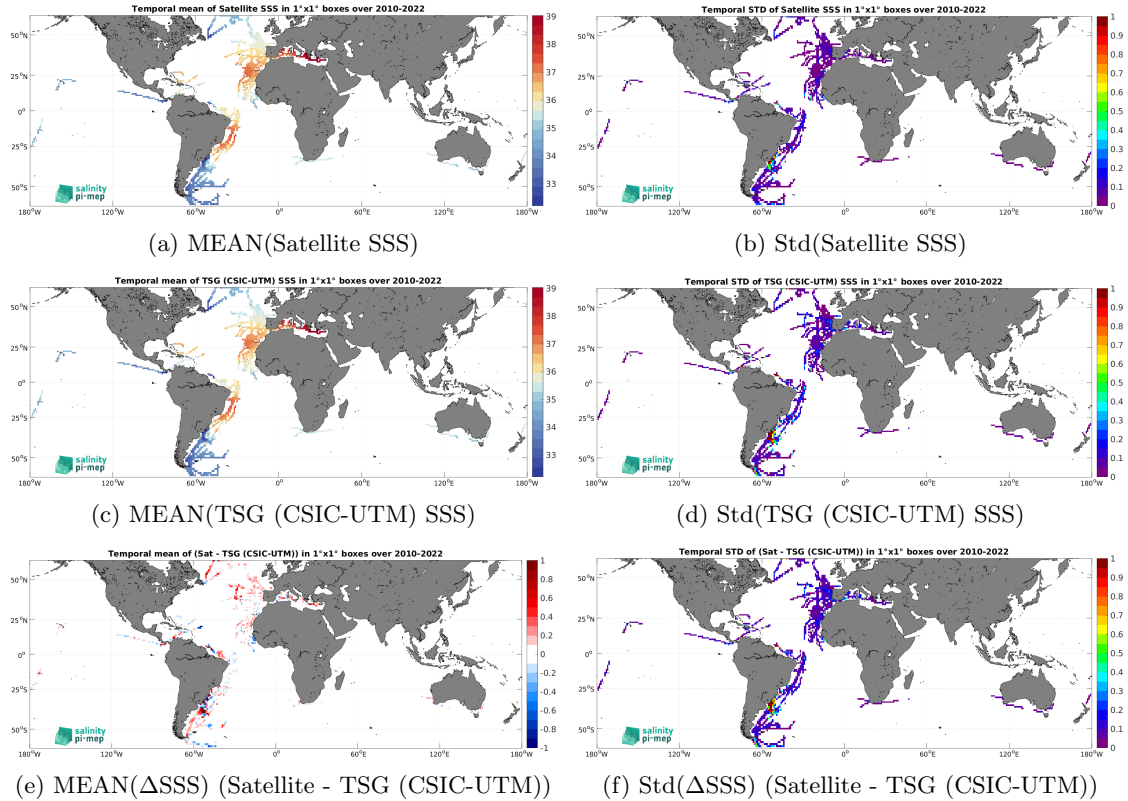
Figure 7: Temporal mean (left) and Std (right) of SSS from CCI SSS L4 Merged-OI v4.41 - 30-day running (ESA) (top), TSG (CSIC-UTM) ( in situ ) dataset (middle), and of \Delta\text{SSS} (Satellite - TSG (CSIC-UTM)). Only match-up pairs are used to generate these maps.
