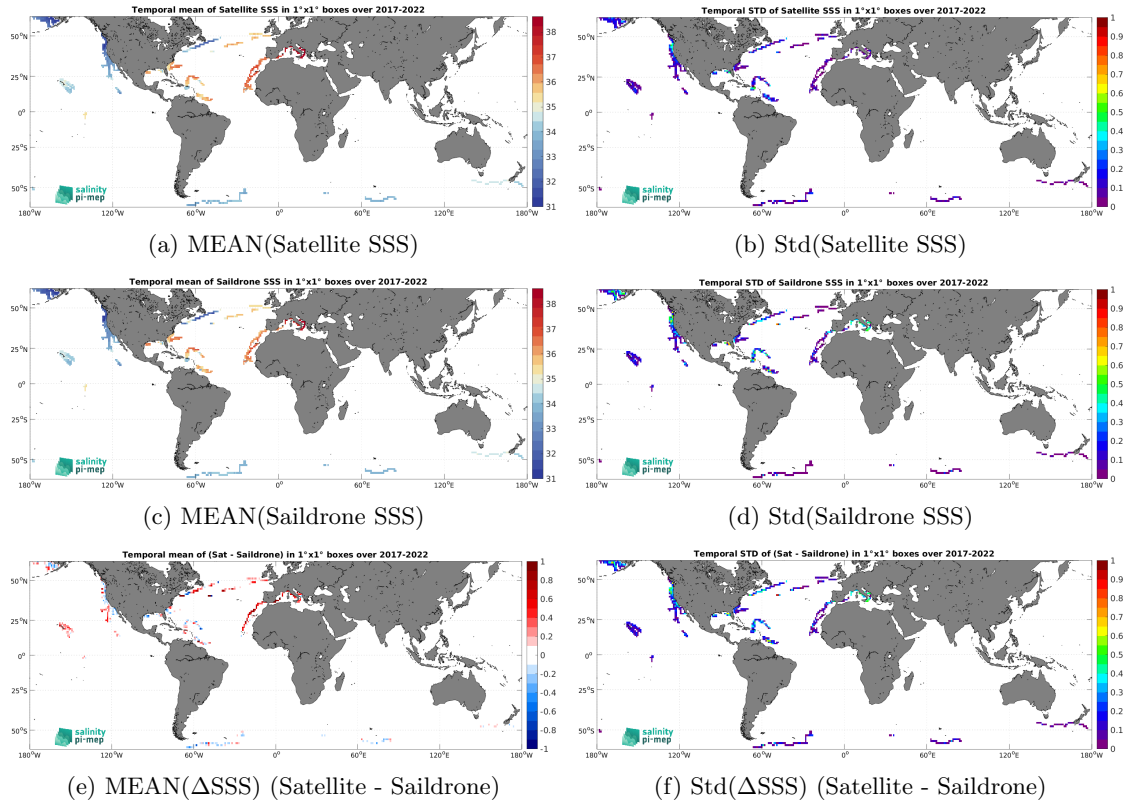
Figure 7: Temporal mean (left) and Std (right) of SSS from CCI SSS L4 Merged-OI v4.41 - 30-day running (ESA) (top), Saildrone (middle), and of \Delta SSS (Satellite - Saildrone). Only match-up pairs are used to generate these maps.
