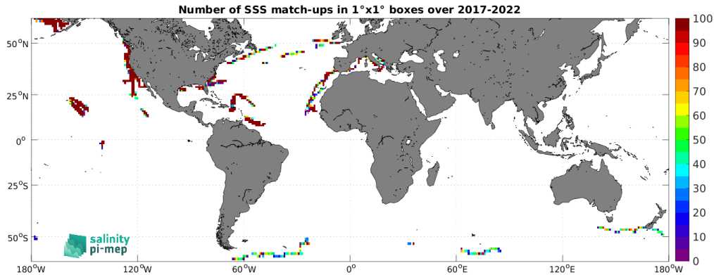
Figure 5: Number of SSS match-ups between Saildrone SSS and the CCI SSS L4 Merged-OI v4.41 - 30-day running (ESA) SSS product for the SMOS coastal zone (<800km) 60N-60S Pi-MEP region over 1^\circ \times 1^\circ boxes and for the full satellite product period.
