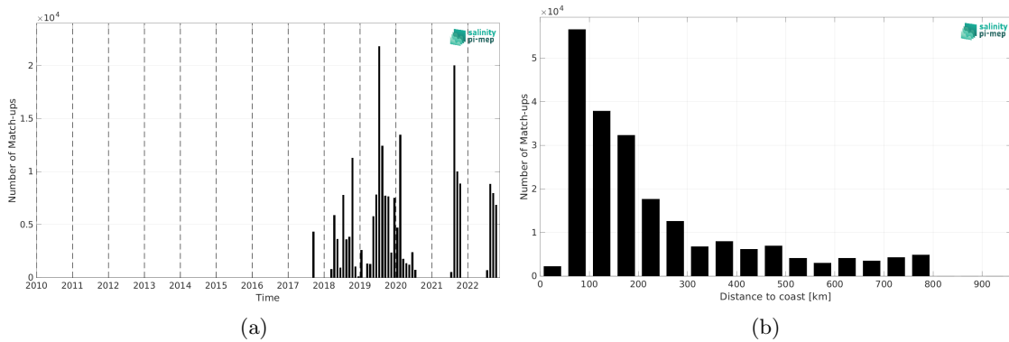
Figure 2: Number of match-ups between Saildrone and CCI SSS L4 Merged-OI v4.41 - 30-day running (ESA) SSS as a function of time (a) and as function of the distance to coast (b) over the SMOS coastal zone (<800km) 60N-60S Pi-MEP region and for the full satellite product period.
