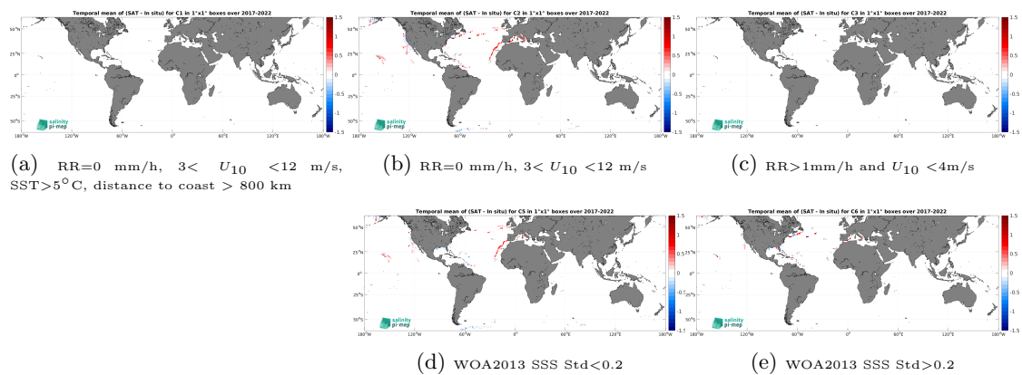
Figure 14: Temporal mean gridded over spatial boxes of size 1^\circ \times 1^\circ of \Delta SSS (CCI SSS L4 Merged-OI v4.41 - 30-day running (ESA) - Saildrone) for 5 different subdatasets corresponding to:RR=0 mm/h, 3 < U_{10} < 12 m/s, SST >5^\circ C, distance to coast > 800 km (a), RR=0 mm/h, 3 < U_{10} < 12 m/s (b), RR >1 mm/h and U_{10} < 4 m/s (c), WOA2013 SSS Std <0.2 (d), WOA2013 SSS Std >0.2 (e).
