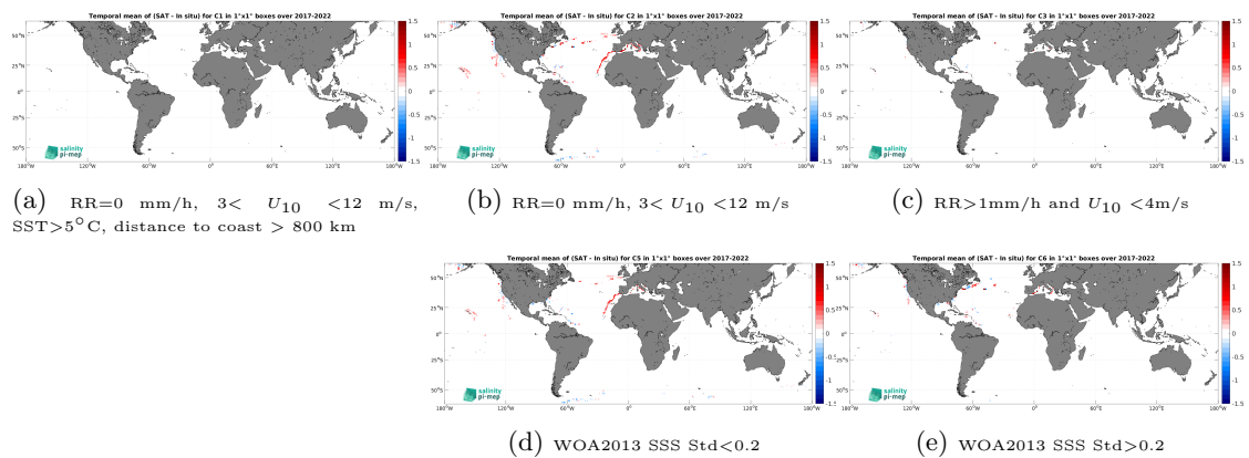
Figure 14: Temporal mean gridded over spatial boxes of size 1^\circ \times 1^\circ of \Delta\text{SSS} (CCI SSS L4 Merged-OI v4.41 - 30-day running (ESA) - Saildrone) for 5 different subdatasets corresponding to:RR=0 mm/h, 3 < U_{10} < 12 m/s, SST >5^\circ\text{C} , distance to coast > 800 km (a), RR=0 mm/h, 3 < U_{10} < 12 m/s (b), RR >1 mm/h and U_{10} < 4 m/s (c), WOA2013 SSS Std <0.2 (d), WOA2013 SSS Std >0.2 (e).
