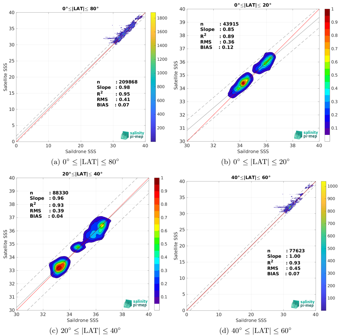
Figure 10: Contour maps of the concentration of CCI SSS L4 Merged-OI v4.41 - 30-day running (ESA) SSS (y-axis) versus Ssaldrone SSS (x-axis) at match-up pairs for different latitude bands. For each plot, the red line shows x=y . The black thin and dashed lines indicate a linear fit through the data cloud and the \pm 95\% confidence levels, respectively. The number match-up pairs n , the slope and R^2 coefficient of the linear fit, the root mean square (RMS) and the mean bias between satellite and in situ data are indicated for each latitude band in each plots.
