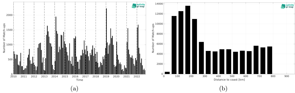
Figure 2: Number of match-ups between Marine mammals and CCI SSS L4 Merged-OI v4.41 - 30-day running (ESA) SSS as a function of time (a) and as function of the distance to coast (b) over the SMOS coastal zone (<800km) 60N-60S Pi-MEP region and for the full satellite product period.
