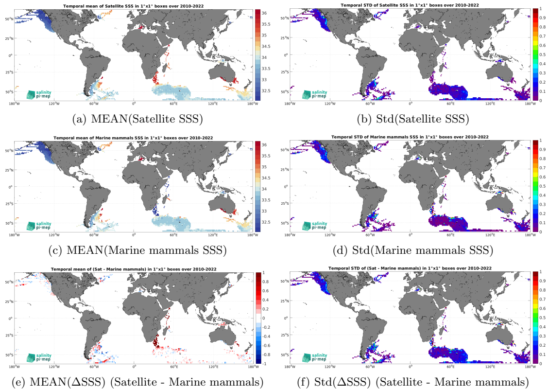
Figure 7: Temporal mean (left) and Std (right) of SSS from CCI SSS L4 Merged-OI v4.41 - 30-day running (ESA) (top), Marine mammals (middle), and of \Delta SSS (Satellite - Marine mammals). Only match-up pairs are used to generate these maps.
