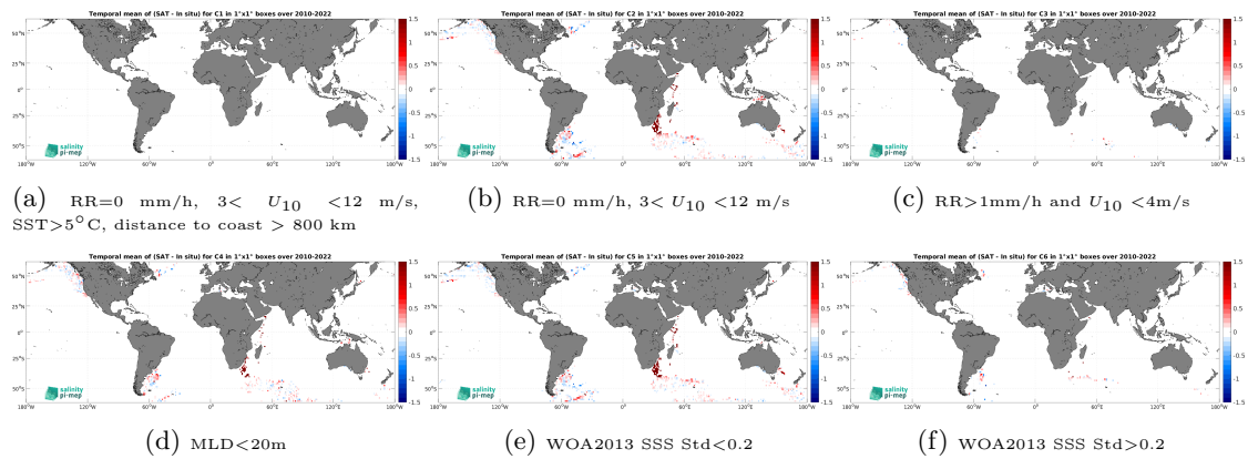
Figure 14: Temporal mean gridded over spatial boxes of size 1^\circ \times 1^\circ of \Delta SSS (CCI SSS L4 Merged-OI v4.41 - 30-day running (ESA) - Marine mammals) for 6 different subdatasets corresponding to:RR=0 mm/h, 3 < U_{10} < 12 m/s, SST >5^\circ C, distance to coast > 800 km (a), RR=0 mm/h, 3 < U_{10} < 12 m/s (b), RR >1 mm/h and U_{10} < 4 m/s (c),MLD <20 m (d),WOA2013 SSS Std <0.2 (e),WOA2013 SSS Std >0.2 (f).
