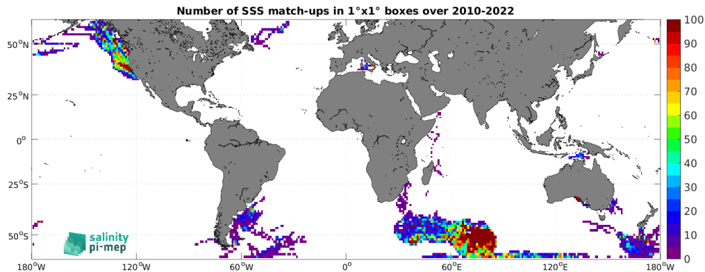
Figure 5: Number of SSS match-ups between Marine mammals SSS and the CCI SSS L4 Merged-OI v4.41 - 30-day running (ESA) SSS product for the SMOS coastal zone (<800km) 60N-60S Pi-MEP region over 1^\circ \times 1^\circ boxes and for the full satellite product period.
