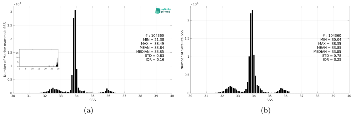
Figure 3: Histograms of SSS from Marine mammals (a) and CCI SSS L4 Merged-OI v4.41 - 30-day running (ESA) (b) considering all match-up pairs per bins of 0.1 over the SMOS coastal zone (<800km) 60N-60S Pi-MEP region and for the full satellite product period.
