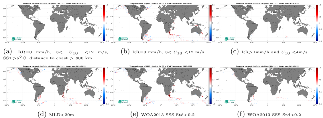
Figure 14: Temporal mean gridded over spatial boxes of size 1^\circ \times 1^\circ of \Delta\text{SSS} (CCI SSS L4 Merged-OI v4.41 - 30-day running (ESA) - Marine mammals) for 6 different subdatasets corresponding to:RR=0 mm/h, 3 < U_{10} < 12 m/s, SST>5°C, distance to coast > 800 km (a), RR=0 mm/h, 3 < U_{10} < 12 m/s (b), RR>1mm/h and U_{10} < 4 m/s (c),MLD<20m (d),WOA2013 SSS Std<0.2 (e),WOA2013 SSS Std>0.2 (f).
