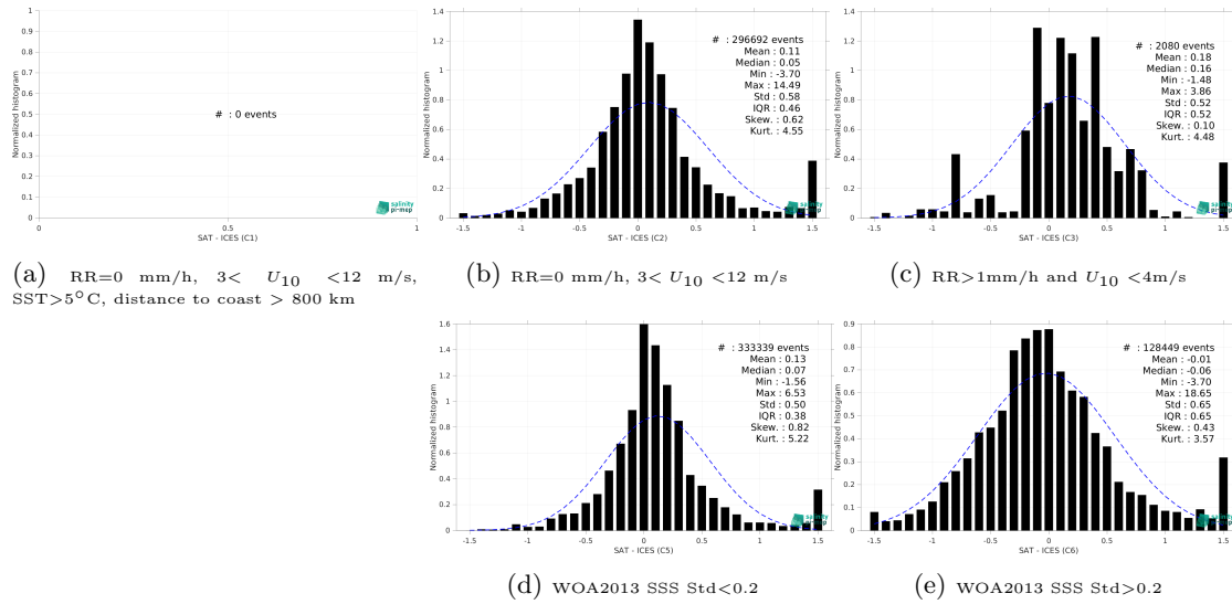
Figure 15: Normalized histogram of \Delta SSS (CCI SSS L4 Merged-OI v4.41 - 30-day running (ESA) - ICES) for 5 different subdatasets corresponding to: RR=0 mm/h, 3 < U_{10} < 12 m/s, SST > 5°C, distance to coast > 800 km (a), RR=0 mm/h, 3 < U_{10} < 12 m/s (b), RR > 1mm/h and U_{10} < 4 m/s (c), WOA2013 SSS Std < 0.2 (d), WOA2013 SSS Std > 0.2 (e).
