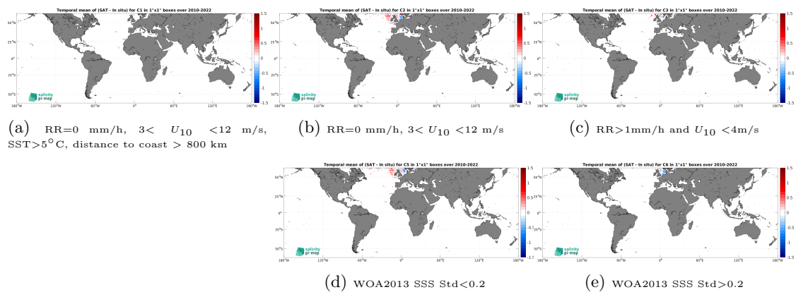
Figure 14: Temporal mean gridded over spatial boxes of size 1^\circ \times 1^\circ of \Delta SSS (CCI SSS L4 Merged-OI v4.41 - 30-day running (ESA) - ICES) for 5 different subdatasets corresponding to:RR=0 mm/h, 3 < U_{10} < 12 m/s, SST >5^\circ C, distance to coast > 800 km (a), RR=0 mm/h, 3 < U_{10} < 12 m/s (b), RR >1 mm/h and U_{10} < 4 m/s (c), WOA2013 SSS Std <0.2 (d), WOA2013 SSS Std >0.2 (e).
