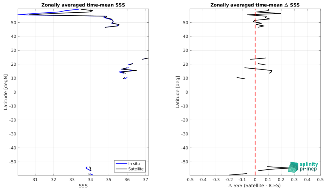
Figure 9: Left panel: Zonal mean SSS from CCI SSS L4 Merged-OI v4.41 - 30-day running (ESA) satellite product (black) and from ICES (blue). Right panel: Zonal mean of \Delta SSS (Satellite - ICES) for all the collected Pi-MEP match-up pairs estimated over the full satellite product period.
