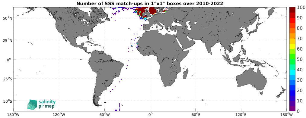
Figure 5: Number of SSS match-ups between ICES SSS and the CCI SSS L4 Merged-OI v4.41 - 30-day running (ESA) SSS product for the SMOS coastal zone (<800km) 60N-60S Pi-MEP region over 1^\circ \times 1^\circ boxes and for the full satellite product period.
