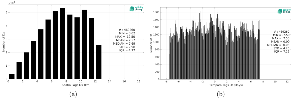
Figure 6: Histograms of the spatial (a) and temporal (b) lags between the location/time of the ICES measurement and the date of the corresponding CCI SSS L4 Merged-OI v4.41 - 30-day running (ESA) SSS pixel.
