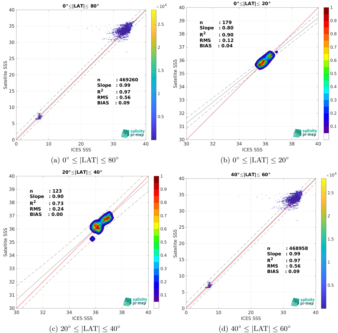
Figure 10: Contour maps of the concentration of CCI SSS L4 Merged-OI v4.41 - 30-day running (ESA) SSS (y-axis) versus ICES SSS (x-axis) at match-up pairs for different latitude bands. For each plot, the red line shows x=y . The black thin and dashed lines indicate a linear fit through the data cloud and the \pm 95\% confidence levels, respectively. The number match-up pairs n , the slope and R^2 coefficient of the linear fit, the root mean square (RMS) and the mean bias between satellite and in situ data are indicated for each latitude band in each plots.
