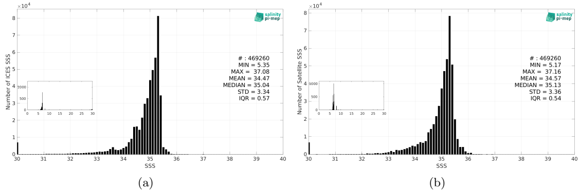
Figure 3: Histograms of SSS from ICES (a) and CCI SSS L4 Merged-OI v4.41 - 30-day running (ESA) (b) considering all match-up pairs per bins of 0.1 over the SMOS coastal zone (<800km) 60N-60S Pi-MEP region and for the full satellite product period.
