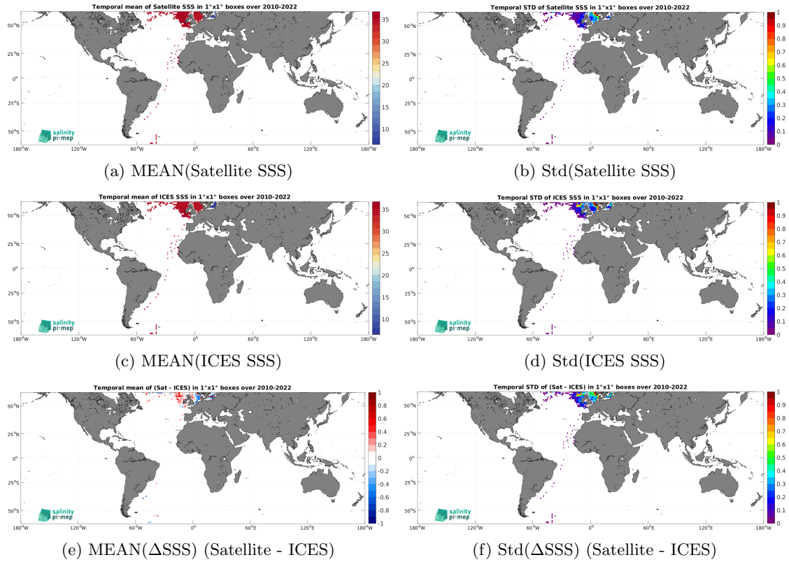
Figure 7: Temporal mean (left) and Std (right) of SSS from CCI SSS L4 Merged-OI v4.41 - 30-day running (ESA) (top), ICES (middle), and of \Delta SSS (Satellite - ICES). Only match-up pairs are used to generate these maps.
