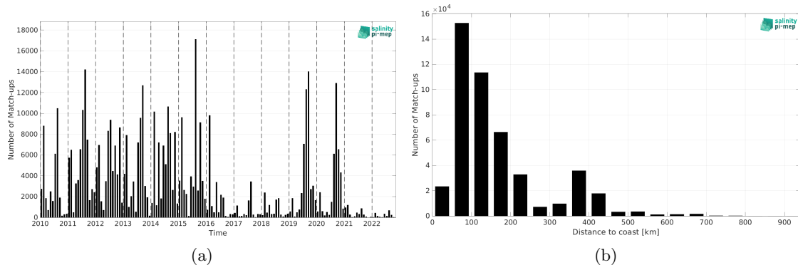
Figure 2: Number of match-ups between ICES and CCI SSS L4 Merged-OI v4.41 - 30-day running (ESA) SSS as a function of time (a) and as function of the distance to coast (b) over the SMOS coastal zone (<800km) 60N-60S Pi-MEP region and for the full satellite product period.
