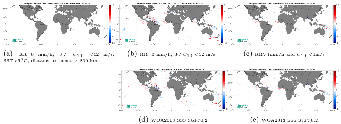
Figure 13: Temporal mean gridded over spatial boxes of size 1^\circ \times 1^\circ of \Delta SSS (CCI SSS L4 Merged-OI v4.41 - 30-day running (ESA) - Surface drifters) for 5 different subdatasets corresponding to:RR=0 mm/h, 3 < U_{10} < 12 m/s, SST >5^\circ C, distance to coast > 800 km (a), RR=0 mm/h, 3 < U_{10} < 12 m/s (b), RR >1 mm/h and U_{10} < 4 m/s (c), WOA2013 SSS Std <0.2 (d), WOA2013 SSS Std >0.2 (e).
