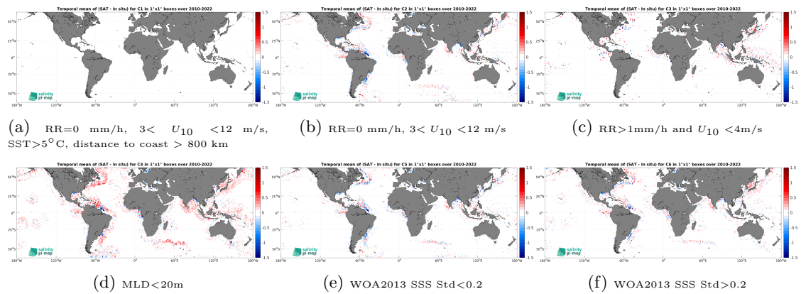
Figure 14: Temporal mean gridded over spatial boxes of size 1^\circ \times 1^\circ of \Delta SSS (CCI SSS L4 Merged-OI v4.41 - 30-day running (ESA) - Argo) for 6 different subdatasets corresponding to:RR=0 mm/h, 3 < U_{10} < 12 m/s, SST >5^\circ C, distance to coast > 800 km (a), RR=0 mm/h, 3 < U_{10} < 12 m/s (b), RR >1 mm/h and U_{10} < 4 m/s (c),MLD <20 m (d),WOA2013 SSS Std <0.2 (e),WOA2013 SSS Std >0.2 (f).
