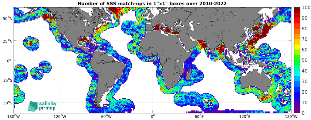
Figure 5: Number of SSS match-ups between Argo SSS and the CCI SSS L4 Merged-OI v4.41 - 30-day running (ESA) SSS product for the SMOS coastal zone (<800km) 60N-60S Pi-MEP region over 1^\circ \times 1^\circ boxes and for the full satellite product period.
