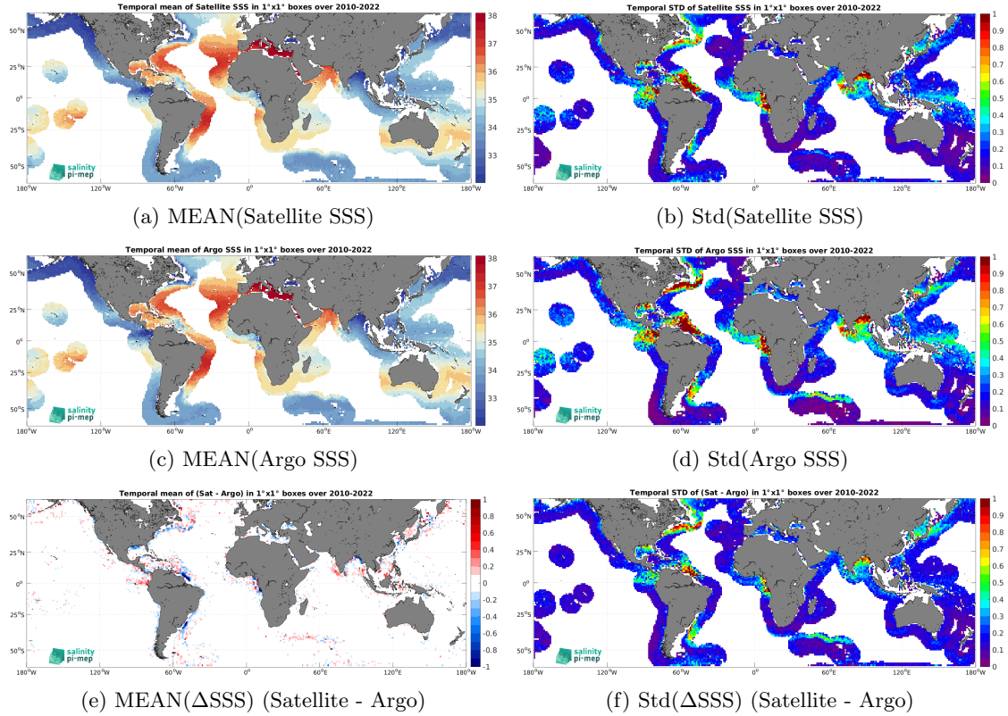
Figure 7: Temporal mean (left) and Std (right) of SSS from CCI SSS L4 Merged-OI v4.41 - 30-day running (ESA) (top), Argo (middle), and of \Delta SSS (Satellite - Argo). Only match-up pairs are used to generate these maps.
