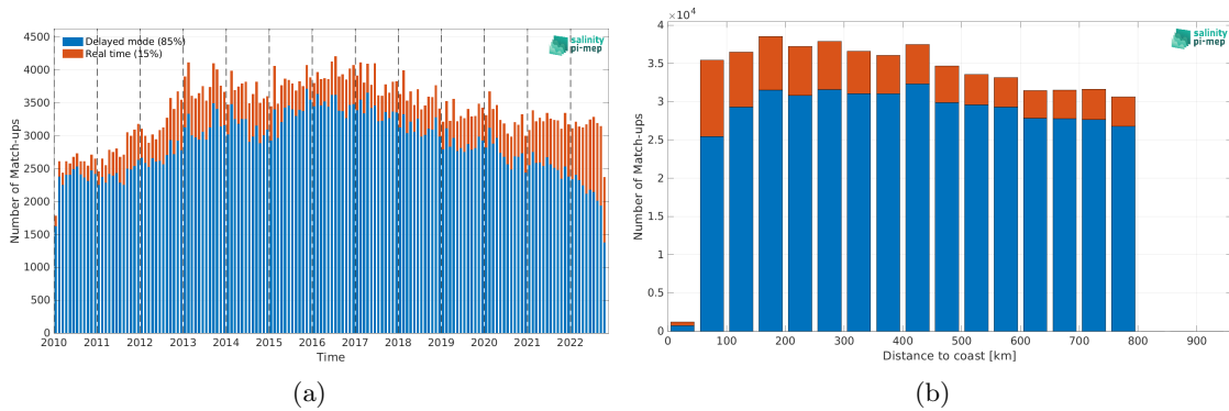
Figure 2: Number of match-ups between Argo and CCI SSS L4 Merged-OI v4.41 - 30-day running (ESA) SSS as a function of time (a) and as function of the distance to coast (b) over the SMOS coastal zone (<800km) 60N-60S Pi-MEP region and for the full satellite product period.
