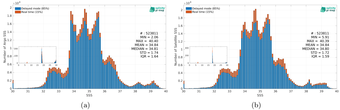
Figure 3: Histograms of SSS from Argo (a) and CCI SSS L4 Merged-OI v4.41 - 30-day running (ESA) (b) considering all match-up pairs per bins of 0.1 over the SMOS coastal zone (<800km) 60N-60S Pi-MEP region and for the full satellite product period.
