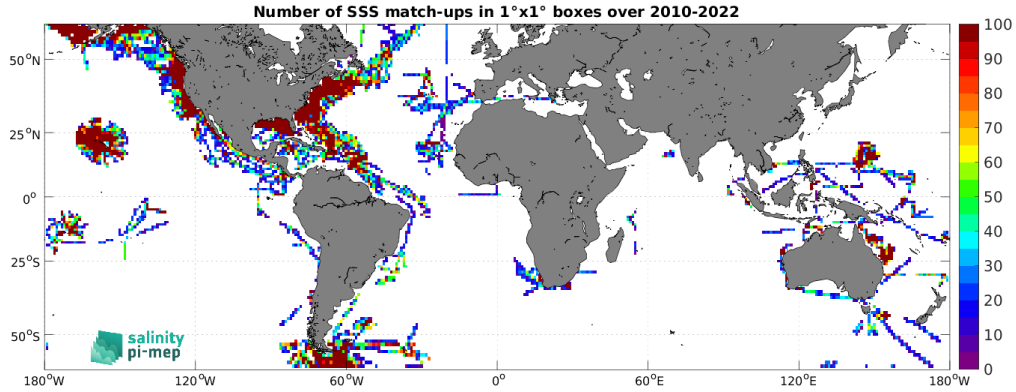
Figure 4: Number of SSS match-ups between TSG (SAMOS) SSS and the CCI SSS L4 Merged-OI v4.4 - 7-day running (ESA) SSS product for the SMOS coastal zone ( <800\text{km} ) 60N-60S Pi-MEP region over 1^\circ \times 1^\circ boxes and for the full satellite product period.
