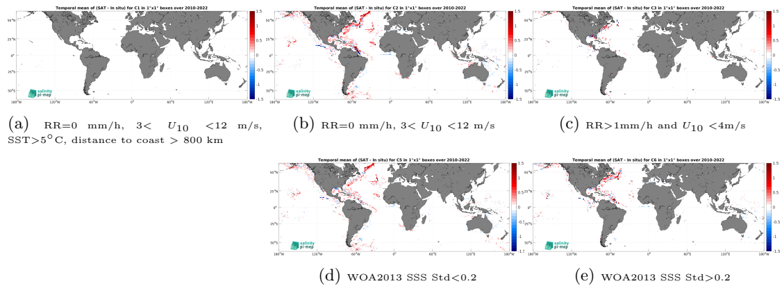
Figure 12: Temporal mean gridded over spatial boxes of size 1^\circ \times 1^\circ of \Delta SSS (CCI SSS L4 Merged-OI v4.4 - 7-day running (ESA) - TSG (SAMOS)) for 5 different subdatasets corresponding to:RR=0 mm/h, 3 < U_{10} < 12 m/s, SST >5^\circ\text{C} , distance to coast > 800 km (a), RR=0 mm/h, 3 < U_{10} < 12 m/s (b), RR >1 mm/h and U_{10} < 4 m/s (c), WOA2013 SSS Std <0.2 (d), WOA2013 SSS Std >0.2 (e).
