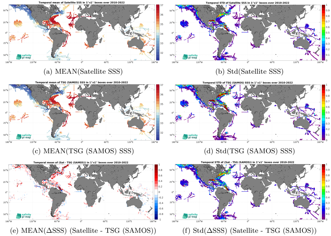
Figure 6: Temporal mean (left) and Std (right) of SSS from CCI SSS L4 Merged-OI v4.4 - 7-day running (ESA) (top), TSG (SAMOS) (middle), and of \Delta SSS (Satellite - TSG (SAMOS)). Only match-up pairs are used to generate these maps.
