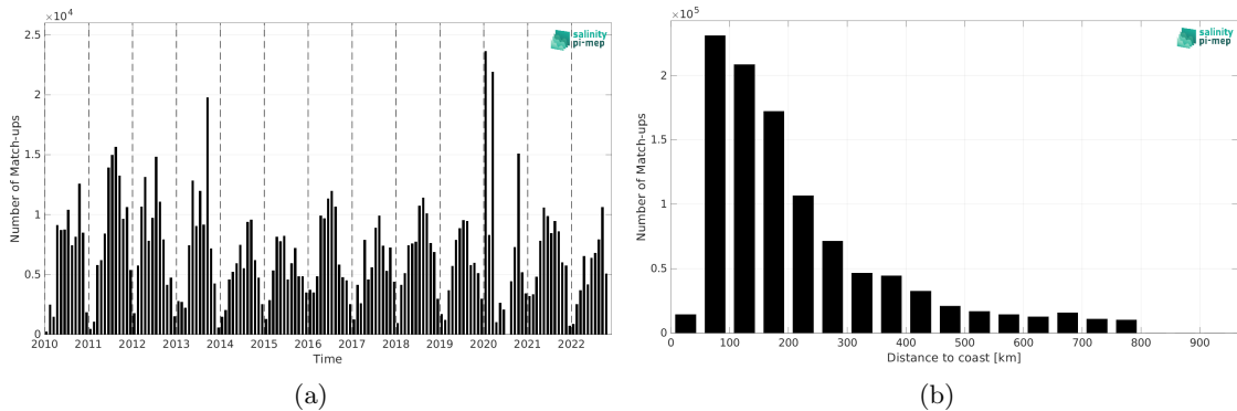
Figure 1: Number of match-ups between TSG (SAMOS) and CCI SSS L4 Merged-OI v4.4 - 7-day running (ESA) SSS as a function of time (a) and as function of the distance to coast (b) over the SMOS coastal zone (<800km) 60N-60S Pi-MEP region and for the full satellite product period.
