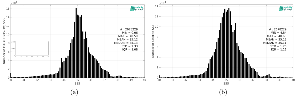
Figure 2: Histograms of SSS from TSG (LEGOS-DM) (a) and CCI SSS L4 Merged-OI v4.4 - 7-day running (ESA) (b) considering all match-up pairs per bins of 0.1 over the SMOS coastal zone (<800km) 60N-60S Pi-MEP region and for the full satellite product period.
