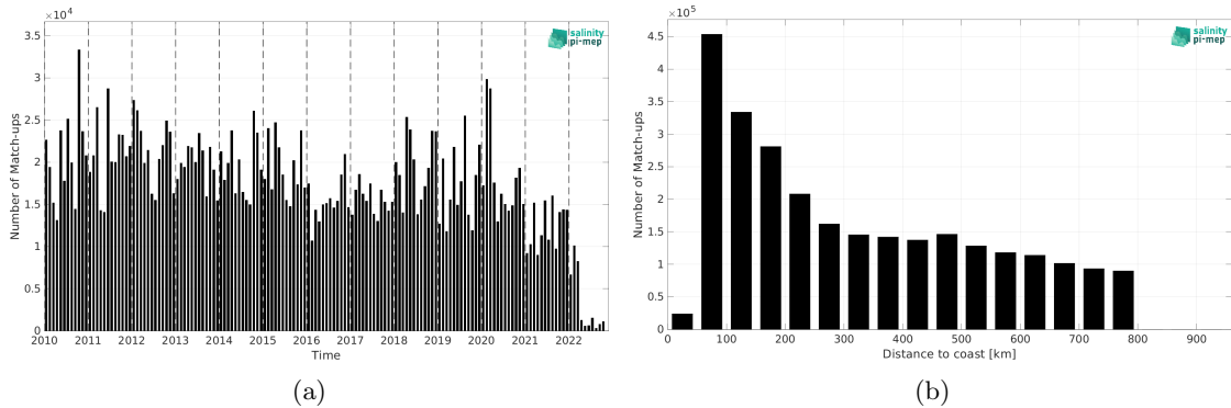
Figure 1: Number of match-ups between TSG (LEGOS-DM) and CCI SSS L4 Merged-OI v4.4 - 7-day running (ESA) SSS as a function of time (a) and as function of the distance to coast (b) over the SMOS coastal zone (<800km) 60N-60S Pi-MEP region and for the full satellite product period.
