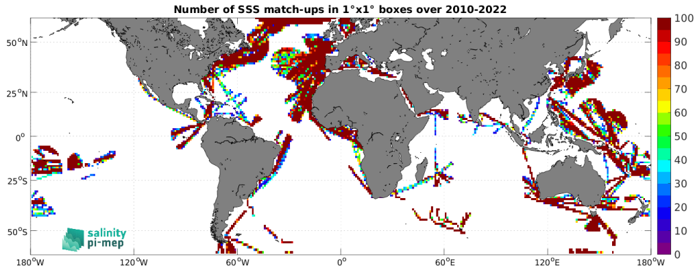
Figure 4: Number of SSS match-ups between TSG (LEGOS-DM) SSS and the CCI SSS L4 Merged-OI v4.4 - 7-day running (ESA) SSS product for the SMOS coastal zone (<800km) 60N-60S Pi-MEP region over 1^{\circ} \times 1^{\circ} boxes and for the full satellite product period.
