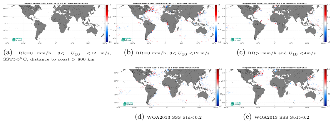
Figure 12: Temporal mean gridded over spatial boxes of size 1^\circ \times 1^\circ of \Delta SSS (CCI SSS L4 Merged-OI v4.4 - 7-day running (ESA) - TSG (LEGOS-DM)) for 5 different subdatasets corresponding to:RR=0 mm/h, 3 < U_{10} < 12 m/s, SST >5^\circ C, distance to coast > 800 km (a), RR=0 mm/h, 3 < U_{10} < 12 m/s (b), RR >1 mm/h and U_{10} < 4 m/s (c), WOA2013 SSS Std <0.2 (d), WOA2013 SSS Std >0.2 (e).
