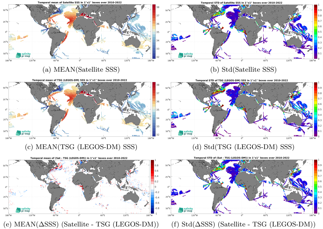
Figure 6: Temporal mean (left) and Std (right) of SSS from CCI SSS L4 Merged-OI v4.4 - 7-day running (ESA) (top), TSG (LEGOS-DM) (middle), and of \Delta SSS (Satellite - TSG (LEGOS-DM)). Only match-up pairs are used to generate these maps.
