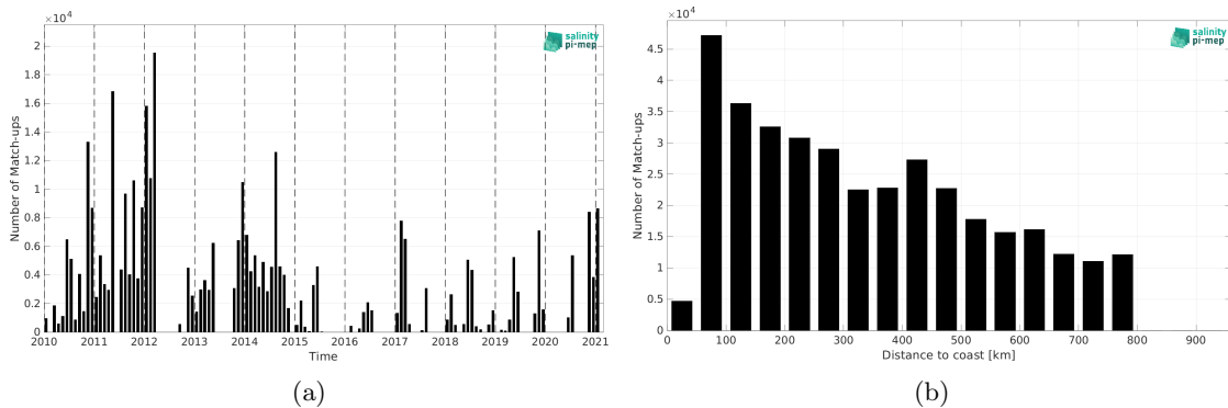
Figure 1: Number of match-ups between TSG (GOSUD-Sailing-ship) and CCI SSS L4 Merged-OI v4.4 - 7-day running (ESA) SSS as a function of time (a) and as function of the distance to coast (b) over the SMOS coastal zone (<800km) 60N-60S Pi-MEP region and for the full satellite product period.
