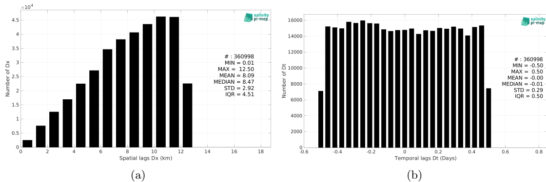
Figure 5: Histograms of the spatial (a) and temporal (b) lags between the location/time of the TSG (GOSUD-Sailing-ship) measurement and the date of the corresponding CCI SSS L4 Merged-OI v4.4 - 7-day running (ESA) SSS pixel.
