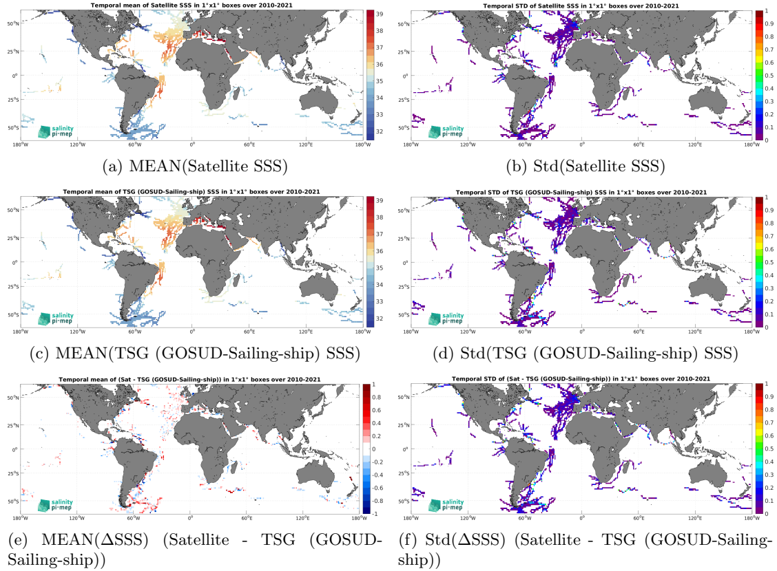
Figure 6: Temporal mean (left) and Std (right) of SSS from CCI SSS L4 Merged-OI v4.4 - 7-day running (ESA) (top), TSG (GOSUD-Sailing-ship) (middle), and of \Delta\text{SSS} (Satellite - TSG (GOSUD-Sailing-ship)). Only match-up pairs are used to generate these maps.
