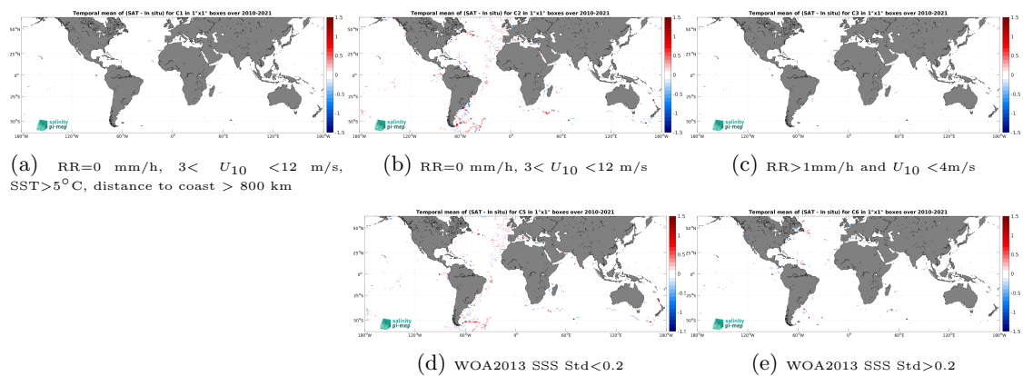
Figure 12: Temporal mean gridded over spatial boxes of size 1^\circ \times 1^\circ of \Delta SSS (CCI SSS L4 Merged-OI v4.4 - 7-day running (ESA) - TSG (GOSUD-Sailing-ship)) for 5 different subdatasets corresponding to: RR=0 mm/h, 3 < U_{10} < 12 m/s, SST > 5^\circ\text{C} , distance to coast > 800 km (a), RR=0 mm/h, 3 < U_{10} < 12 m/s (b), RR > 1 mm/h and U_{10} < 4 m/s (c), WOA2013 SSS Std < 0.2 (d), WOA2013 SSS Std > 0.2 (e).
