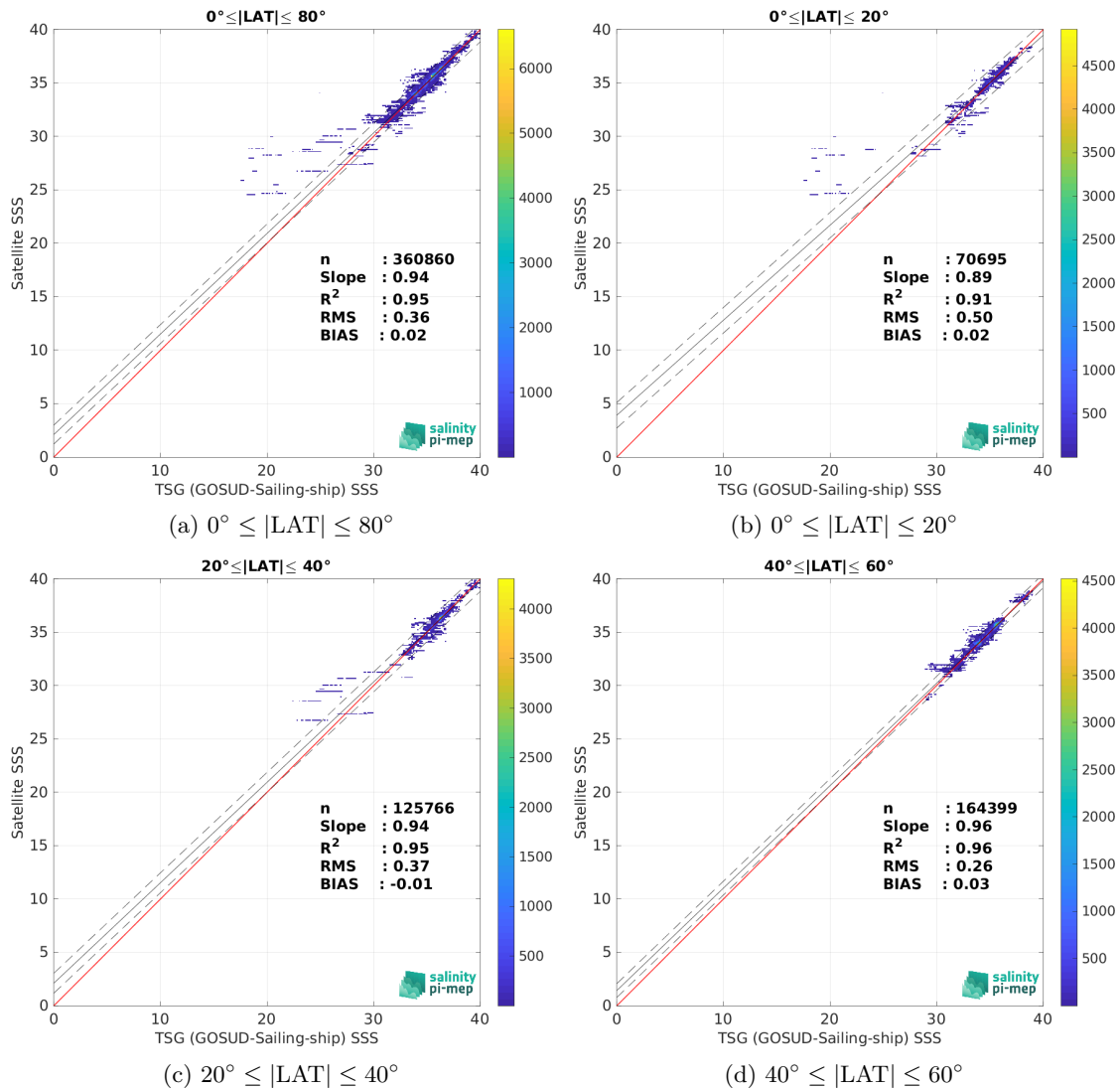
Figure 9: Contour maps of the concentration of CCI SSS L4 Merged-OI v4.4 - 7-day running (ESA) SSS (y-axis) versus TSG (GOSUD-Sailing-ship) SSS (x-axis) at match-up pairs for different latitude bands. For each plot, the red line shows x=y . The black thin and dashed lines indicate a linear fit through the data cloud and the \pm 95\% confidence levels, respectively. The number match-up pairs n , the slope and R^2 coefficient of the linear fit, the root mean square (RMS) and the mean bias between satellite and in situ data are indicated for each latitude band in each plots.
