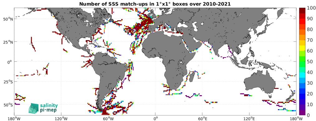
Figure 4: Number of SSS match-ups between TSG (GOSUD-Sailing-ship) SSS and the CCI SSS L4 Merged-OI v4.4 - 7-day running (ESA) SSS product for the SMOS coastal zone ( <800\text{km} ) 60N-60S Pi-MEP region over 1^\circ \times 1^\circ boxes and for the full satellite product period.
