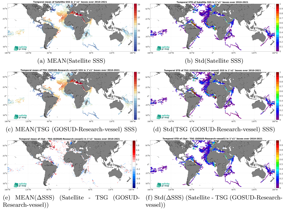
Figure 6: Temporal mean (left) and Std (right) of SSS from CCI SSS L4 Merged-OI v4.4 - 7-day running (ESA) (top), TSG (GOSUD-Research-vessel) (middle), and of \Delta\text{SSS} (Satellite - TSG (GOSUD-Research-vessel)). Only match-up pairs are used to generate these maps.
