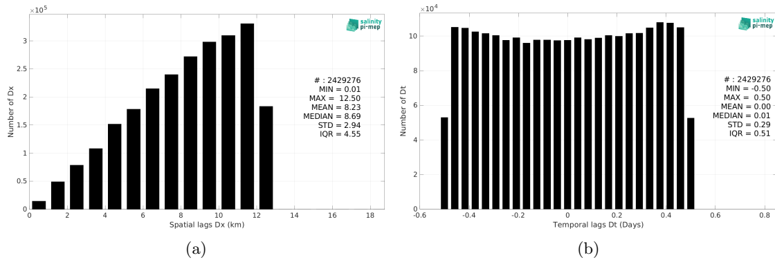
Figure 5: Histograms of the spatial (a) and temporal (b) lags between the location/time of the TSG (GOSUD-Research-vessel) measurement and the date of the corresponding CCI SSS L4 Merged-OI v4.4 - 7-day running (ESA) SSS pixel.
