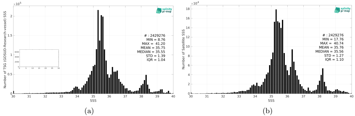
Figure 2: Histograms of SSS from TSG (GOSUD-Research-vessel) (a) and CCI SSS L4 Merged-OI v4.4 - 7-day running (ESA) (b) considering all match-up pairs per bins of 0.1 over the SMOS coastal zone (<800km) 60N-60S Pi-MEP region and for the full satellite product period.
