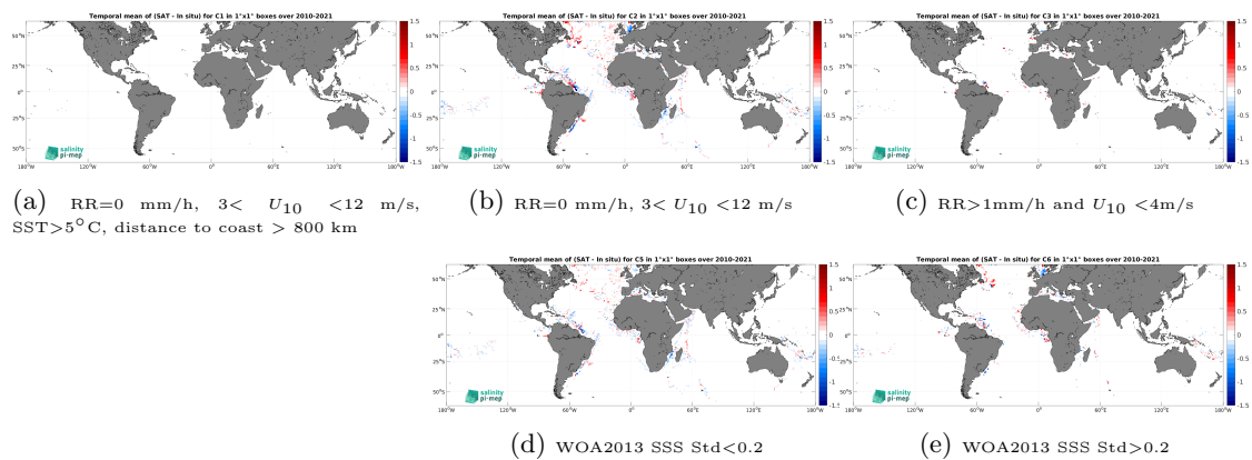
Figure 12: Temporal mean gridded over spatial boxes of size 1^\circ \times 1^\circ of \Delta SSS (CCI SSS L4 Merged-OI v4.4 - 7-day running (ESA) - TSG (GOSUD-Research-vessel)) for 5 different subdatasets corresponding to: RR=0 mm/h, 3 < U_{10} < 12 m/s, SST > 5^\circ\text{C} , distance to coast > 800 km (a), RR=0 mm/h, 3 < U_{10} < 12 m/s (b), RR > 1 mm/h and U_{10} < 4 m/s (c), WOA2013 SSS Std < 0.2 (d), WOA2013 SSS Std > 0.2 (e).
