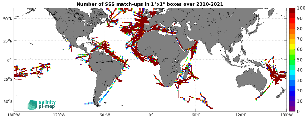
Figure 4: Number of SSS match-ups between TSG (GOSUD-Research-vessel) SSS and the CCI SSS L4 Merged-OI v4.4 - 7-day running (ESA) SSS product for the SMOS coastal zone ( <800\text{km} ) 60N-60S Pi-MEP region over 1^\circ \times 1^\circ boxes and for the full satellite product period.
