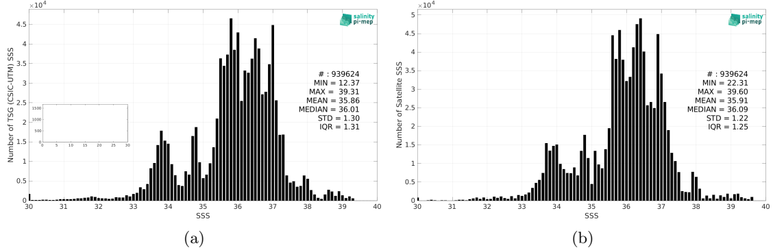
Figure 2: Histograms of SSS from TSG (CSIC-UTM) (a) and CCI SSS L4 Merged-OI v4.4 - 7-day running (ESA) (b) considering all match-up pairs per bins of 0.1 over the SMOS coastal zone (<800km) 60N-60S Pi-MEP region and for the full satellite product period.
