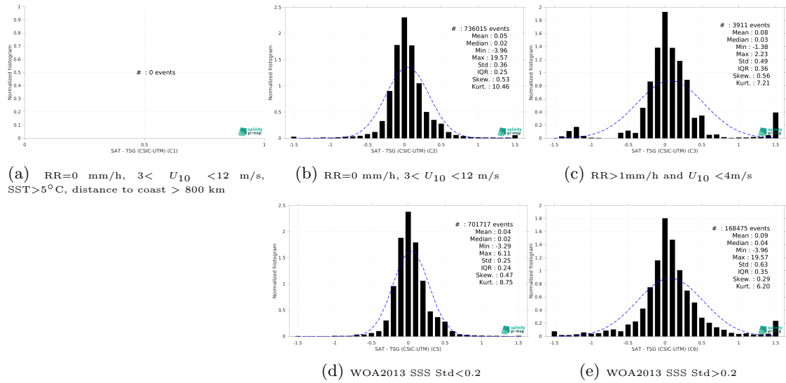
Figure 13: Normalized histogram of \Delta SSS (CCI SSS L4 Merged-OI v4.4 - 7-day running (ESA) - TSG (CSIC-UTM)) for 5 different subdatasets corresponding to: RR=0 mm/h, 3 < U_{10} < 12 m/s, SST>5°C, distance to coast > 800 km (a), RR=0 mm/h, 3 < U_{10} < 12 m/s (b), RR>1mm/h and U_{10} < 4 m/s (c), WOA2013 SSS Std<0.2 (d), WOA2013 SSS Std>0.2 (e).
