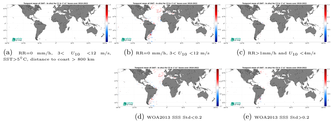
Figure 12: Temporal mean gridded over spatial boxes of size 1^\circ \times 1^\circ of \Delta\text{SSS} (CCI SSS L4 Merged-OI v4.4 - 7-day running (ESA) - TSG (CSIC-UTM)) for 5 different subdatasets corresponding to:RR=0 mm/h, 3 < U_{10} < 12 m/s, SST >5^\circ\text{C} , distance to coast > 800 km (a), RR=0 mm/h, 3 < U_{10} < 12 m/s (b), RR >1 mm/h and U_{10} < 4 m/s (c), WOA2013 SSS Std <0.2 (d), WOA2013 SSS Std >0.2 (e).
