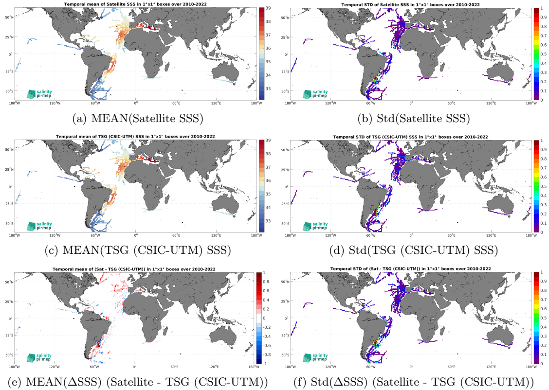
Figure 6: Temporal mean (left) and Std (right) of SSS from CCI SSS L4 Merged-OI v4.4 - 7-day running (ESA) (top), TSG (CSIC-UTM) (middle), and of \Delta SSS (Satellite - TSG (CSIC-UTM)). Only match-up pairs are used to generate these maps.
