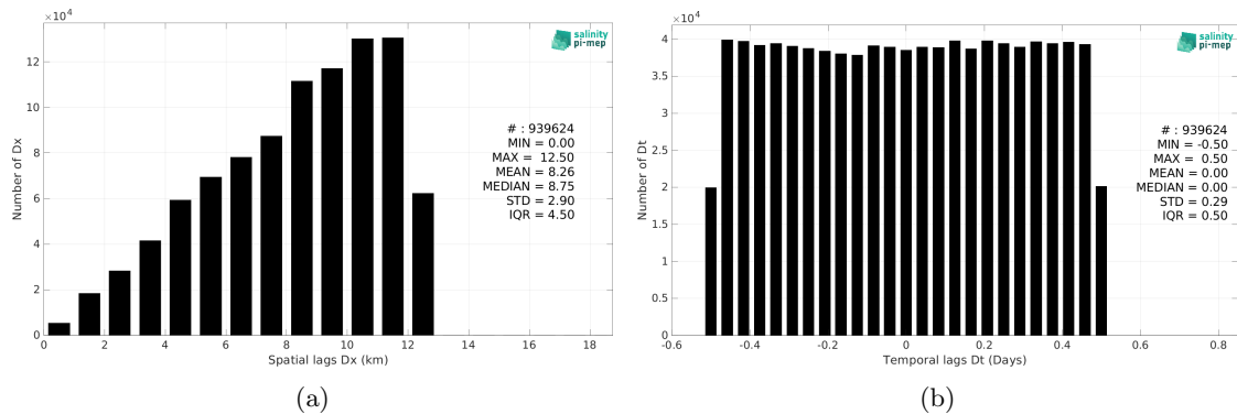
Figure 5: Histograms of the spatial (a) and temporal (b) lags between the location/time of the TSG (CSIC-UTM) measurement and the date of the corresponding CCI SSS L4 Merged-OI v4.4 - 7-day running (ESA) SSS pixel.
