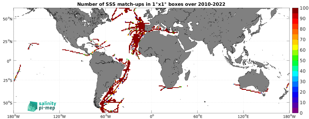
Figure 4: Number of SSS match-ups between TSG (CSIC-UTM) SSS and the CCI SSS L4 Merged-OI v4.4 - 7-day running (ESA) SSS product for the SMOS coastal zone (<800km) 60N-60S Pi-MEP region over 1^\circ \times 1^\circ boxes and for the full satellite product period.
