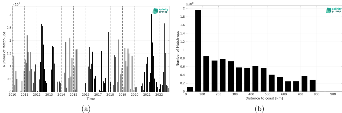
Figure 1: Number of match-ups between TSG (CSIC-UTM) and CCI SSS L4 Merged-OI v4.4 - 7-day running (ESA) SSS as a function of time (a) and as function of the distance to coast (b) over the SMOS coastal zone (<800km) 60N-60S Pi-MEP region and for the full satellite product period.
