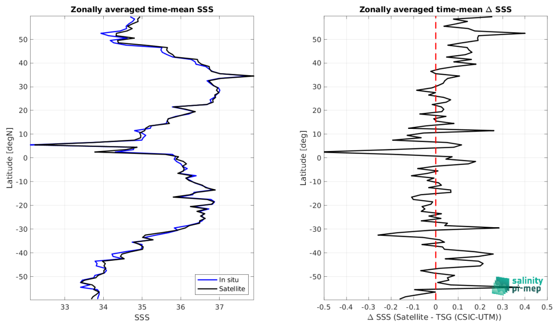
Figure 8: Left panel: Zonal mean SSS from CCI SSS L4 Merged-OI v4.4 - 7-day running (ESA) satellite product (black) and from TSG (CSIC-UTM) (blue). Right panel: Zonal mean of \Delta SSS (Satellite - TSG (CSIC-UTM)) for all the collected Pi-MEP match-up pairs estimated over the full satellite product period.
