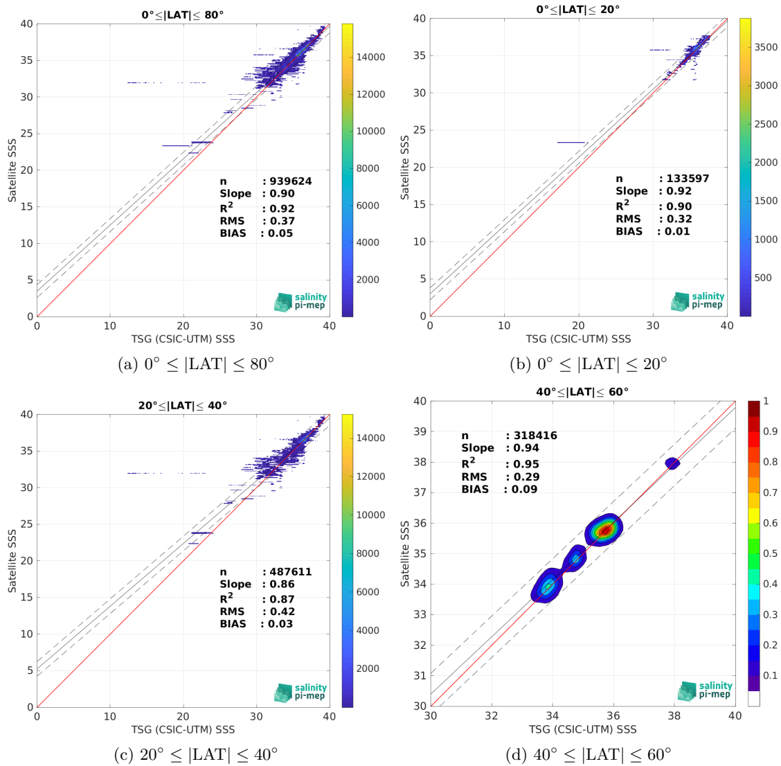
Figure 9: Contour maps of the concentration of CCI SSS L4 Merged-OI v4.4 - 7-day running (ESA) SSS (y-axis) versus TSG (CSIC-UTM) SSS (x-axis) at match-up pairs for different latitude bands. For each plot, the red line shows x=y . The black thin and dashed lines indicate a linear fit through the data cloud and the \pm 95\% confidence levels, respectively. The number match-up pairs n , the slope and R^2 coefficient of the linear fit, the root mean square (RMS) and the mean bias between satellite and in situ data are indicated for each latitude band in each plots.
