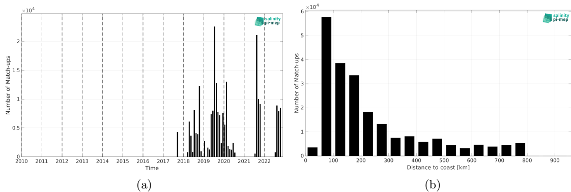
Figure 1: Number of match-ups between Saildrone and CCI SSS L4 Merged-OI v4.4 - 7-day running (ESA) SSS as a function of time (a) and as function of the distance to coast (b) over the SMOS coastal zone (<800km) 60N-60S Pi-MEP region and for the full satellite product period.
