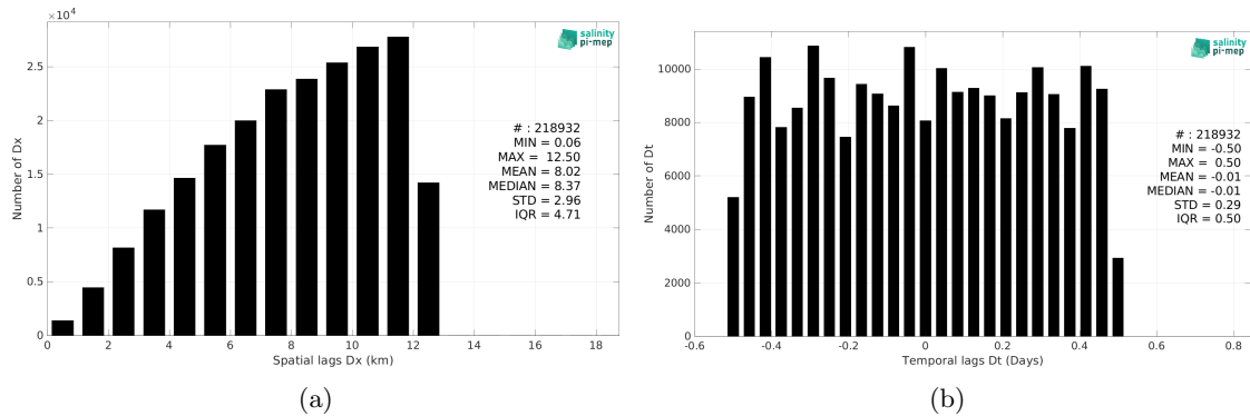
Figure 5: Histograms of the spatial (a) and temporal (b) lags between the location/time of the Saildrone measurement and the date of the corresponding CCI SSS L4 Merged-OI v4.4 - 7-day running (ESA) SSS pixel.
