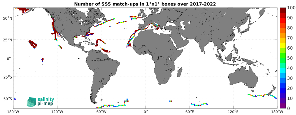
Figure 4: Number of SSS match-ups between Saildrone SSS and the CCI SSS L4 Merged-OI v4.4 - 7-day running (ESA) SSS product for the SMOS coastal zone ( <800\text{km} ) 60N-60S Pi-MEP region over 1^\circ \times 1^\circ boxes and for the full satellite product period.
