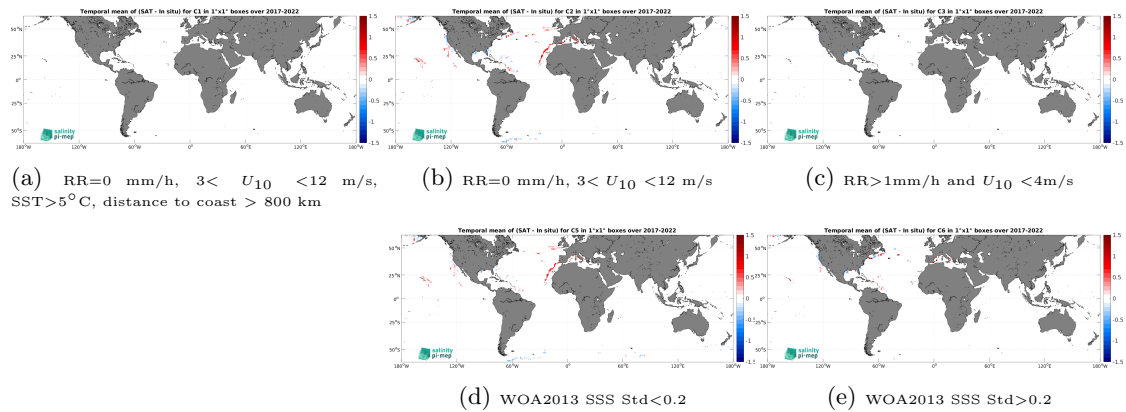
Figure 12: Temporal mean gridded over spatial boxes of size 1^\circ \times 1^\circ of \Delta SSS (CCI SSS L4 Merged-OI v4.4 - 7-day running (ESA) - Saildrone) for 5 different subdatasets corresponding to:RR=0 mm/h, 3 < U_{10} < 12 m/s, SST >5^\circ C, distance to coast > 800 km (a), RR=0 mm/h, 3 < U_{10} < 12 m/s (b), RR >1 mm/h and U_{10} < 4 m/s (c), WOA2013 SSS Std <0.2 (d), WOA2013 SSS Std >0.2 (e).
