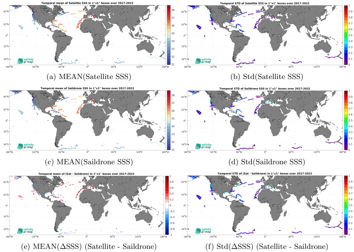
Figure 6: Temporal mean (left) and Std (right) of SSS from CCI SSS L4 Merged-OI v4.4 - 7-day running (ESA) (top), Saildrone (middle), and of \Delta SSS (Satellite - Saildrone). Only match-up pairs are used to generate these maps.
