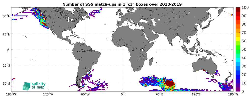
Figure 4: Number of SSS match-ups between Marine mammals SSS and the CCI SSS L4 Merged-OI v4.4 - 7-day running (ESA) SSS product for the SMOS coastal zone (<800km) 60N-60S Pi-MEP region over 1^\circ \times 1^\circ boxes and for the full satellite product period.
