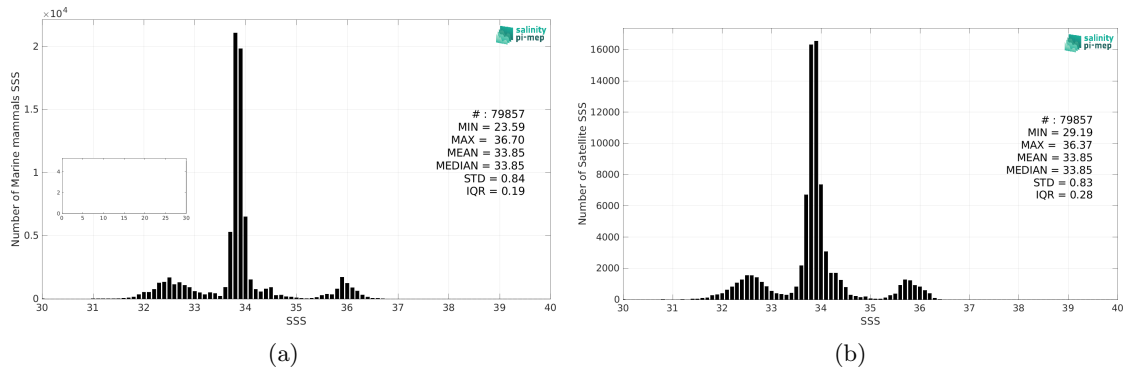
Figure 2: Histograms of SSS from Marine mammals (a) and CCI SSS L4 Merged-OI v4.4 - 7-day running (ESA) (b) considering all match-up pairs per bins of 0.1 over the SMOS coastal zone (<800km) 60N-60S Pi-MEP region and for the full satellite product period.
