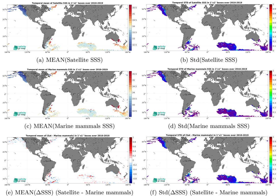
Figure 6: Temporal mean (left) and Std (right) of SSS from CCI SSS L4 Merged-OI v4.4 - 7-day running (ESA) (top), Marine mammals (middle), and of \Delta SSS (Satellite - Marine mammals). Only match-up pairs are used to generate these maps.
