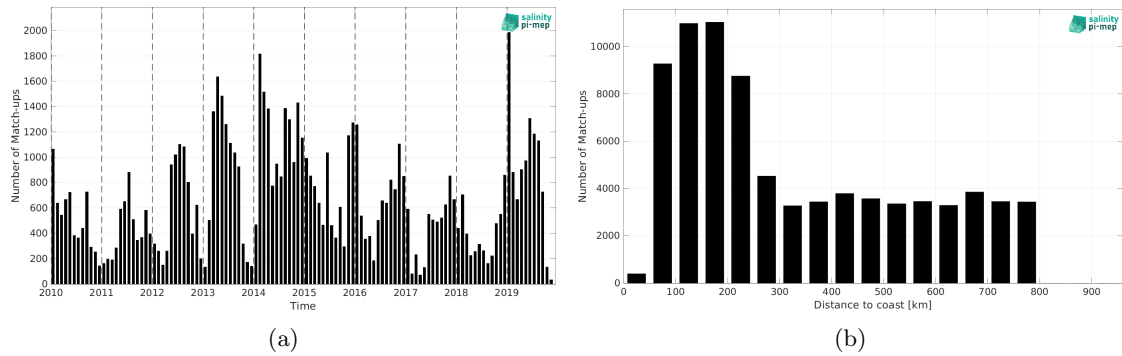
Figure 1: Number of match-ups between Marine mammals and CCI SSS L4 Merged-OI v4.4 - 7-day running (ESA) SSS as a function of time (a) and as function of the distance to coast (b) over the SMOS coastal zone (<800km) 60N-60S Pi-MEP region and for the full satellite product period.
