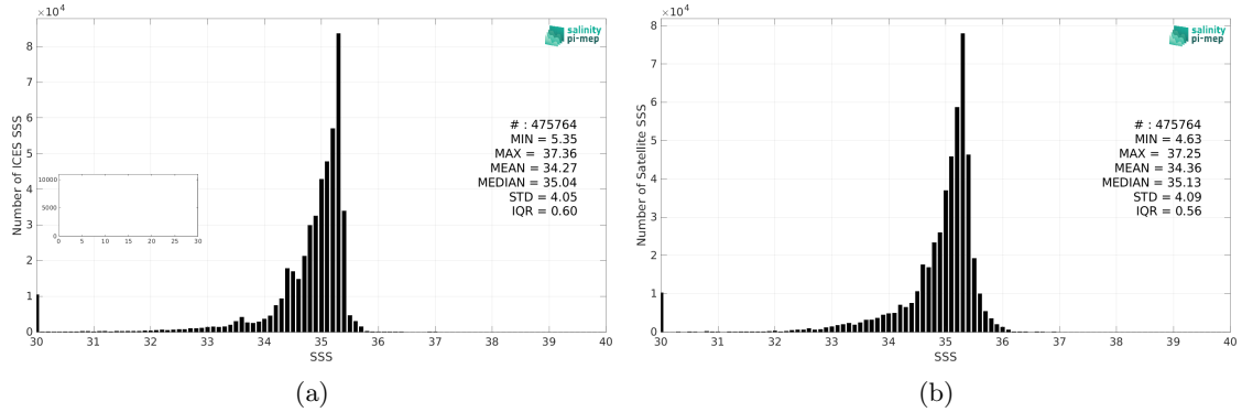
Figure 2: Histograms of SSS from ICES (a) and CCI SSS L4 Merged-OI v4.4 - 7-day running (ESA) (b) considering all match-up pairs per bins of 0.1 over the SMOS coastal zone (<800km) 60N-60S Pi-MEP region and for the full satellite product period.
