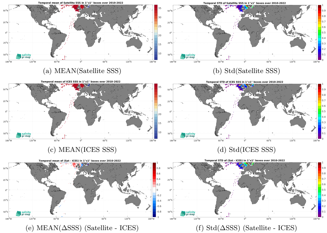
Figure 6: Temporal mean (left) and Std (right) of SSS from CCI SSS L4 Merged-OI v4.4 - 7-day running (ESA) (top), ICES (middle), and of \Delta SSS (Satellite - ICES). Only match-up pairs are used to generate these maps.
