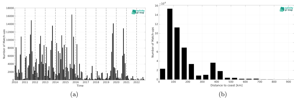
Figure 1: Number of match-ups between ICES and CCI SSS L4 Merged-OI v4.4 - 7-day running (ESA) SSS as a function of time (a) and as function of the distance to coast (b) over the SMOS coastal zone (<800km) 60N-60S Pi-MEP region and for the full satellite product period.
