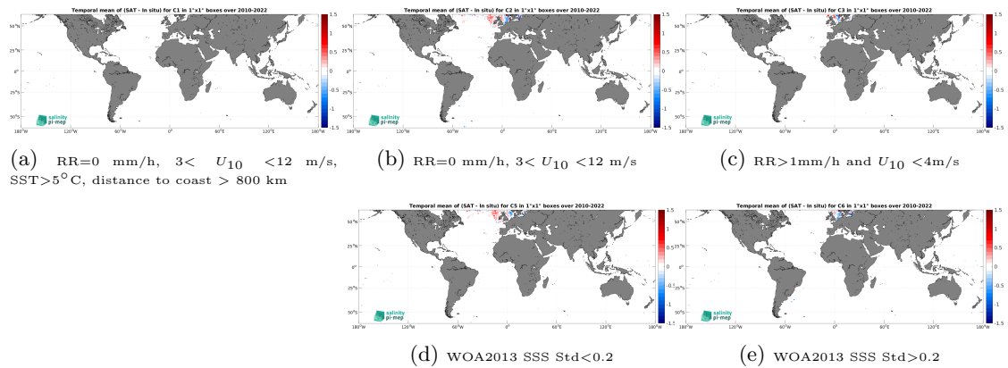
Figure 12: Temporal mean gridded over spatial boxes of size 1^\circ \times 1^\circ of \Delta\text{SSS} (CCI SSS L4 Merged-OI v4.4 - 7-day running (ESA) - ICES) for 5 different subdatasets corresponding to:RR=0 mm/h, 3 < U_{10} < 12 m/s, SST >5^\circ\text{C} , distance to coast > 800 km (a), RR=0 mm/h, 3 < U_{10} < 12 m/s (b), RR >1 mm/h and U_{10} < 4 m/s (c), WOA2013 SSS Std <0.2 (d), WOA2013 SSS Std >0.2 (e).
