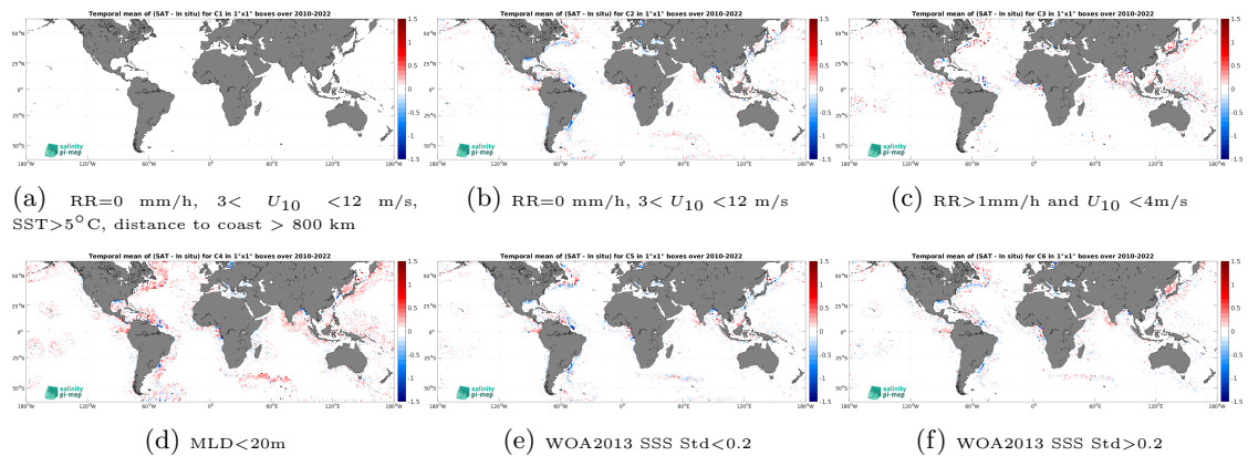
Figure 12: Temporal mean gridded over spatial boxes of size 1^\circ \times 1^\circ of \Delta SSS (CCI SSS L4 Merged-OI v4.4 - 7-day running (ESA) - Argo) for 6 different subdatasets corresponding to:RR=0 mm/h, 3 < U_{10} < 12 m/s, SST >5^\circ C, distance to coast > 800 km (a), RR=0 mm/h, 3 < U_{10} < 12 m/s (b), RR >1 mm/h and U_{10} < 4 m/s (c),MLD <20 m (d),WOA2013 SSS Std <0.2 (e),WOA2013 SSS Std >0.2 (f).
