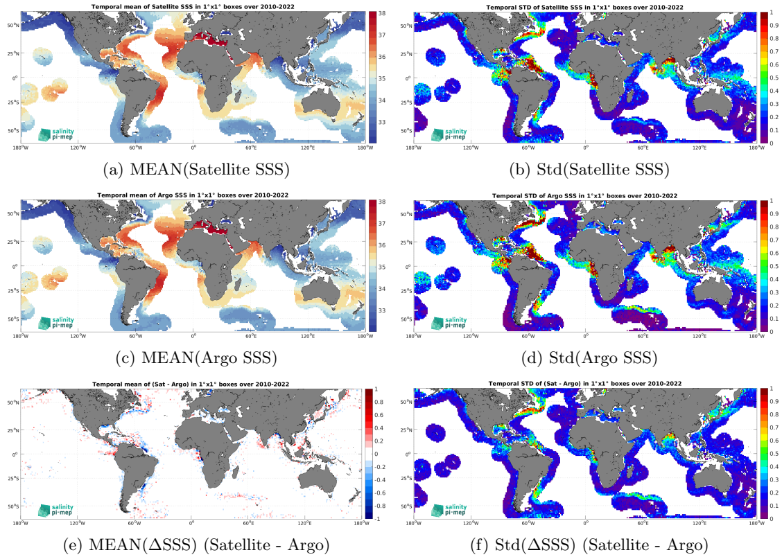
Figure 6: Temporal mean (left) and Std (right) of SSS from CCI SSS L4 Merged-OI v4.4 - 7-day running (ESA) (top), Argo (middle), and of \Delta SSS (Satellite - Argo). Only match-up pairs are used to generate these maps.
