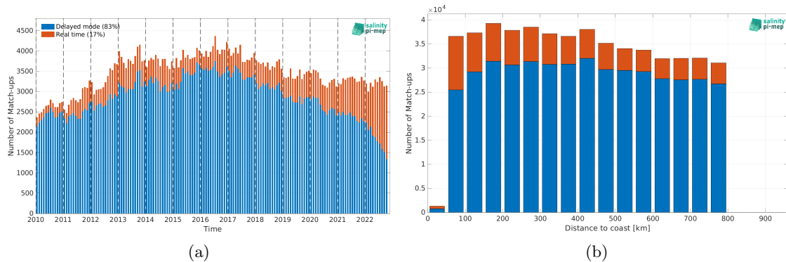
Figure 1: Number of match-ups between Argo and CCI SSS L4 Merged-OI v4.4 - 7-day running (ESA) SSS as a function of time (a) and as function of the distance to coast (b) over the SMOS coastal zone ( < 800\text{km} ) 60N-60S Pi-MEP region and for the full satellite product period.
