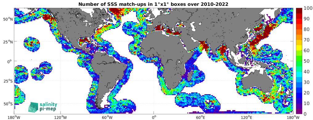
Figure 4: Number of SSS match-ups between Argo SSS and the CCI SSS L4 Merged-OI v4.4 - 7-day running (ESA) SSS product for the SMOS coastal zone (<800km) 60N-60S Pi-MEP region over 1^\circ \times 1^\circ boxes and for the full satellite product period.
