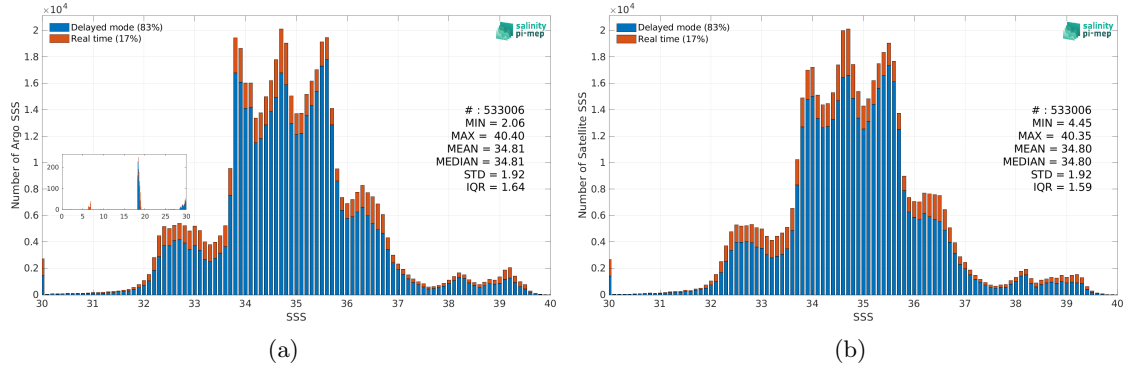
Figure 2: Histograms of SSS from Argo (a) and CCI SSS L4 Merged-OI v4.4 - 7-day running (ESA) (b) considering all match-up pairs per bins of 0.1 over the SMOS coastal zone (<800km) 60N-60S Pi-MEP region and for the full satellite product period.
