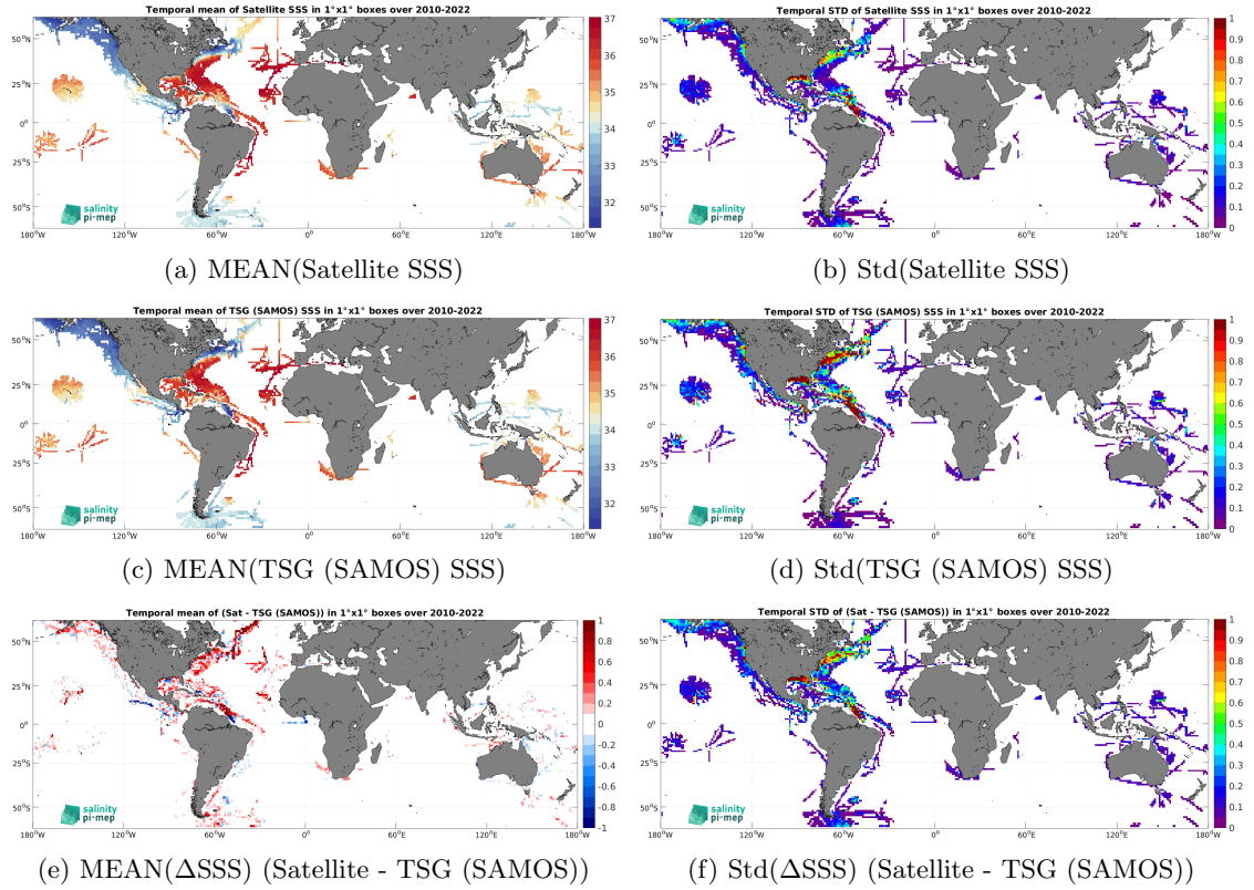
Figure 6: Temporal mean (left) and Std (right) of SSS from CCI SSS L4 Merged-OI v4.4 - 30-day running (ESA) (top), TSG (SAMOS) (middle), and of \Delta SSS (Satellite - TSG (SAMOS)). Only match-up pairs are used to generate these maps.
