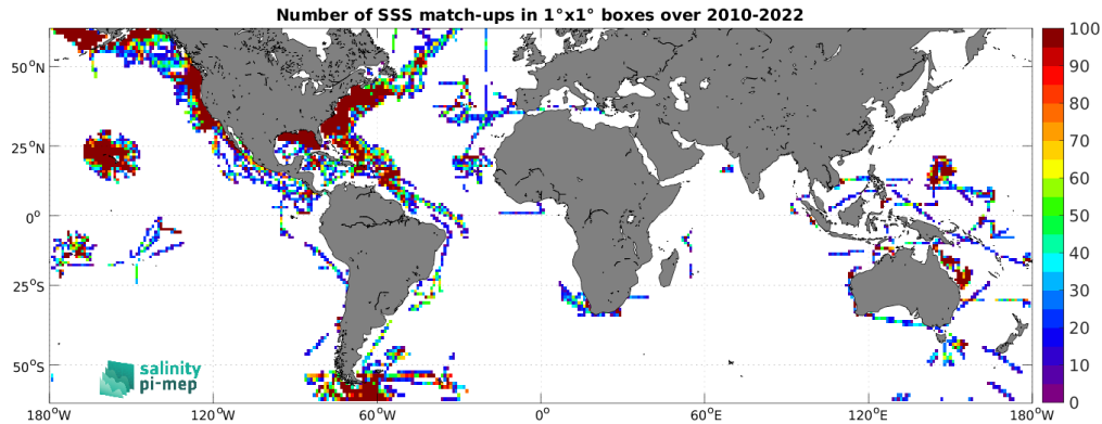
Figure 4: Number of SSS match-ups between TSG (SAMOS) SSS and the CCI SSS L4 Merged-OI v4.4 - 30-day running (ESA) SSS product for the SMOS coastal zone (<800km) 60N-60S Pi-MEP region over 1^{\circ} \times 1^{\circ} boxes and for the full satellite product period.
