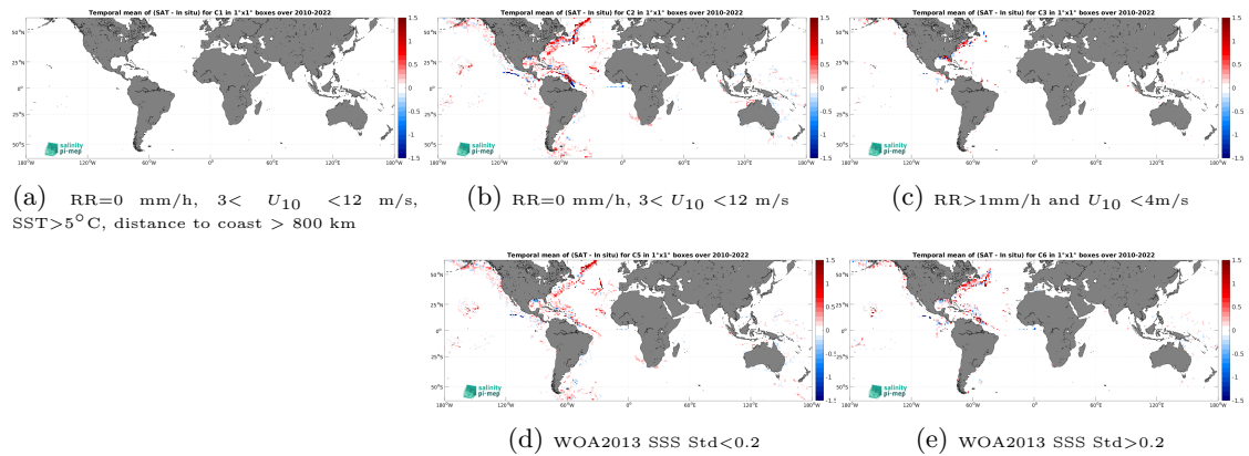
Figure 12: Temporal mean gridded over spatial boxes of size 1^\circ \times 1^\circ of \Delta\text{SSS} (CCI SSS L4 Merged-OI v4.4 - 30-day running (ESA) - TSG (SAMOS)) for 5 different subdatasets corresponding to:RR=0 mm/h, 3 < U_{10} < 12 m/s, SST >5^\circ\text{C} , distance to coast > 800 km (a), RR=0 mm/h, 3 < U_{10} < 12 m/s (b), RR >1 mm/h and U_{10} < 4 m/s (c), WOA2013 SSS Std <0.2 (d), WOA2013 SSS Std >0.2 (e).
