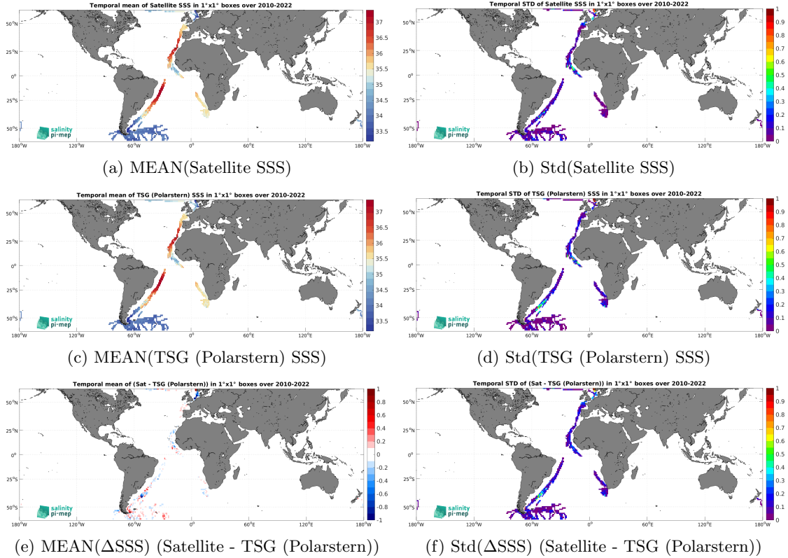
Figure 6: Temporal mean (left) and Std (right) of SSS from CCI SSS L4 Merged-OI v4.4 - 30-day running (ESA) (top), TSG (Polarstern) (middle), and of \Delta SSS (Satellite - TSG (Polarstern)). Only match-up pairs are used to generate these maps.
