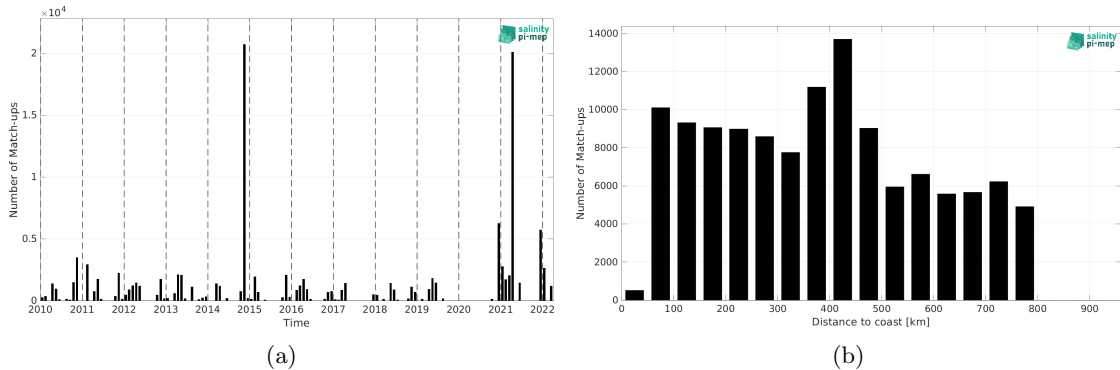
Figure 1: Number of match-ups between TSG (Polarstern) and CCI SSS L4 Merged-OI v4.4 - 30-day running (ESA) SSS as a function of time (a) and as function of the distance to coast (b) over the SMOS coastal zone (<800km) 60N-60S Pi-MEP region and for the full satellite product period.
