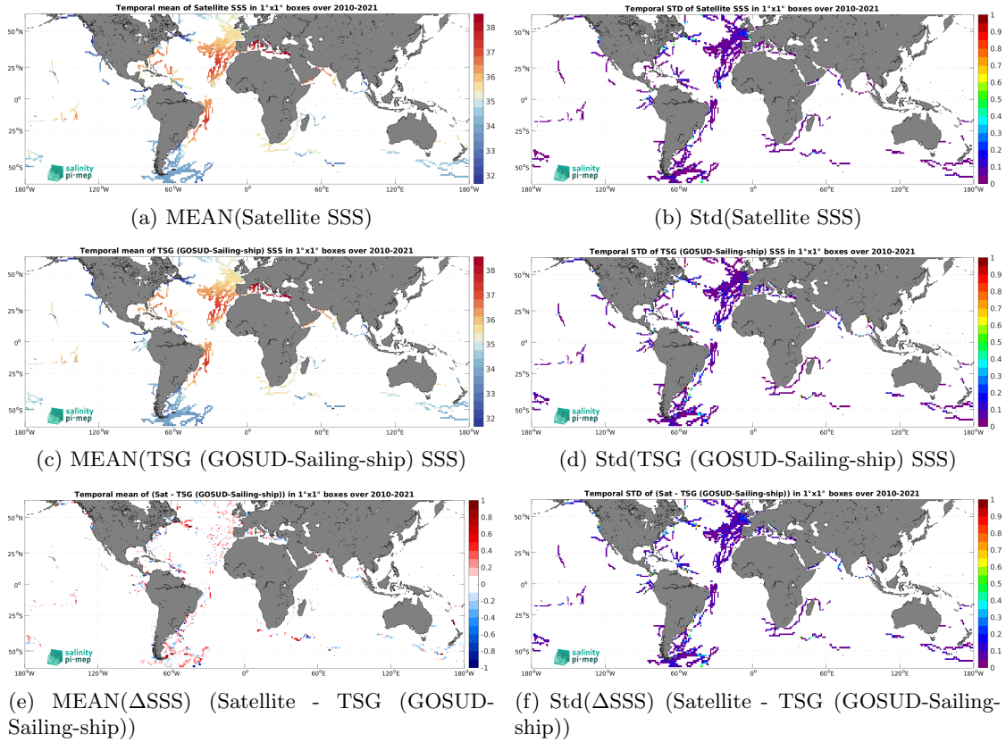
Figure 6: Temporal mean (left) and Std (right) of SSS from CCI SSS L4 Merged-OI v4.4 - 30-day running (ESA) (top), TSG (GOSUD-Sailing-ship) (middle), and of \Delta SSS (Satellite - TSG (GOSUD-Sailing-ship)). Only match-up pairs are used to generate these maps.
