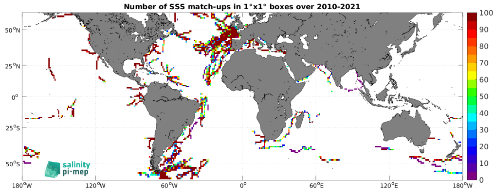
Figure 4: Number of SSS match-ups between TSG (GOSUD-Sailing-ship) SSS and the CCI SSS L4 Merged-OI v4.4 - 30-day running (ESA) SSS product for the SMOS coastal zone (<800km) 60N-60S Pi-MEP region over 1^\circ \times 1^\circ boxes and for the full satellite product period.
