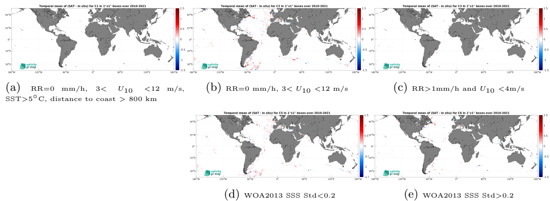
Figure 12: Temporal mean gridded over spatial boxes of size 1^\circ \times 1^\circ of \Delta\text{SSS} (CCI SSS L4 Merged-OI v4.4 - 30-day running (ESA) - TSG (GOSUD-Sailing-ship)) for 5 different subdatasets corresponding to: RR=0 mm/h, 3 < U_{10} < 12 m/s, SST > 5°C, distance to coast > 800 km (a), RR=0 mm/h, 3 < U_{10} < 12 m/s (b), RR > 1mm/h and U_{10} < 4 m/s (c), WOA2013 SSS Std < 0.2 (d), WOA2013 SSS Std > 0.2 (e).
