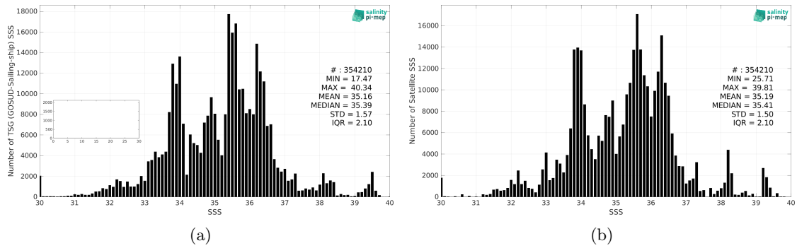
Figure 2: Histograms of SSS from TSG (GOSUD-Sailing-ship) (a) and CCI SSS L4 Merged-OI v4.4 - 30-day running (ESA) (b) considering all match-up pairs per bins of 0.1 over the SMOS coastal zone (<800km) 60N-60S Pi-MEP region and for the full satellite product period.
