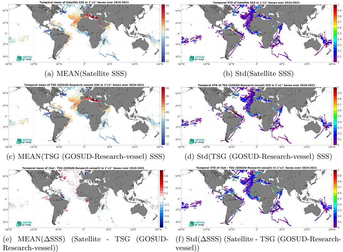
Figure 6: Temporal mean (left) and Std (right) of SSS from CCI SSS L4 Merged-OI v4.4 - 30-day running (ESA) (top), TSG (GOSUD-Research-vessel) (middle), and of \Delta\text{SSS} (Satellite - TSG (GOSUD-Research-vessel)). Only match-up pairs are used to generate these maps.
