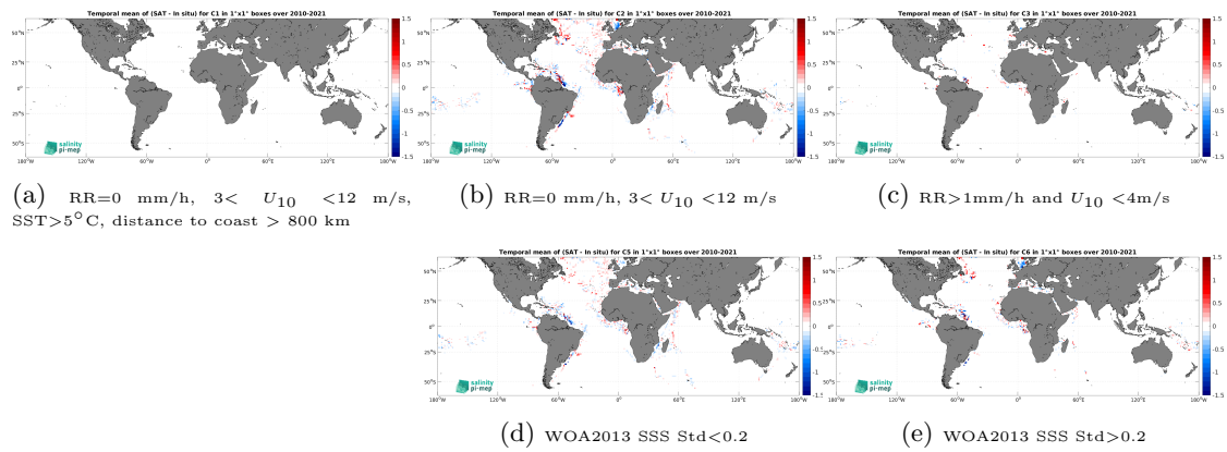
Figure 12: Temporal mean gridded over spatial boxes of size 1^\circ \times 1^\circ of \Delta SSS (CCI SSS L4 Merged-OI v4.4 - 30-day running (ESA) - TSG (GOSUD-Research-vessel)) for 5 different subdatasets corresponding to:RR=0 mm/h, 3 < U_{10} < 12 m/s, SST >5^\circ\text{C} , distance to coast > 800 km (a), RR=0 mm/h, 3 < U_{10} < 12 m/s (b), RR >1 mm/h and U_{10} < 4 m/s (c), WOA2013 SSS Std <0.2 (d), WOA2013 SSS Std >0.2 (e).
