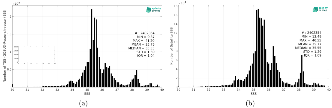
Figure 2: Histograms of SSS from TSG (GOSUD-Research-vessel) (a) and CCI SSS L4 Merged-OI v4.4 - 30-day running (ESA) (b) considering all match-up pairs per bins of 0.1 over the SMOS coastal zone (<800km) 60N-60S Pi-MEP region and for the full satellite product period.
