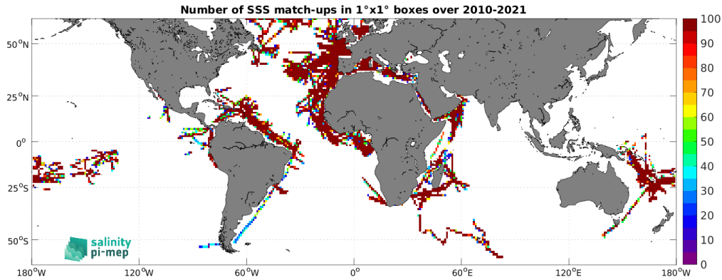
Figure 4: Number of SSS match-ups between TSG (GOSUD-Research-vessel) SSS and the CCI SSS L4 Merged-OI v4.4 - 30-day running (ESA) SSS product for the SMOS coastal zone (<800km) 60N-60S Pi-MEP region over 1^\circ \times 1^\circ boxes and for the full satellite product period.
