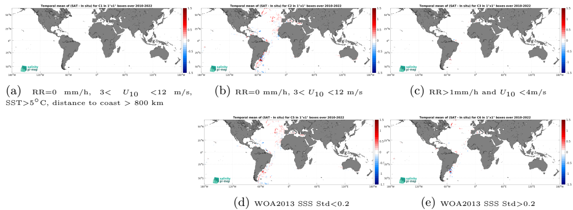
Figure 12: Temporal mean gridded over spatial boxes of size 1^\circ \times 1^\circ of \Delta\text{SSS} (CCI SSS L4 Merged-OI v4.4 - 30-day running (ESA) - TSG (CSIC-UTM)) for 5 different subdatasets corresponding to:RR=0 mm/h, 3 < U_{10} < 12 m/s, SST >5^\circ\text{C} , distance to coast > 800 km (a), RR=0 mm/h, 3 < U_{10} < 12 m/s (b), RR >1 mm/h and U_{10} < 4 m/s (c), WOA2013 SSS Std <0.2 (d), WOA2013 SSS Std >0.2 (e).
