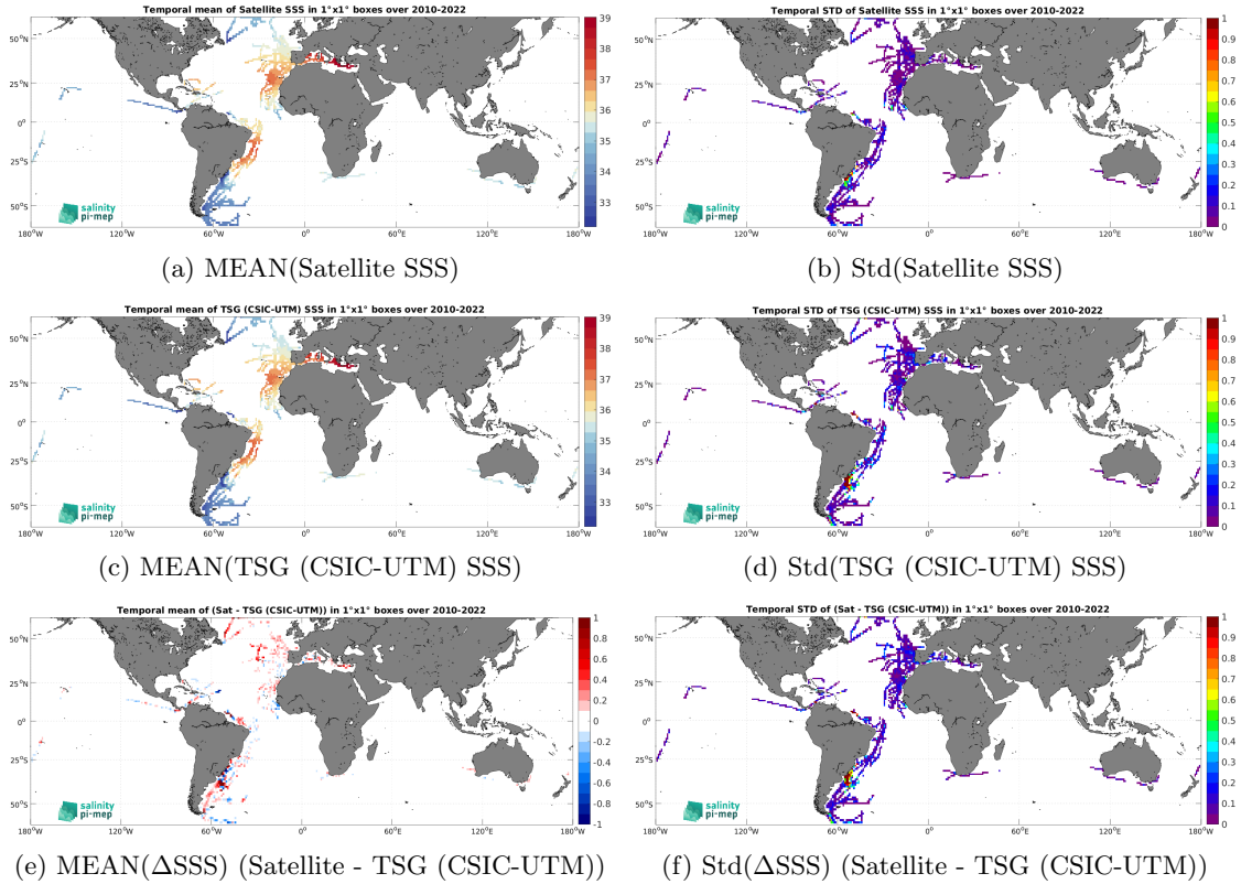
Figure 6: Temporal mean (left) and Std (right) of SSS from CCI SSS L4 Merged-OI v4.4 - 30-day running (ESA) (top), TSG (CSIC-UTM) (middle), and of \Delta SSS (Satellite - TSG (CSIC-UTM)). Only match-up pairs are used to generate these maps.
