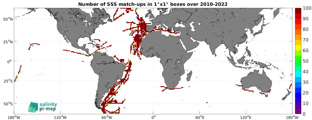
Figure 4: Number of SSS match-ups between TSG (CSIC-UTM) SSS and the CCI SSS L4 Merged-OI v4.4 - 30-day running (ESA) SSS product for the SMOS coastal zone (<800km) 60N-60S Pi-MEP region over 1^\circ \times 1^\circ boxes and for the full satellite product period.
