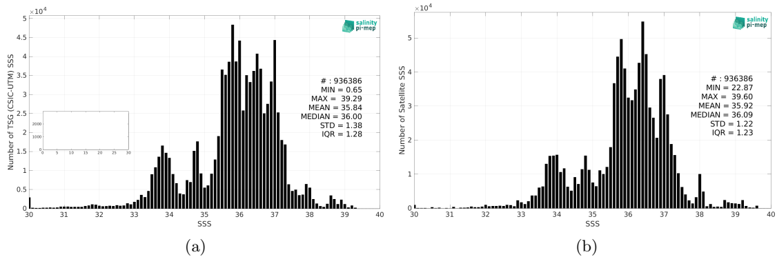
Figure 2: Histograms of SSS from TSG (CSIC-UTM) (a) and CCI SSS L4 Merged-OI v4.4 - 30-day running (ESA) (b) considering all match-up pairs per bins of 0.1 over the SMOS coastal zone (<800km) 60N-60S Pi-MEP region and for the full satellite product period.
