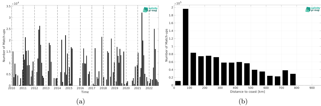
Figure 1: Number of match-ups between TSG (CSIC-UTM) and CCI SSS L4 Merged-OI v4.4 - 30-day running (ESA) SSS as a function of time (a) and as function of the distance to coast (b) over the SMOS coastal zone (<800km) 60N-60S Pi-MEP region and for the full satellite product period.
