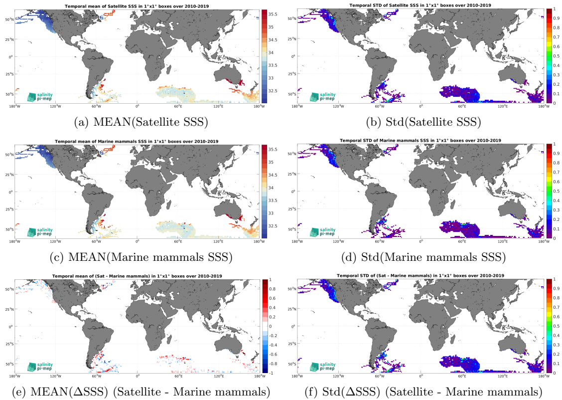
Figure 6: Temporal mean (left) and Std (right) of SSS from CCI SSS L4 Merged-OI v4.4 - 30-day running (ESA) (top), Marine mammals (middle), and of \Delta SSS (Satellite - Marine mammals). Only match-up pairs are used to generate these maps.
