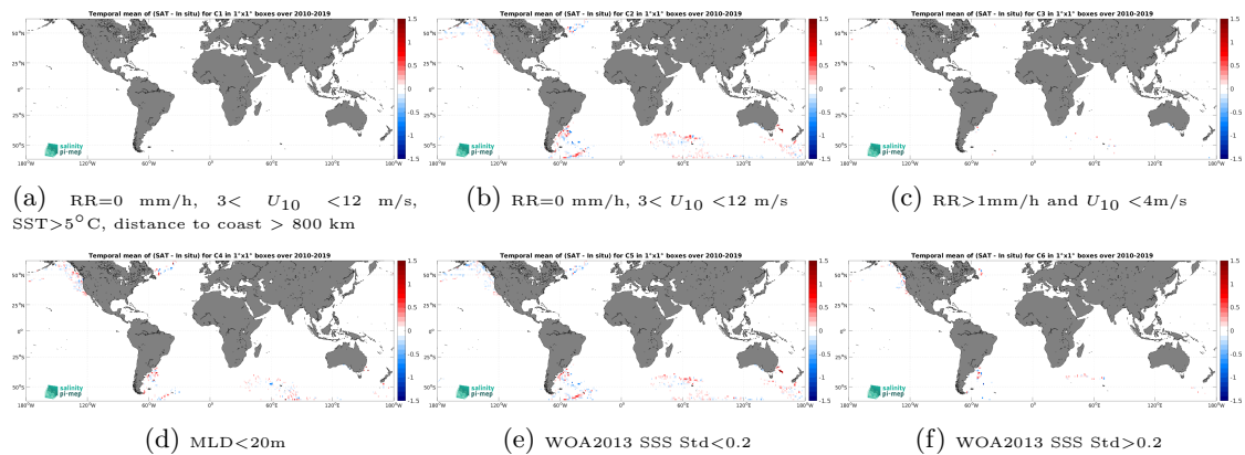
Figure 12: Temporal mean gridded over spatial boxes of size 1^\circ \times 1^\circ of \Delta SSS (CCI SSS L4 Merged-OI v4.4 - 30-day running (ESA) - Marine mammals) for 6 different subdatasets corresponding to:RR=0 mm/h, 3 < U_{10} < 12 m/s, SST >5^\circ C, distance to coast > 800 km (a), RR=0 mm/h, 3 < U_{10} < 12 m/s (b), RR >1 mm/h and U_{10} < 4 m/s (c),MLD <20 m (d),WOA2013 SSS Std <0.2 (e),WOA2013 SSS Std >0.2 (f).
