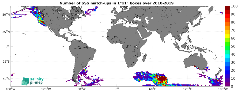
Figure 4: Number of SSS match-ups between Marine mammals SSS and the CCI SSS L4 Merged-OI v4.4 - 30-day running (ESA) SSS product for the SMOS coastal zone (<800km) 60N-60S Pi-MEP region over 1^\circ \times 1^\circ boxes and for the full satellite product period.
