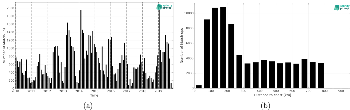
Figure 1: Number of match-ups between Marine mammals and CCI SSS L4 Merged-OI v4.4 - 30-day running (ESA) SSS as a function of time (a) and as function of the distance to coast (b) over the SMOS coastal zone (<800km) 60N-60S Pi-MEP region and for the full satellite product period.
