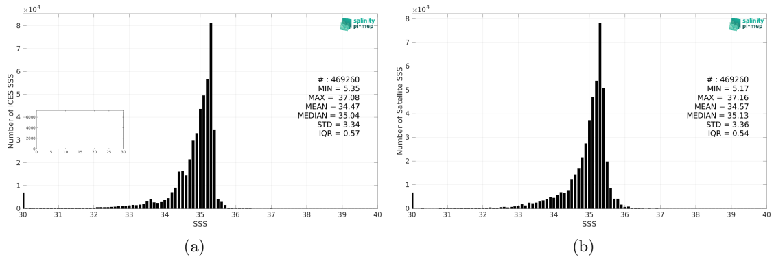
Figure 2: Histograms of SSS from ICES (a) and CCI SSS L4 Merged-OI v4.4 - 30-day running (ESA) (b) considering all match-up pairs per bins of 0.1 over the SMOS coastal zone (<800km) 60N-60S Pi-MEP region and for the full satellite product period.
