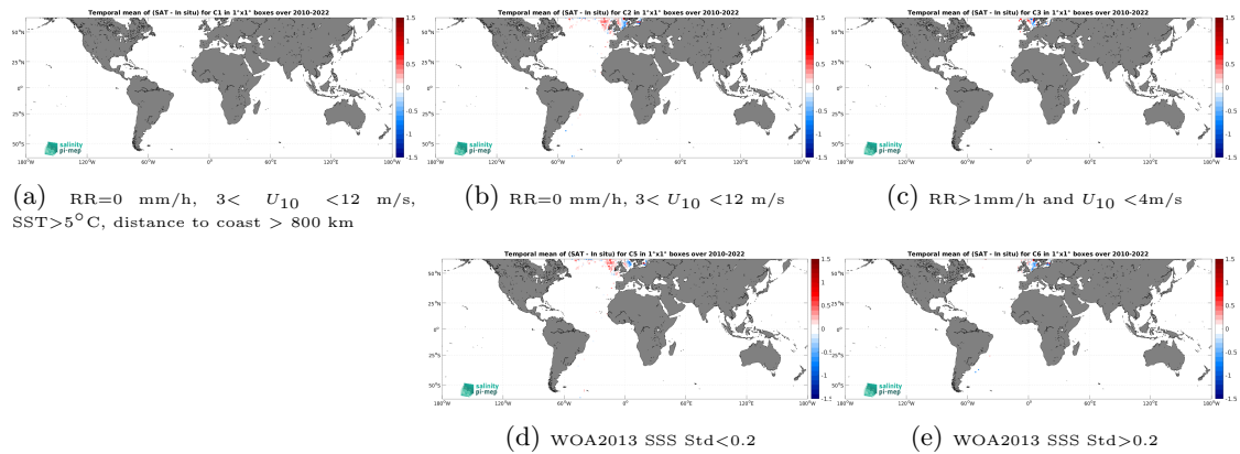
Figure 12: Temporal mean gridded over spatial boxes of size 1^\circ \times 1^\circ of \Delta SSS (CCI SSS L4 Merged-OI v4.4 - 30-day running (ESA) - ICES) for 5 different subdatasets corresponding to:RR=0 mm/h, 3 < U_{10} < 12 m/s, SST >5^\circ C, distance to coast > 800 km (a), RR=0 mm/h, 3 < U_{10} < 12 m/s (b), RR >1 mm/h and U_{10} < 4 m/s (c), WOA2013 SSS Std <0.2 (d), WOA2013 SSS Std >0.2 (e).
