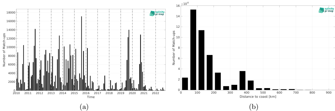
Figure 1: Number of match-ups between ICES and CCI SSS L4 Merged-OI v4.4 - 30-day running (ESA) SSS as a function of time (a) and as function of the distance to coast (b) over the SMOS coastal zone (<800km) 60N-60S Pi-MEP region and for the full satellite product period.
