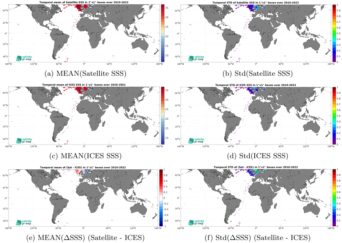
Figure 6: Temporal mean (left) and Std (right) of SSS from CCI SSS L4 Merged-OI v4.4 - 30-day running (ESA) (top), ICES (middle), and of \Delta SSS (Satellite - ICES). Only match-up pairs are used to generate these maps.
