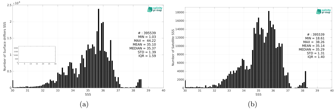
Figure 2: Histograms of SSS from Surface drifters (a) and CCI SSS L4 Merged-OI v4.4 - 30-day running (ESA) (b) considering all match-up pairs per bins of 0.1 over the SMOS coastal zone (<800km) 60N-60S Pi-MEP region and for the full satellite product period.
