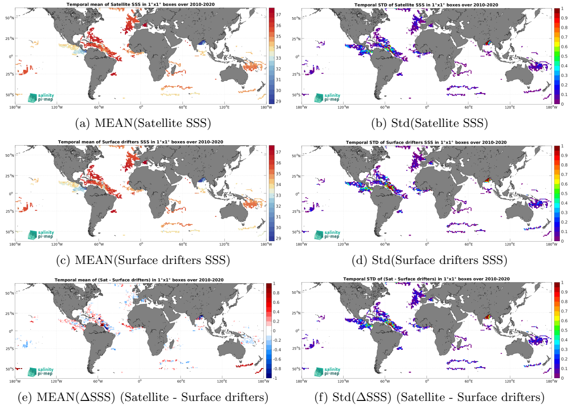
Figure 5: Temporal mean (left) and Std (right) of SSS from CCI SSS L4 Merged-OI v4.4 - 30-day running (ESA) (top), Surface drifters (middle), and of \Delta SSS (Satellite - Surface drifters). Only match-up pairs are used to generate these maps.
