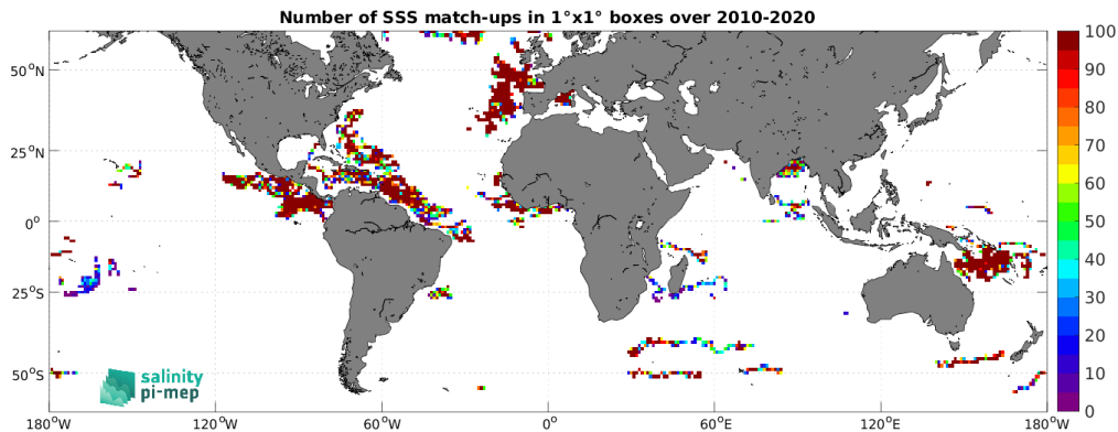
Figure 3: Number of SSS match-ups between Surface drifters SSS and the CCI SSS L4 Merged-OI v4.4 - 30-day running (ESA) SSS product for the SMOS coastal zone (<800km) 60N-60S Pi-MEP region over 1^\circ \times 1^\circ boxes and for the full satellite product period.
