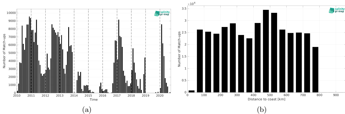
Figure 1: Number of match-ups between Surface drifters and CCI SSS L4 Merged-OI v4.4 - 30-day running (ESA) SSS as a function of time (a) and as function of the distance to coast (b) over the SMOS coastal zone (<800km) 60N-60S Pi-MEP region and for the full satellite product period.
