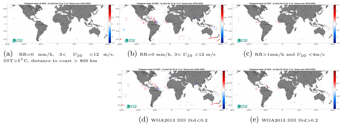
Figure 11: Temporal mean gridded over spatial boxes of size 1^\circ \times 1^\circ of \Delta\text{SSS} (CCI SSS L4 Merged-OI v4.4 - 30-day running (ESA) - Surface drifters) for 5 different subdatasets corresponding to:RR=0 mm/h, 3 < U_{10} < 12 m/s, SST >5^\circ\text{C} , distance to coast > 800 km (a), RR=0 mm/h, 3 < U_{10} < 12 m/s (b), RR >1 mm/h and U_{10} < 4 m/s (c), WOA2013 SSS Std <0.2 (d), WOA2013 SSS Std >0.2 (e).
