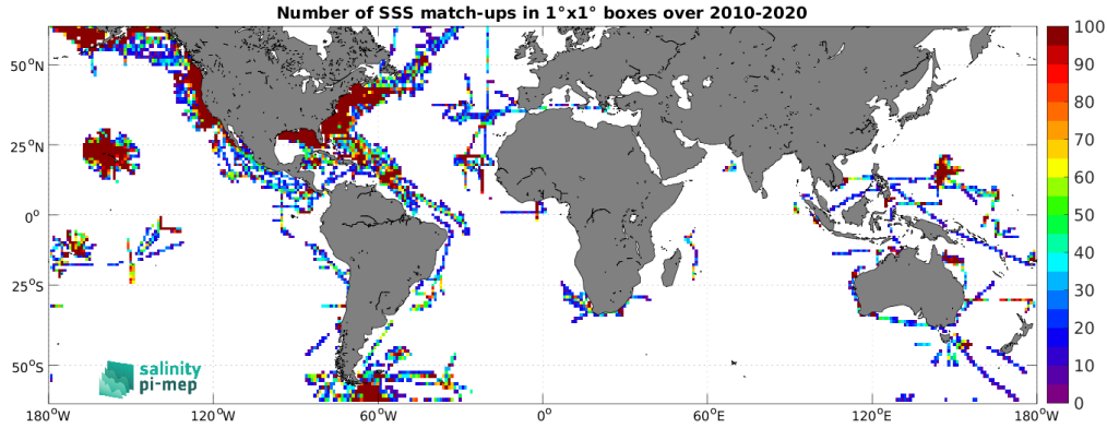
Figure 4: Number of SSS match-ups between TSG (SAMOS) SSS and the CCI SSS L4 Merged-OI v3.2 - 7-day running (ESA) SSS product for the SMOS coastal zone ( <800\text{km} ) 60N-60S Pi-MEP region over 1^\circ \times 1^\circ boxes and for the full satellite product period.
